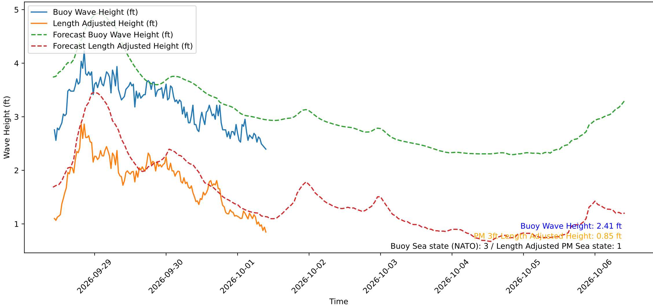
Wave Heights over Time for Oceanside Harbor at 2026-10-01 10:20:29
