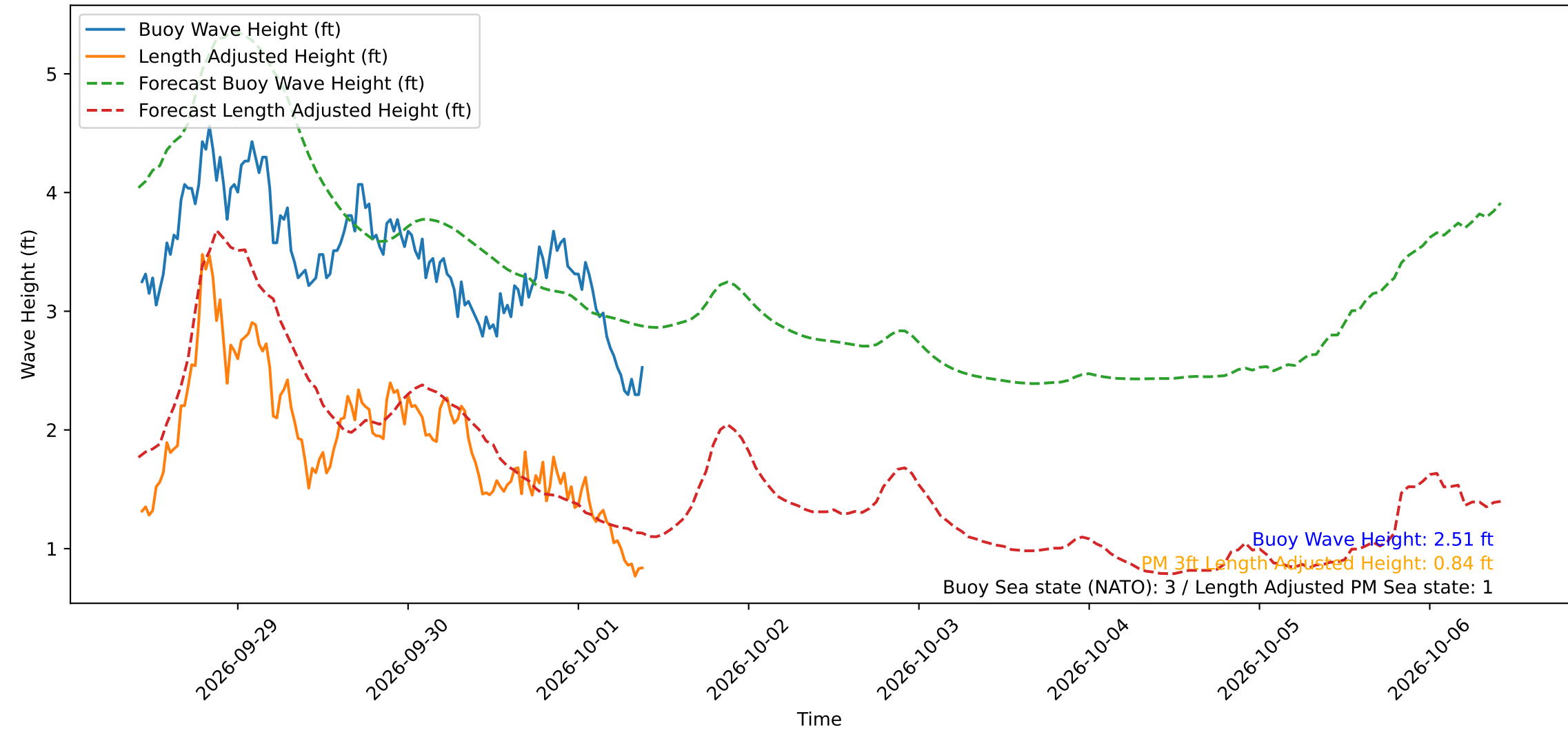
Wave Heights over Time for Green Beach at 2026-10-01 10:21:16
