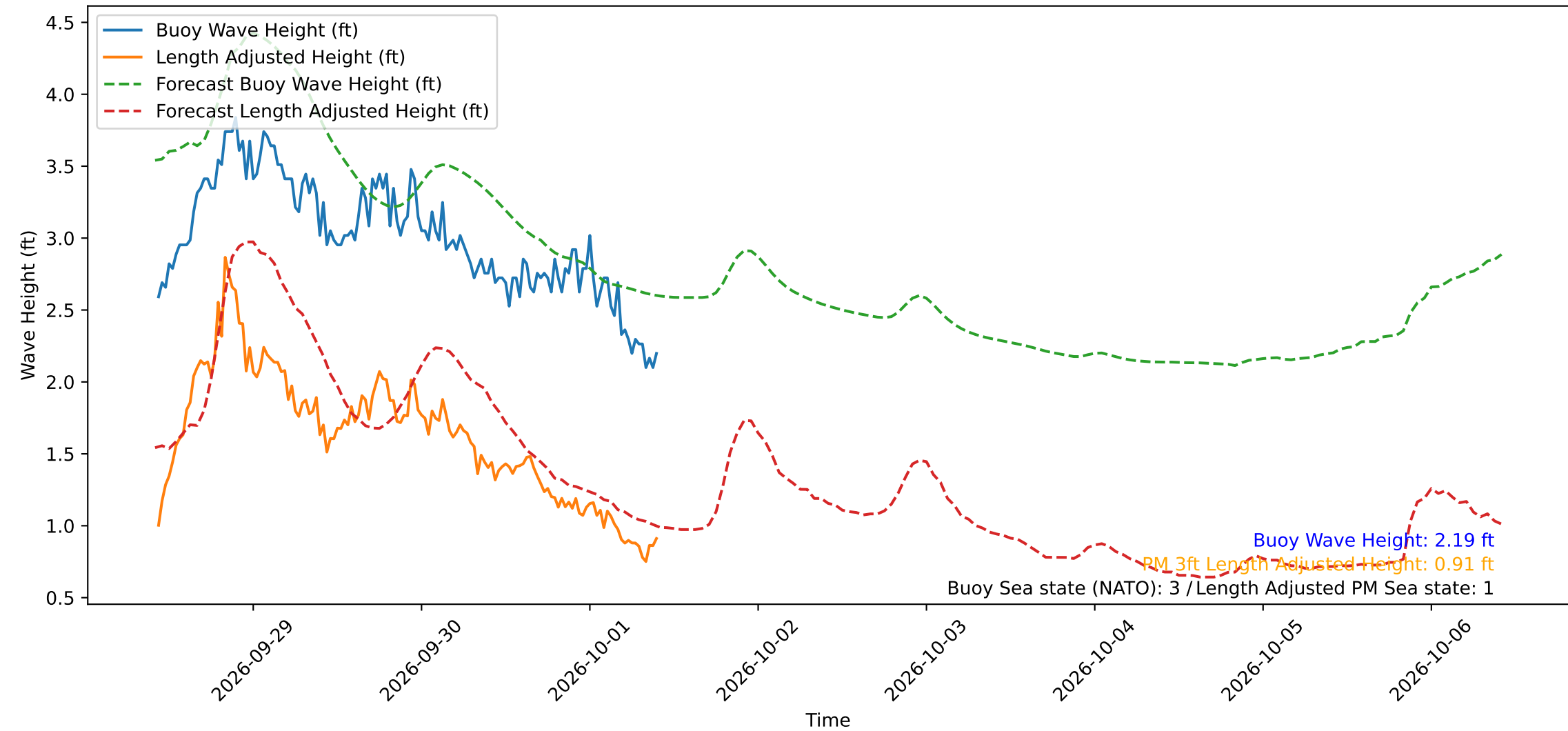
Wave Heights over Time for Red Beach at 2026-10-01 10:20:51
