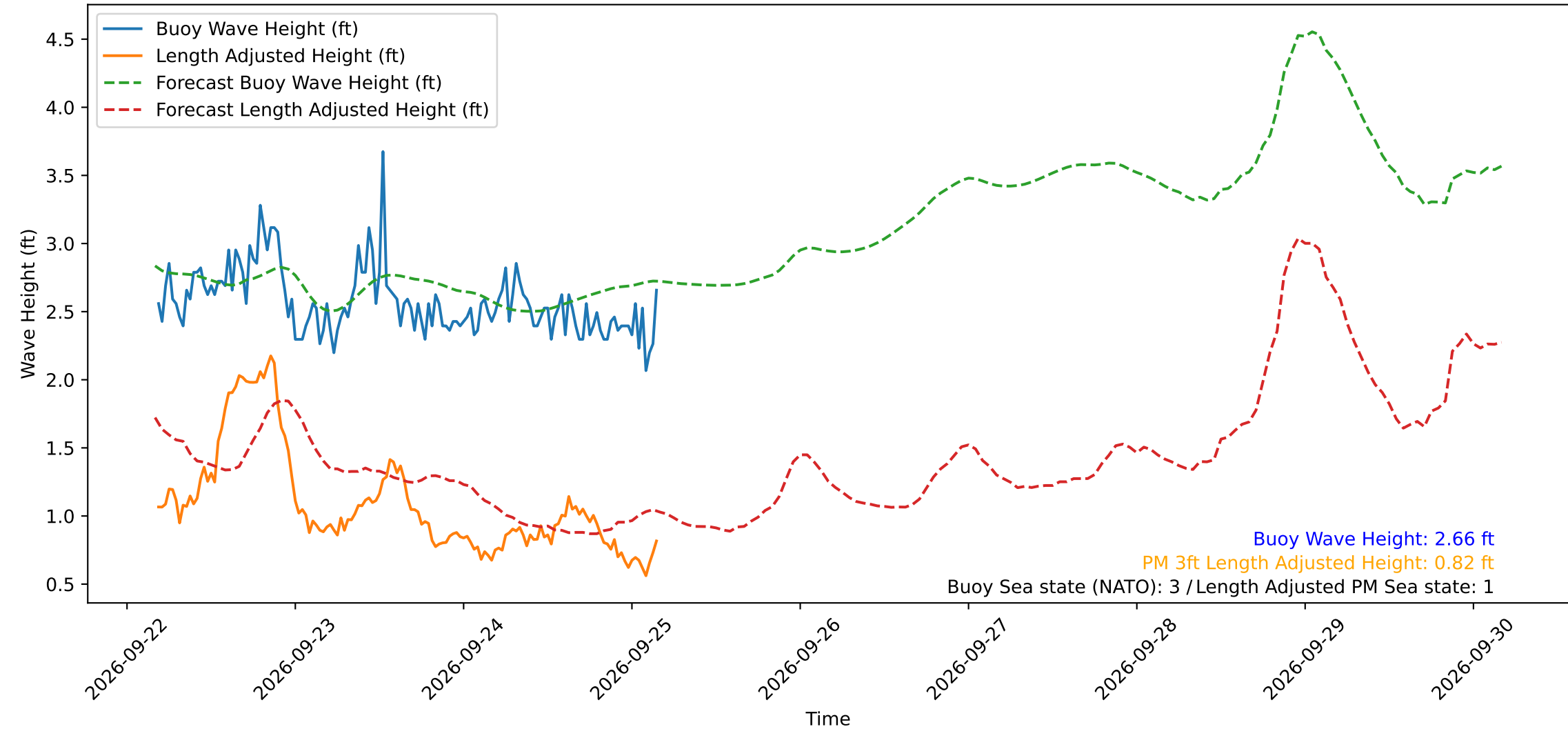
Wave Heights over Time for Red Beach at 2026-09-25 04:10:49
