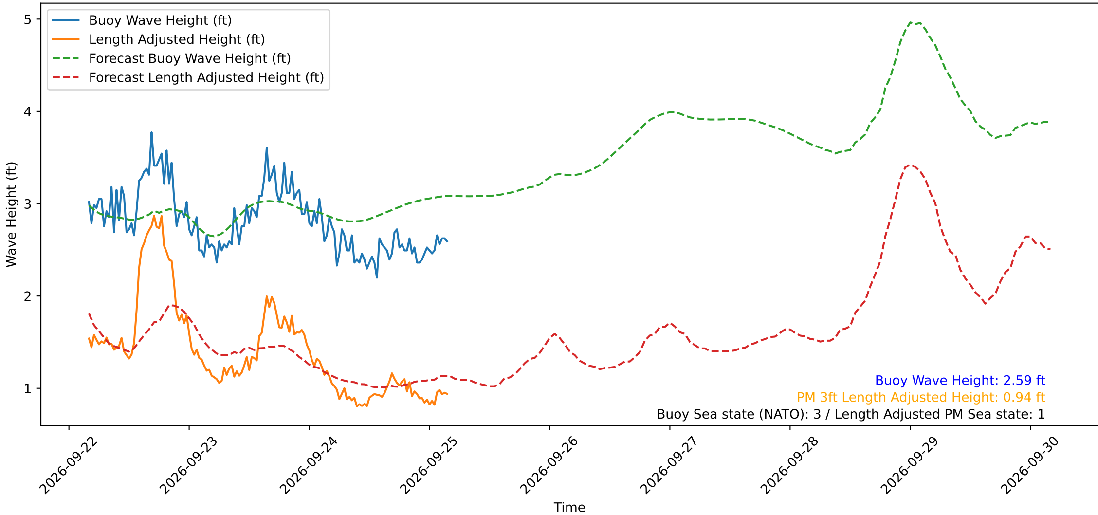
Wave Heights over Time for Oceanside Harbor at 2026-09-25 04:10:29
