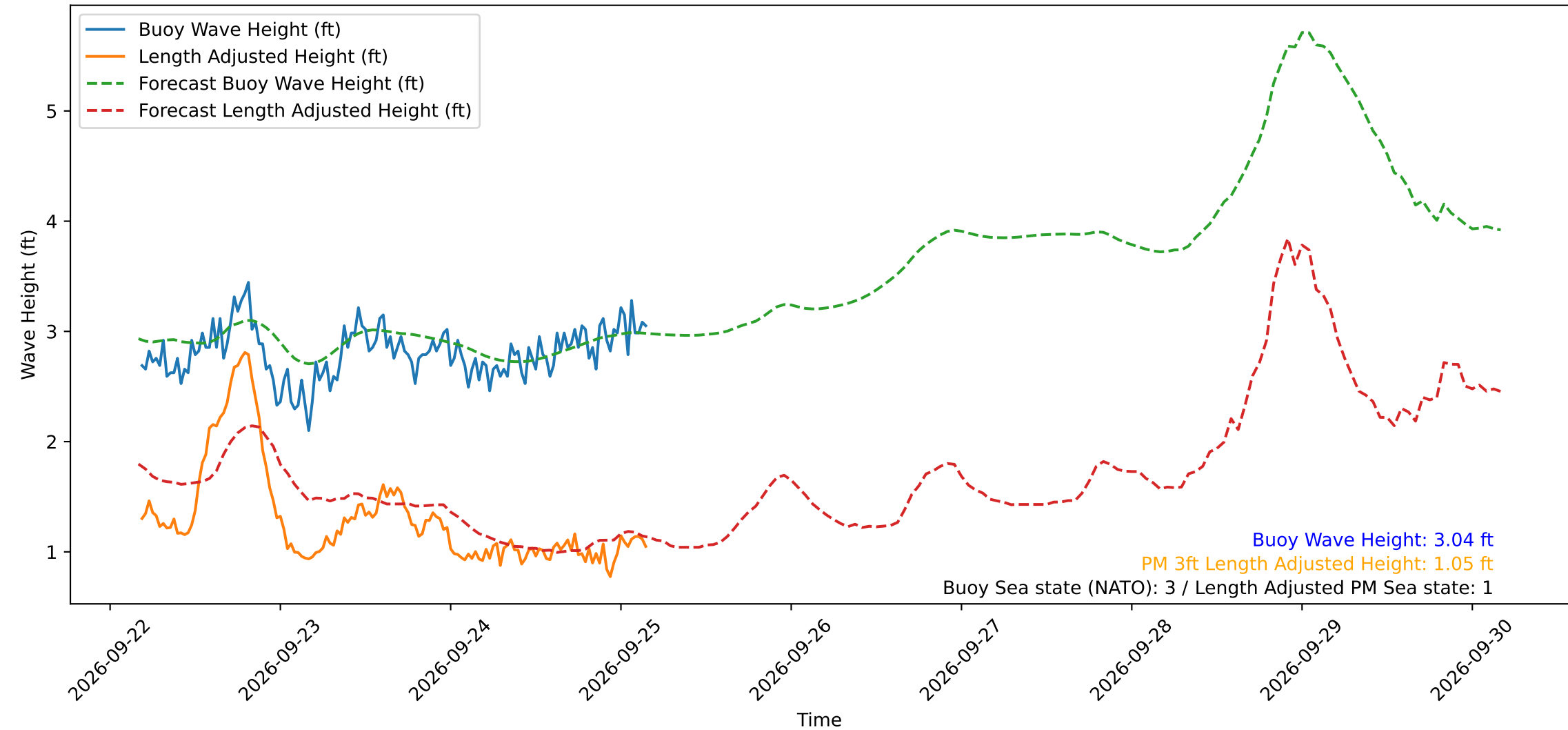
Wave Heights over Time for Green Beach at 2026-09-25 04:11:11
