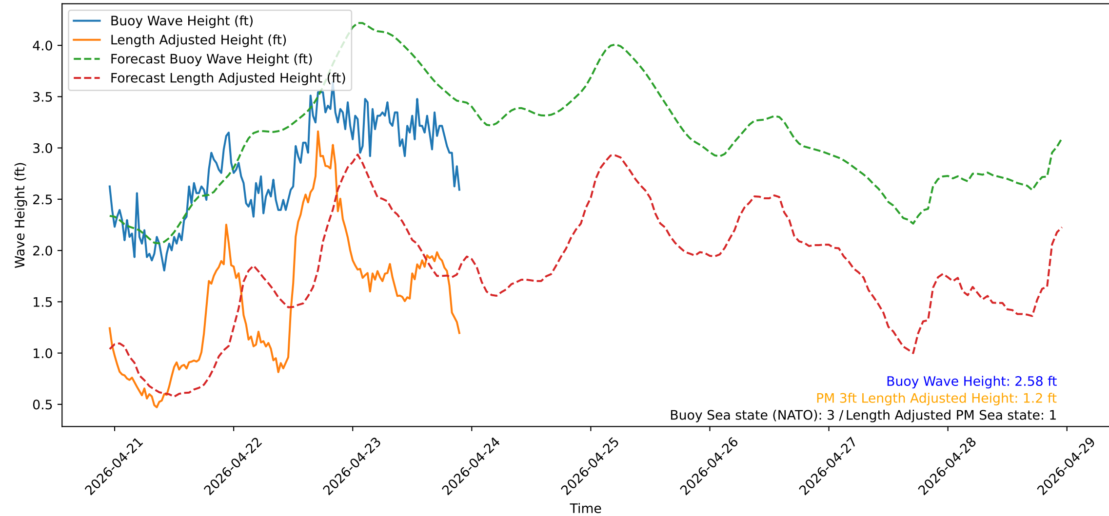
Wave Heights over Time for Red Beach at 2026-04-23 22:30:49
