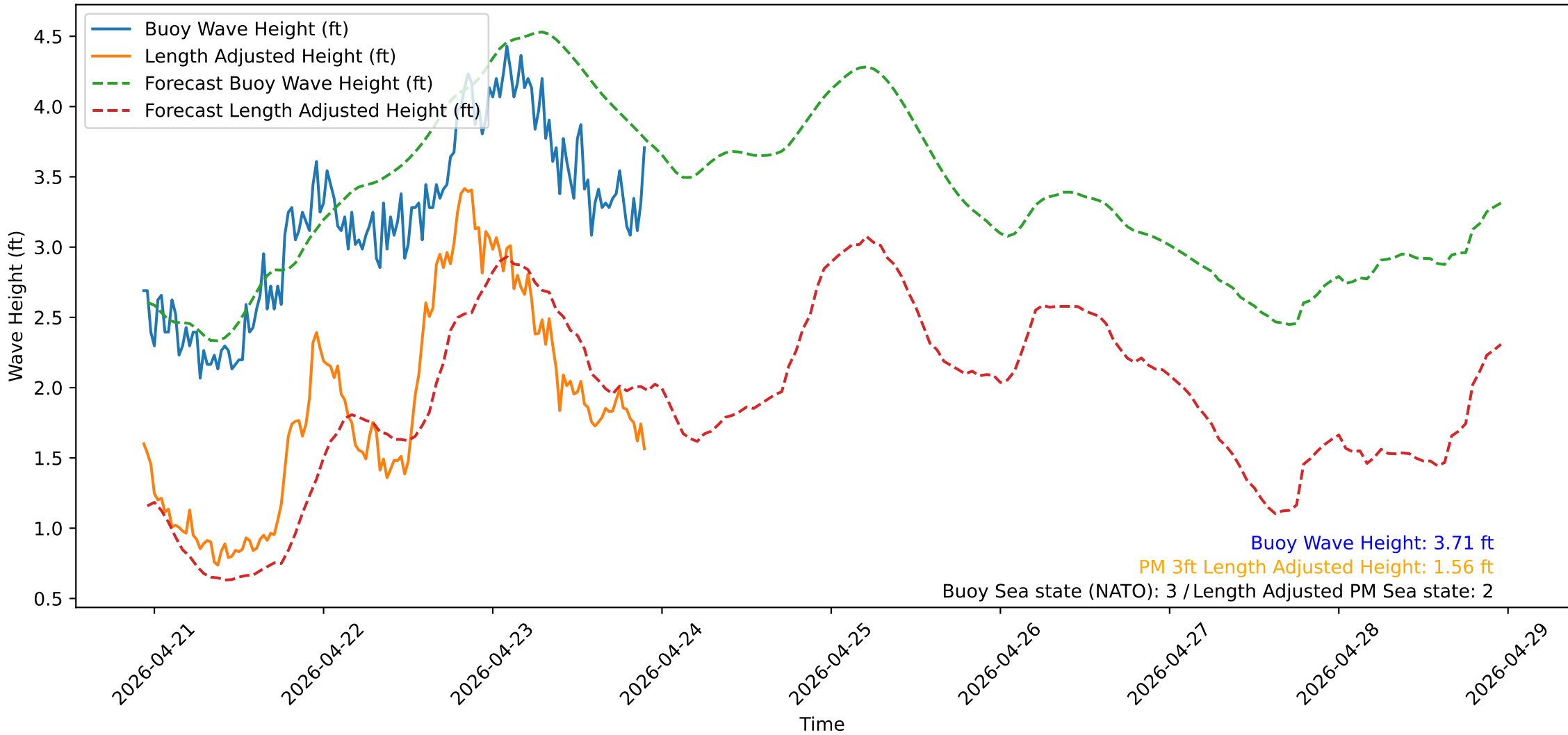
Wave Heights over Time for Oceanside Harbor at 2026-04-23 22:30:30
