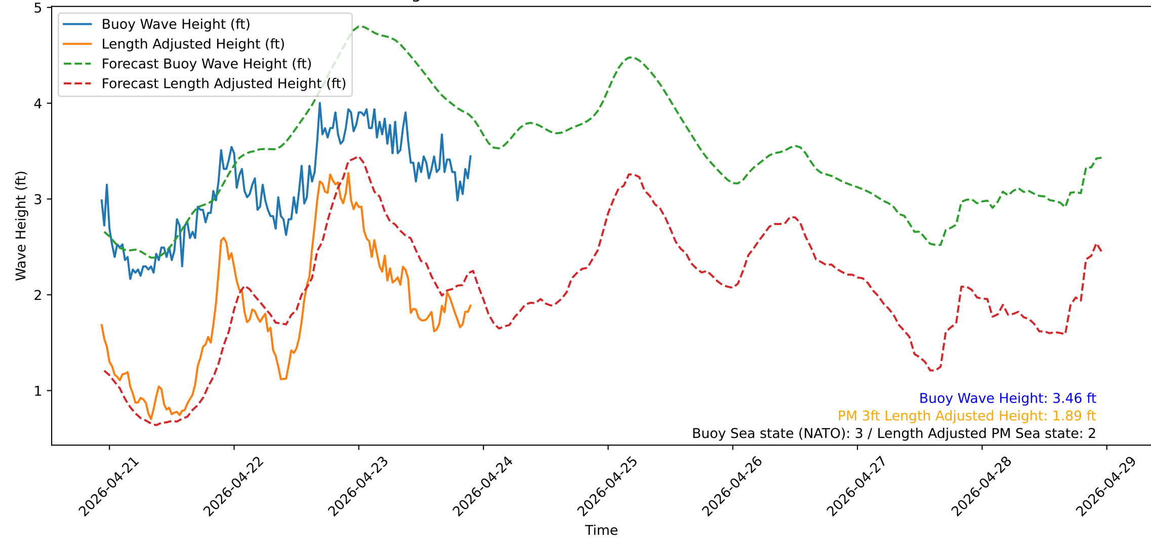
Wave Heights over Time for Green Beach at 2026-04-23 22:31:11
