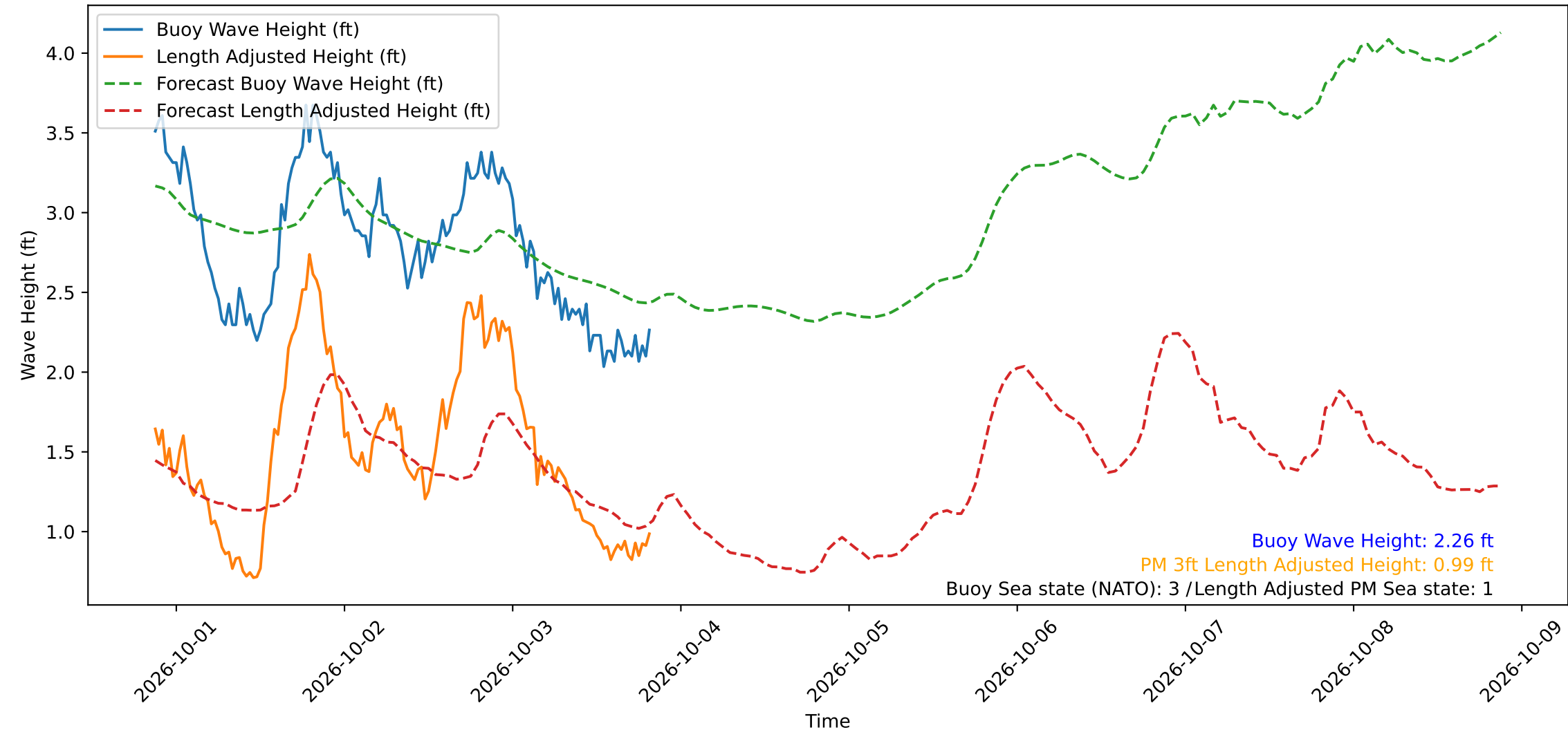
Wave Heights over Time for Green Beach at 2026-10-03 20:31:12
