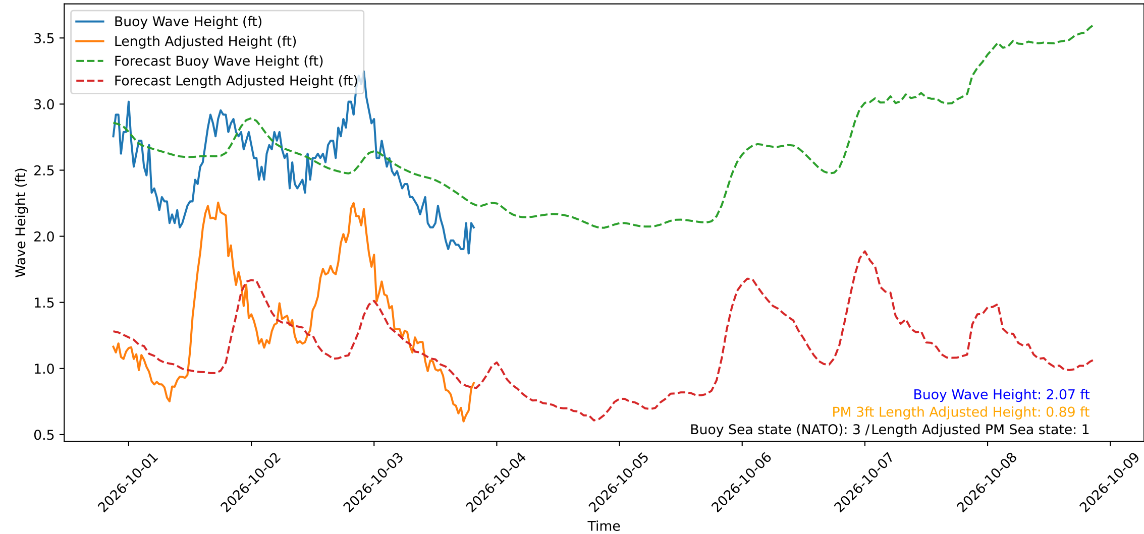
Wave Heights over Time for Red Beach at 2026-10-03 20:30:49
