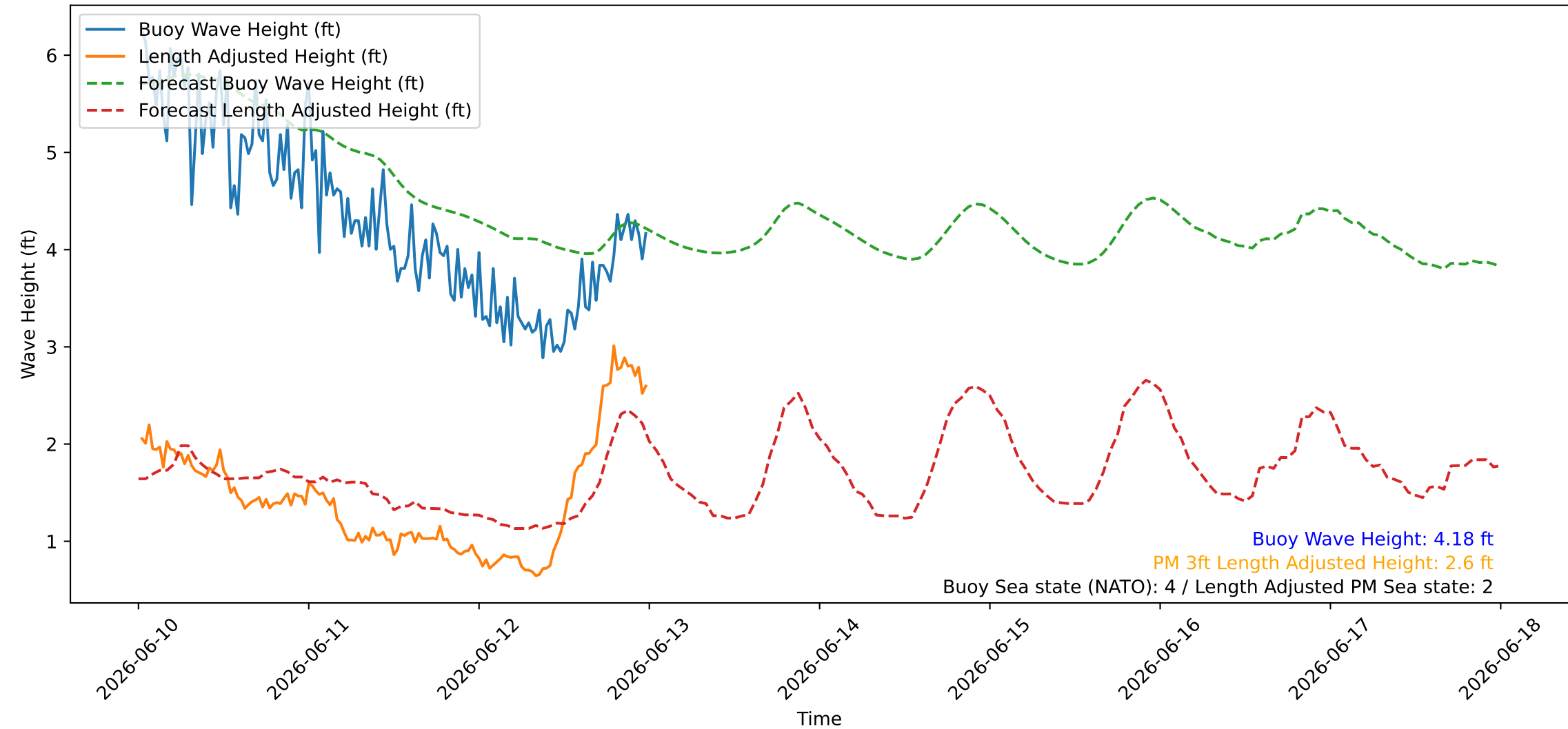
Wave Heights over Time for Green Beach at 2026-06-13 00:21:10
