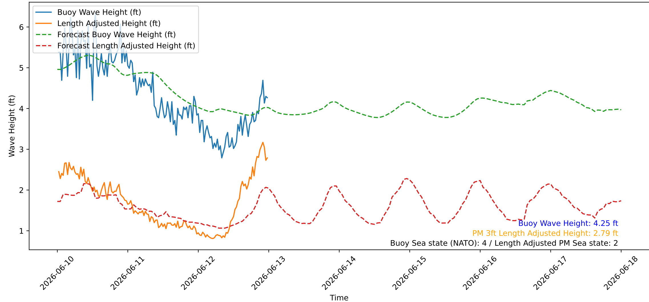
Wave Heights over Time for Oceanside Harbor at 2026-06-13 00:20:26
