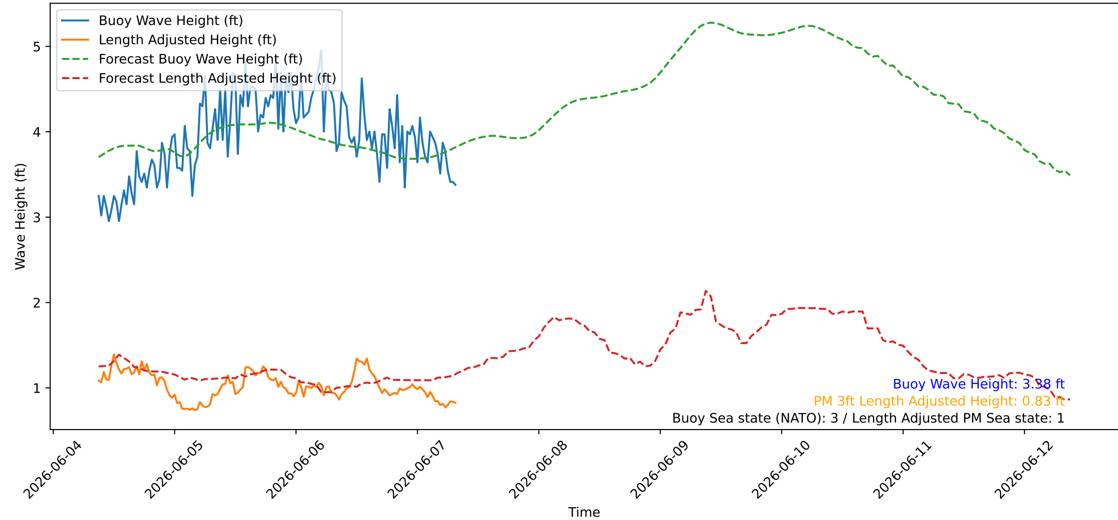
Wave Heights over Time for Red Beach at 2026-06-07 08:30:46
