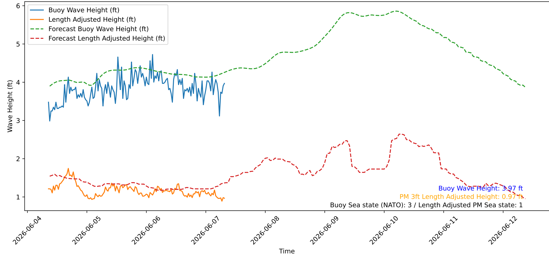
Wave Heights over Time for Green Beach at 2026-06-07 08:31:08
