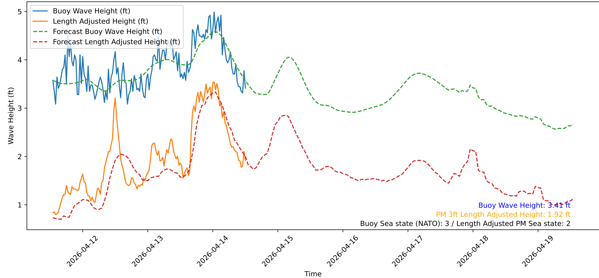
Wave Heights over Time for Green Beach at 2026-04-14 12:51:13
