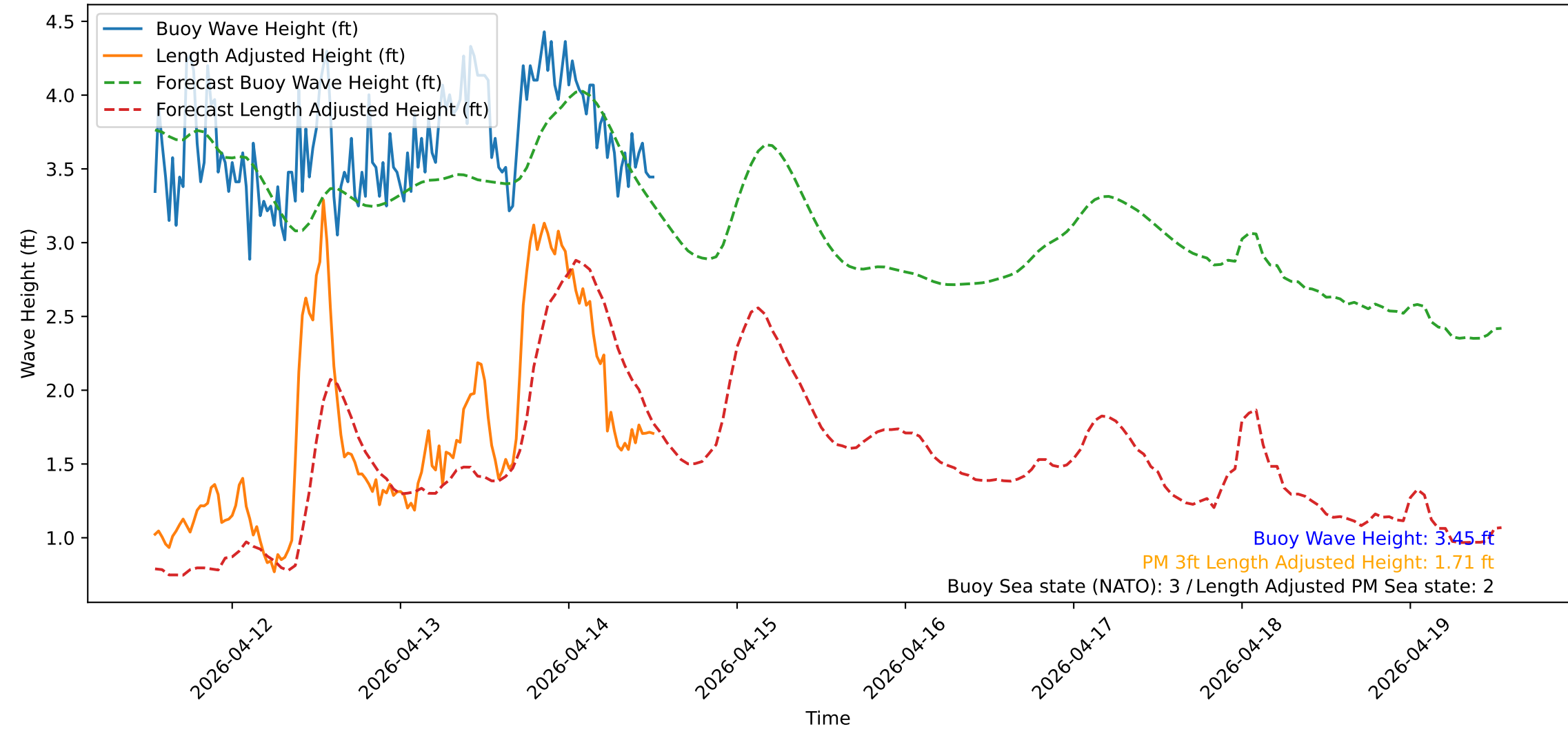
Wave Heights over Time for Red Beach at 2026-04-14 12:50:51
