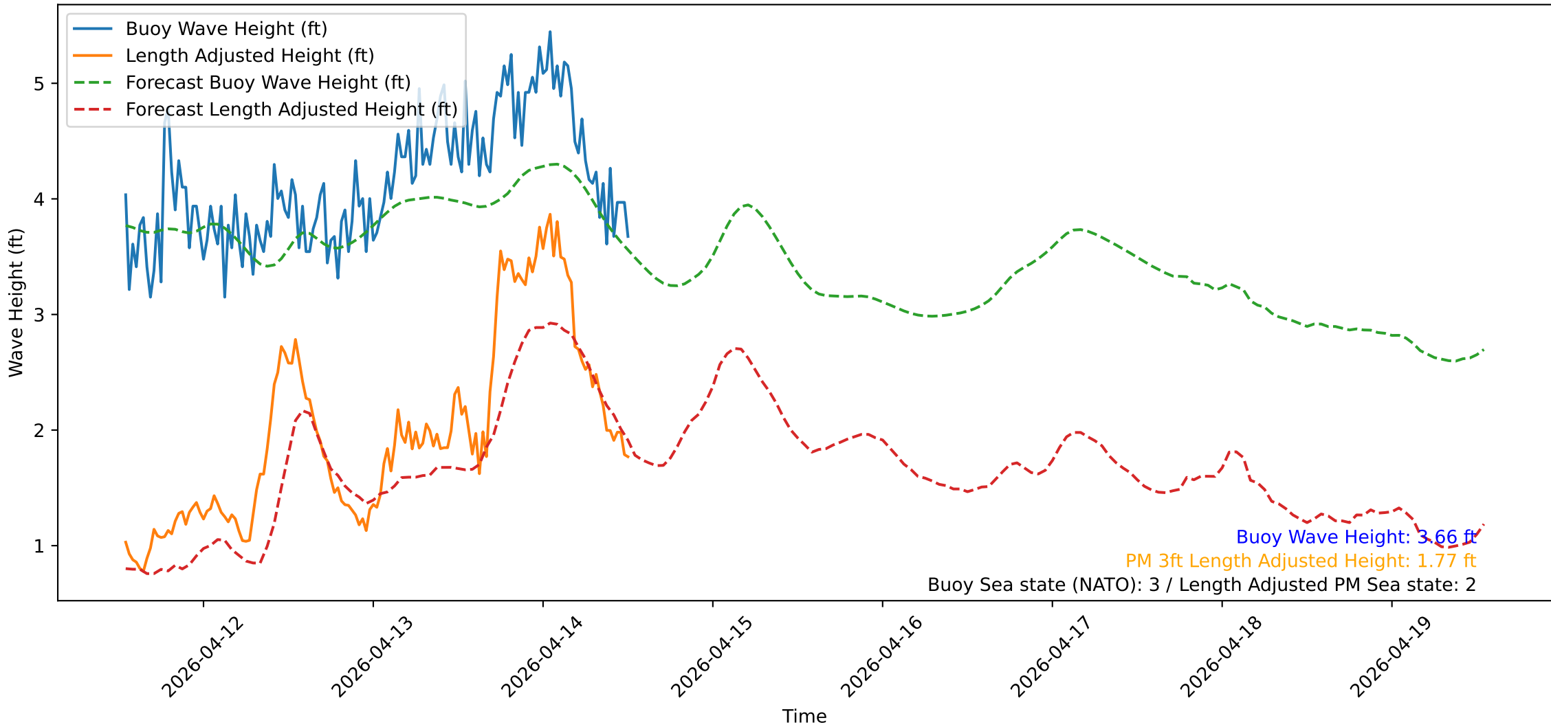
Wave Heights over Time for Oceanside Harbor at 2026-04-14 12:50:31
