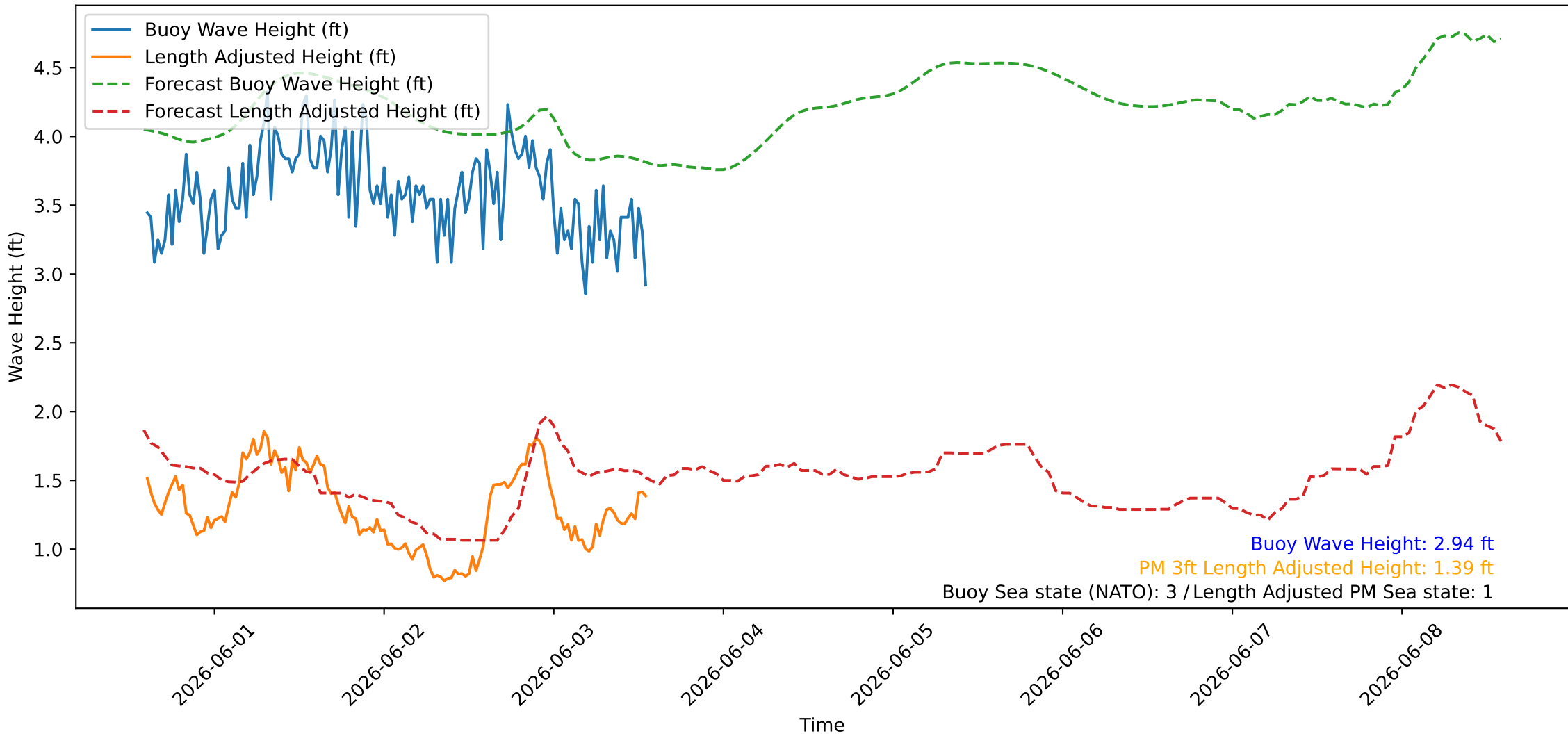
Wave Heights over Time for Green Beach at 2026-06-03 14:21:08
