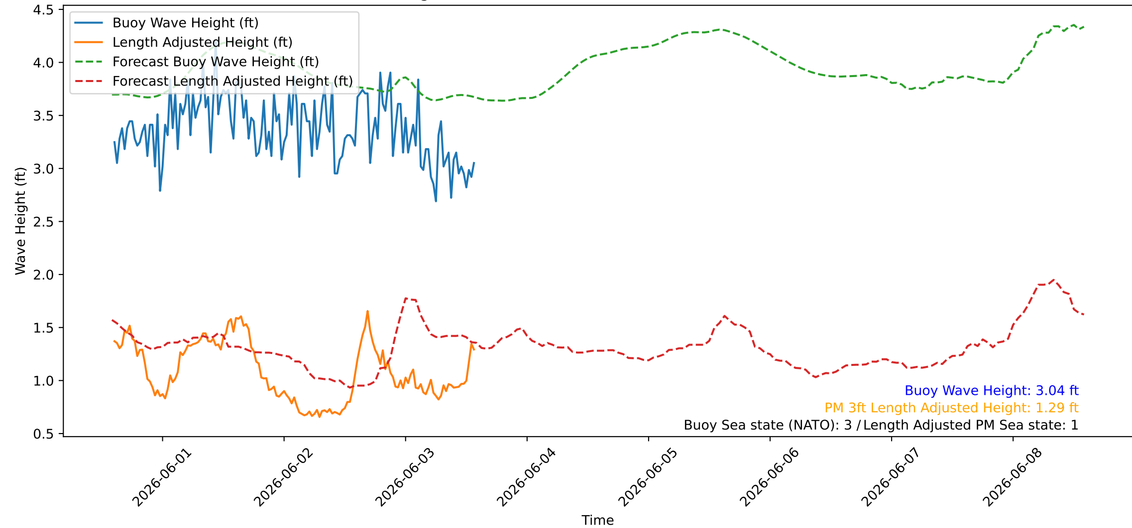
Wave Heights over Time for Red Beach at 2026-06-03 14:20:46
