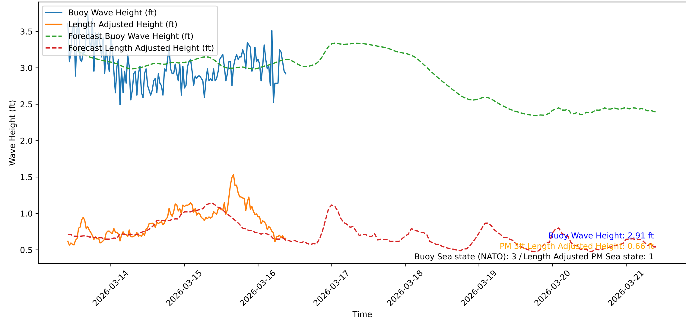
Wave Heights over Time for Red Beach at 2026-03-16 09:51:03
