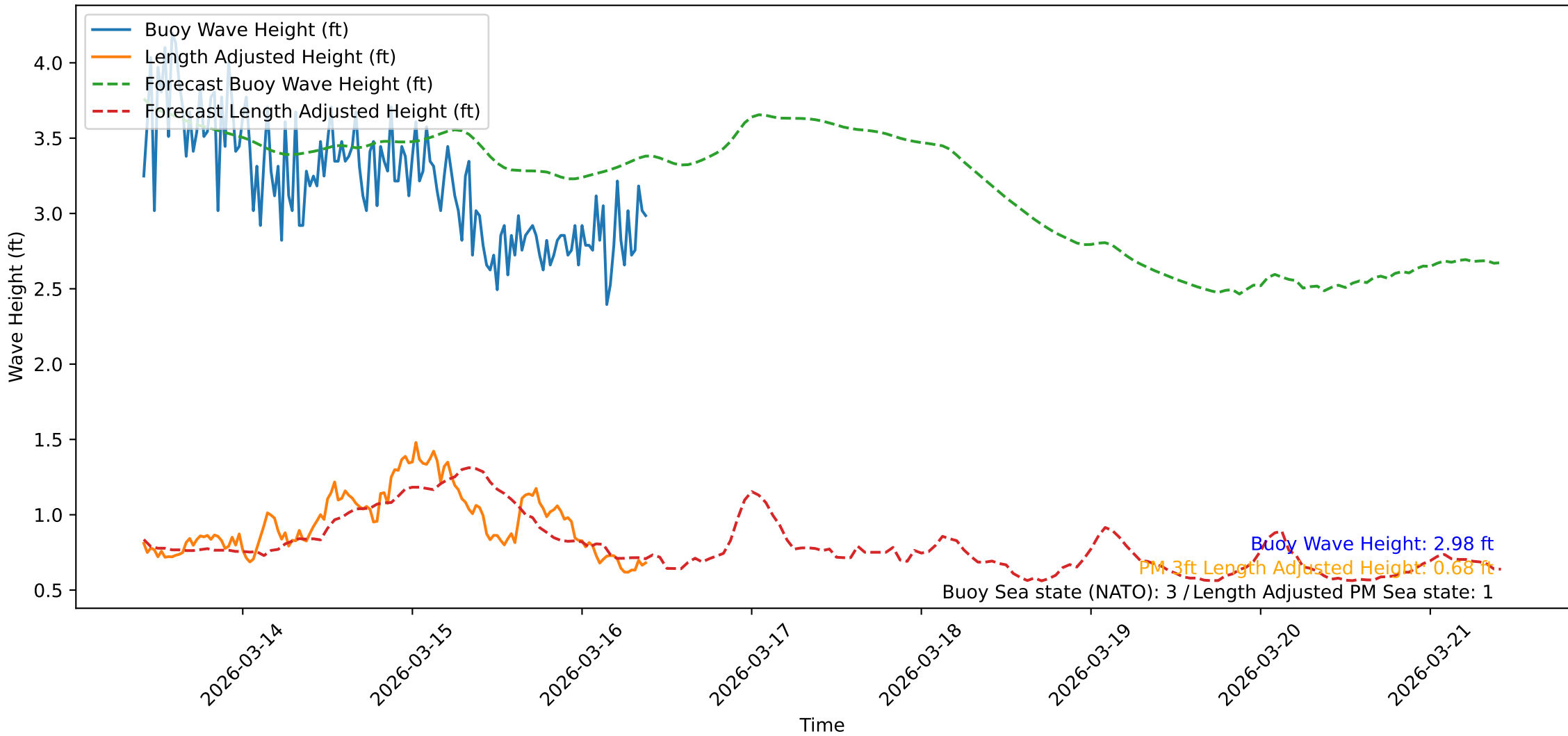
Wave Heights over Time for Oceanside Harbor at 2026-03-16 09:50:41
