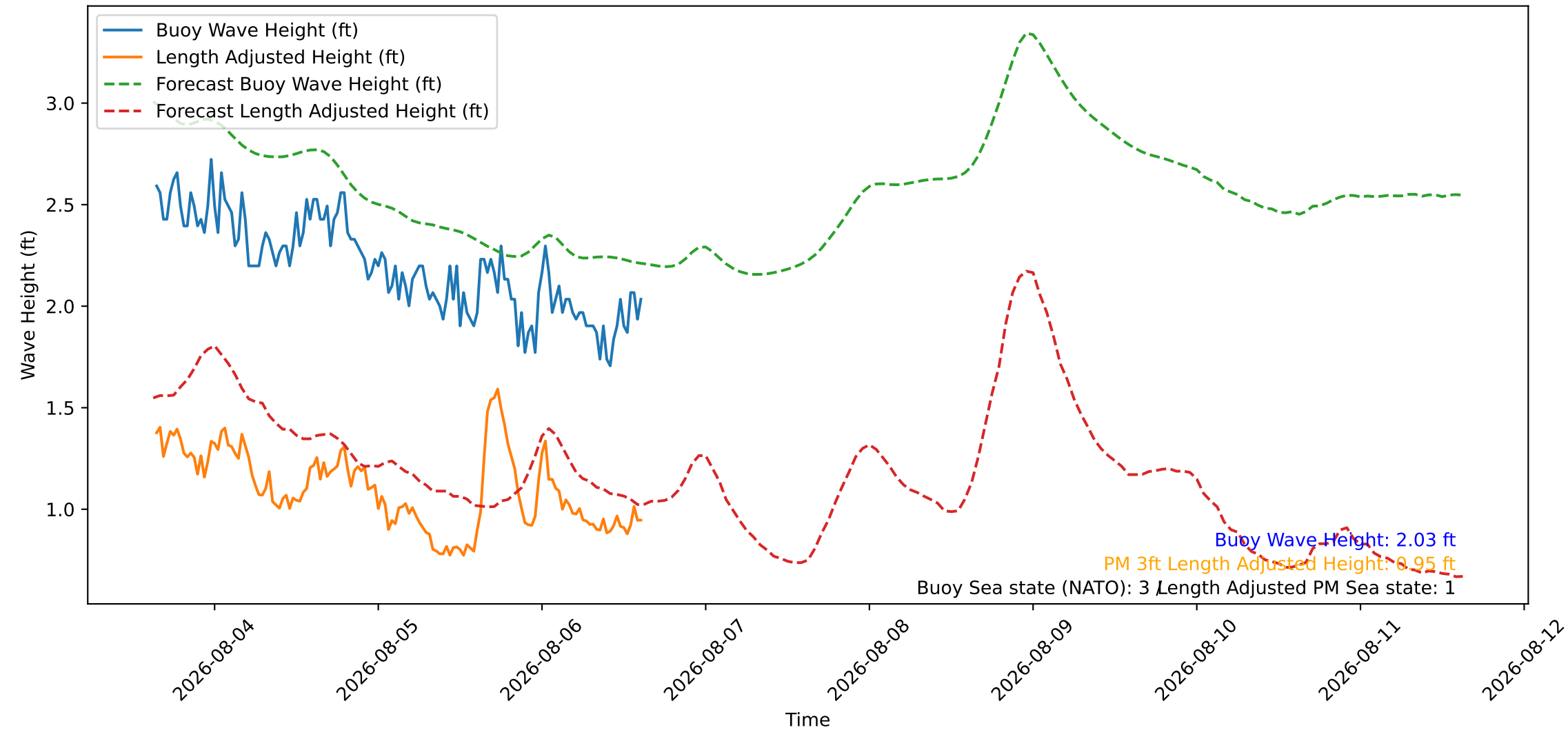
Wave Heights over Time for Oceanside Harbor at 2026-08-06 15:20:26
