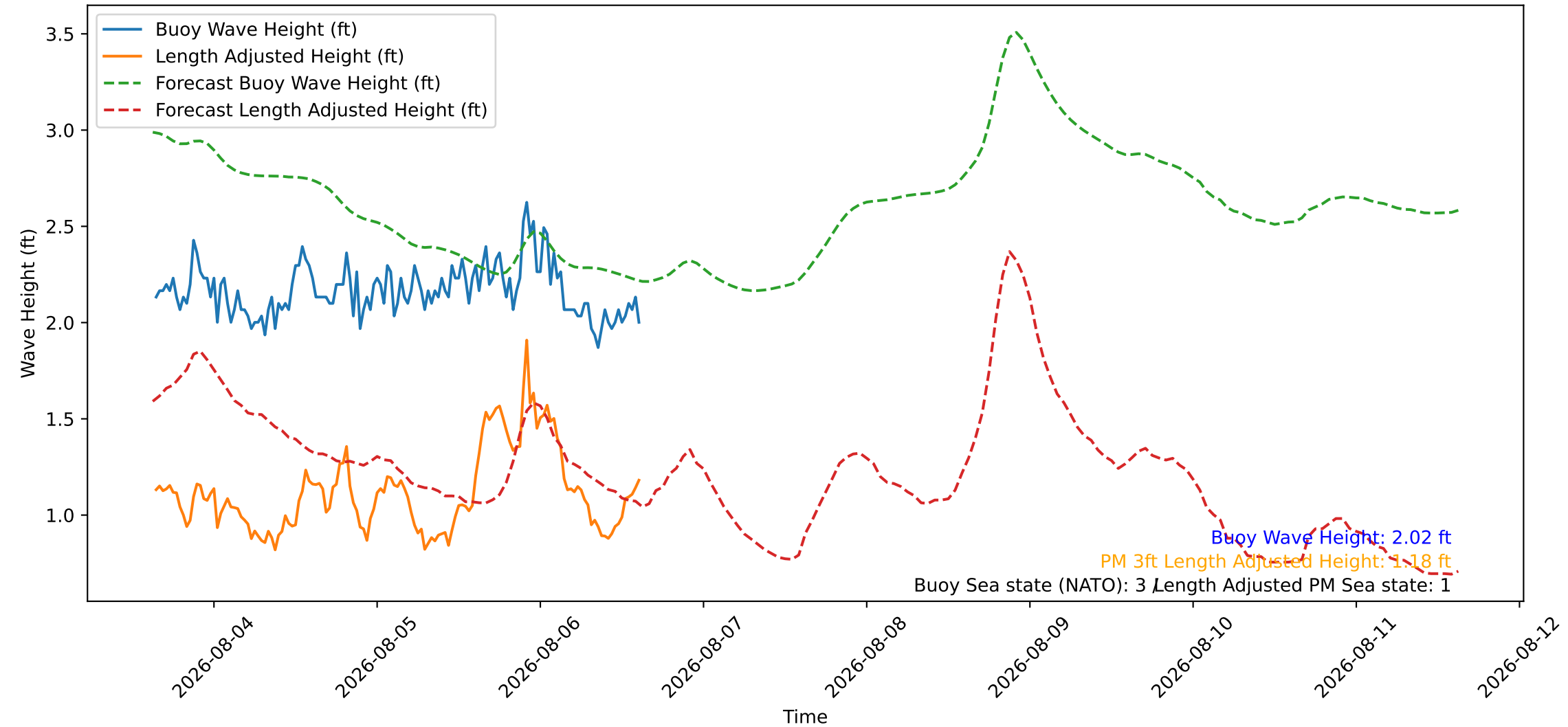
Wave Heights over Time for Green Beach at 2026-08-06 15:21:08
