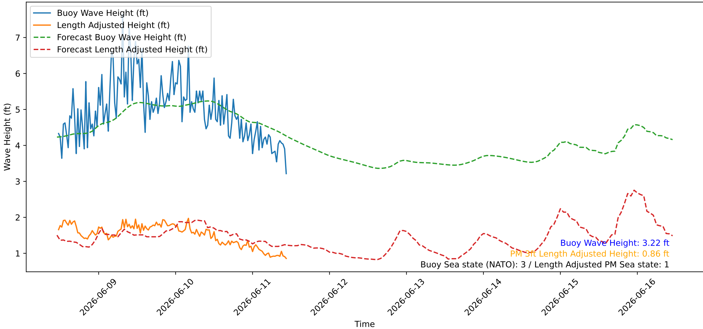
Wave Heights over Time for Red Beach at 2026-06-11 11:20:47
