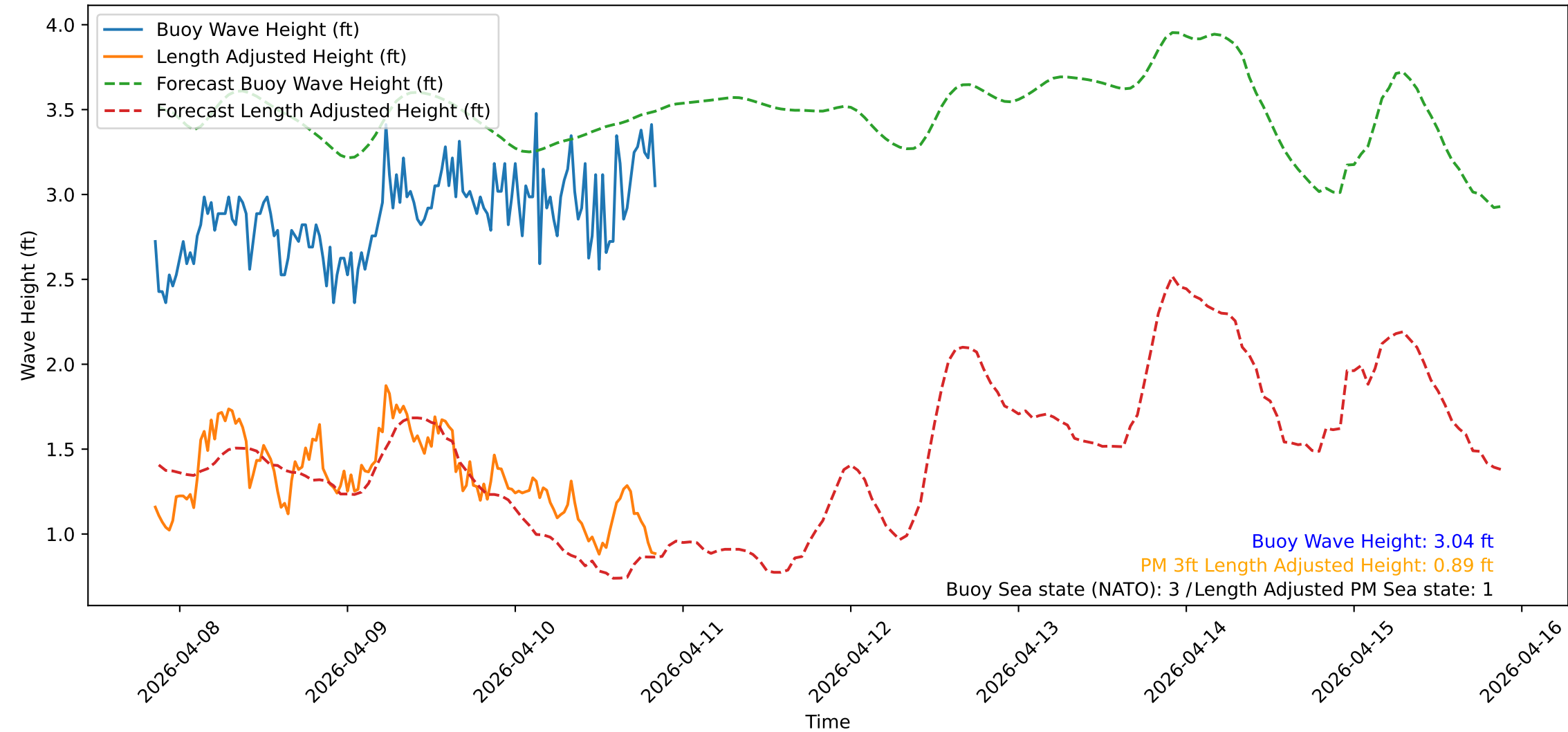
Wave Heights over Time for Green Beach at 2026-04-10 20:41:13
