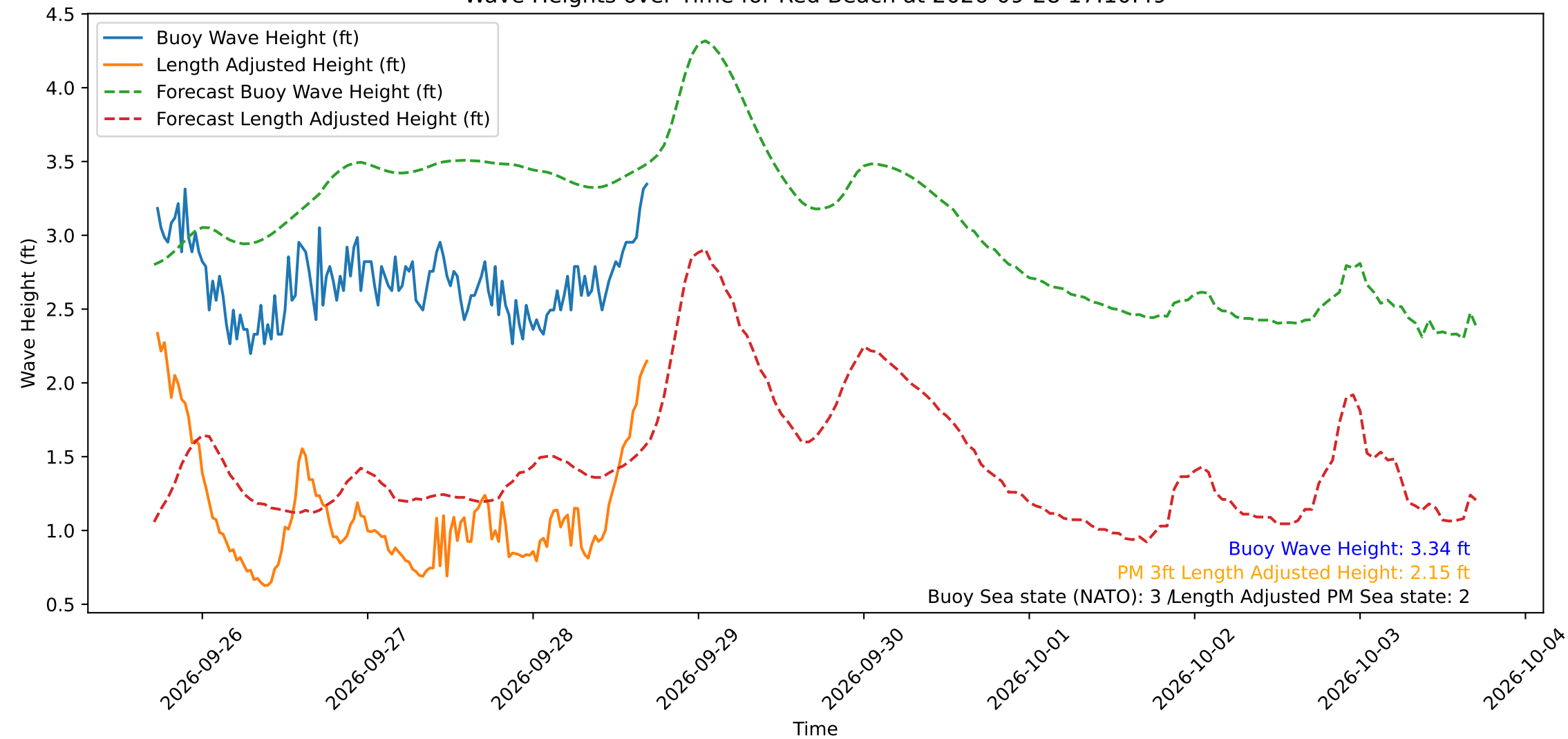
Wave Heights over Time for Red Beach at 2026-09-28 17:10:49
