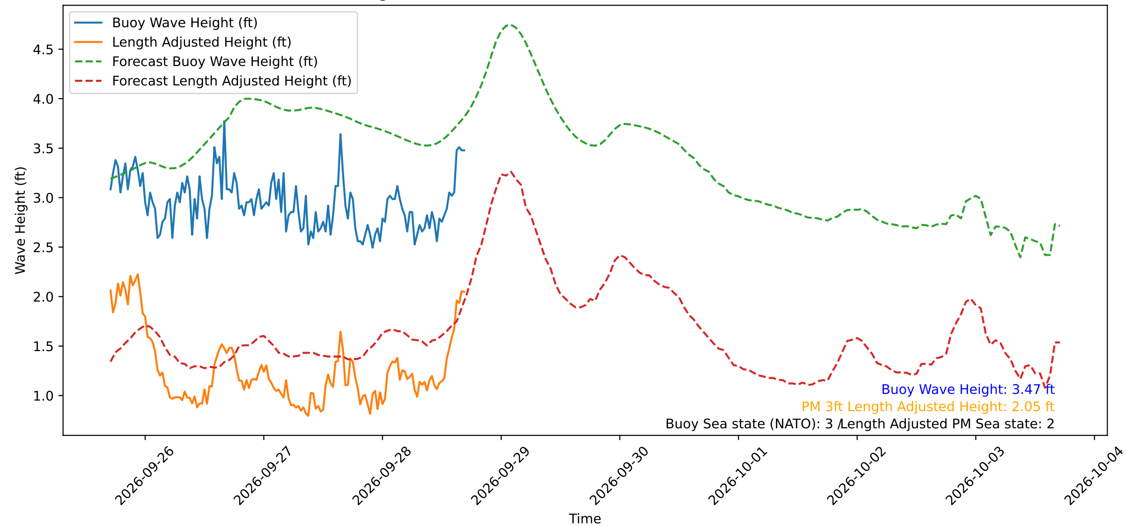
Wave Heights over Time for Oceanside Harbor at 2026-09-28 17:10:29
