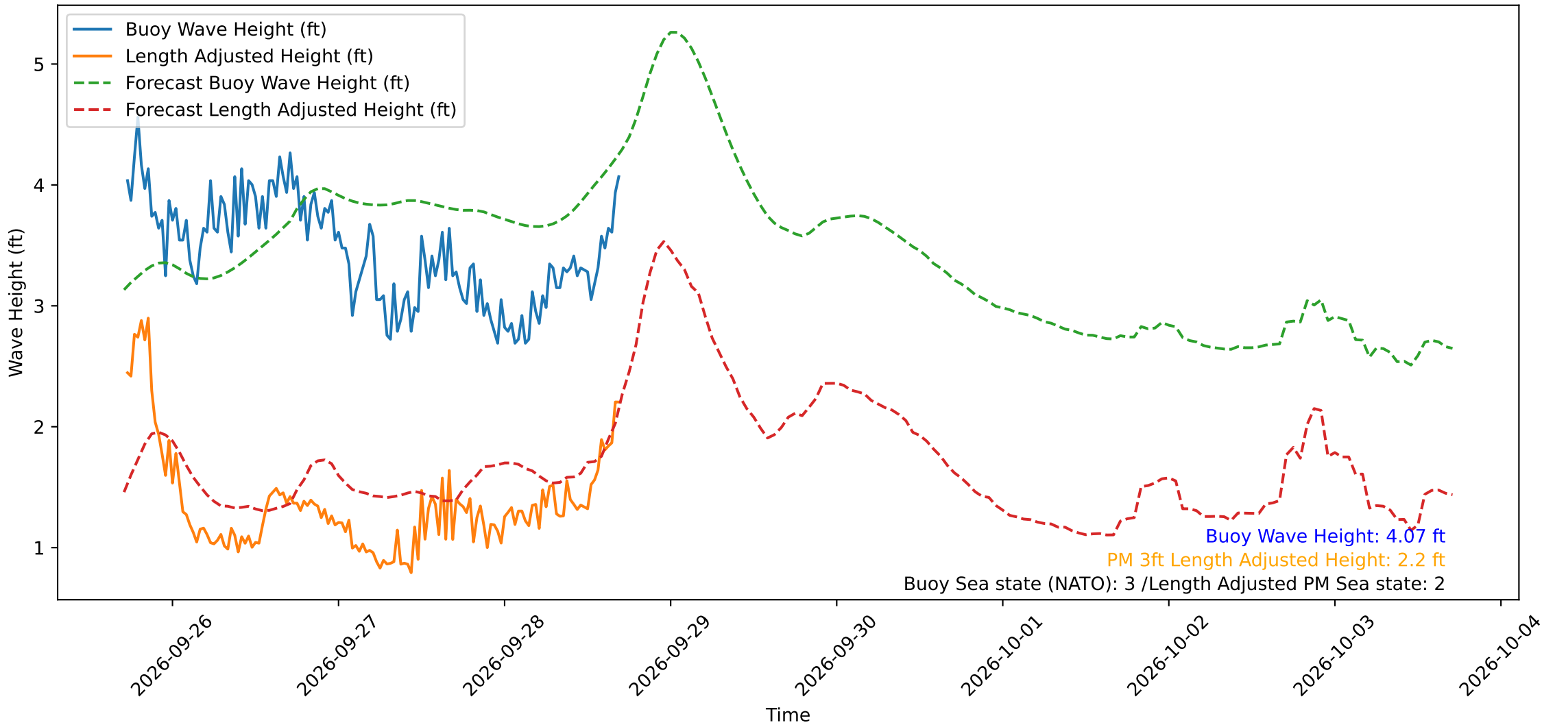
Wave Heights over Time for Green Beach at 2026-09-28 17:11:11
