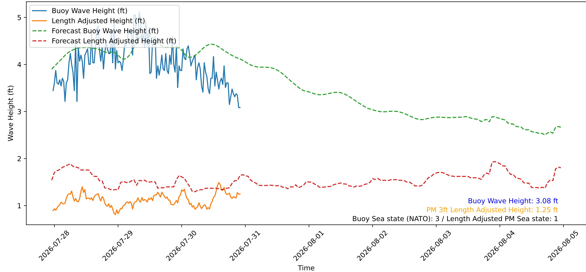
Wave Heights over Time for Red Beach at 2026-07-30 23:00:53
