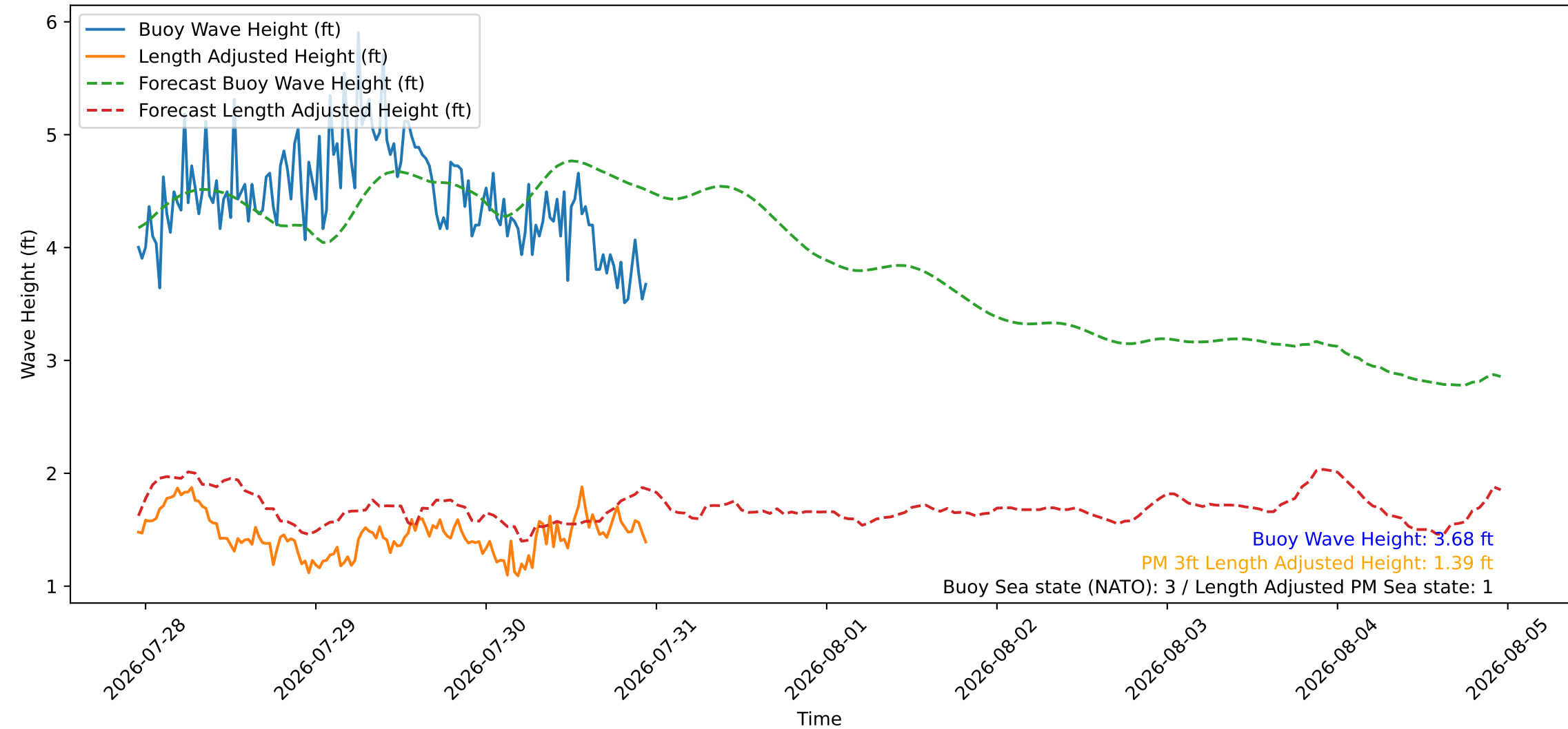
Wave Heights over Time for Oceanside Harbor at 2026-07-30 23:00:30
