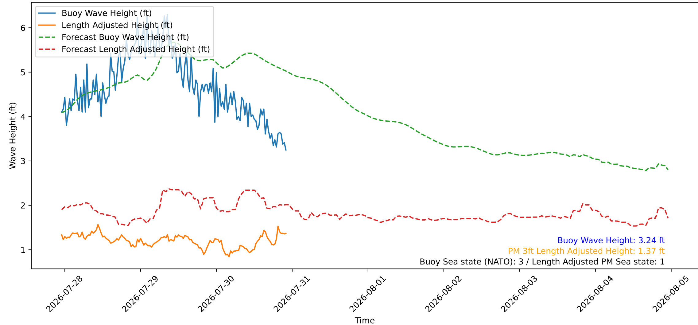
Wave Heights over Time for Green Beach at 2026-07-30 23:01:22
