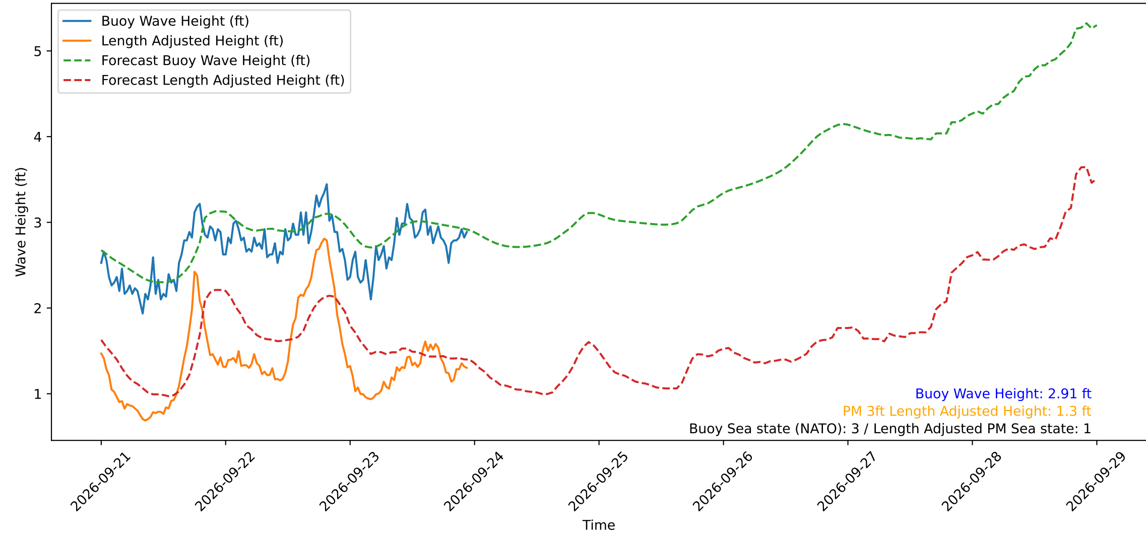
Wave Heights over Time for Green Beach at 2026-09-23 23:31:11
