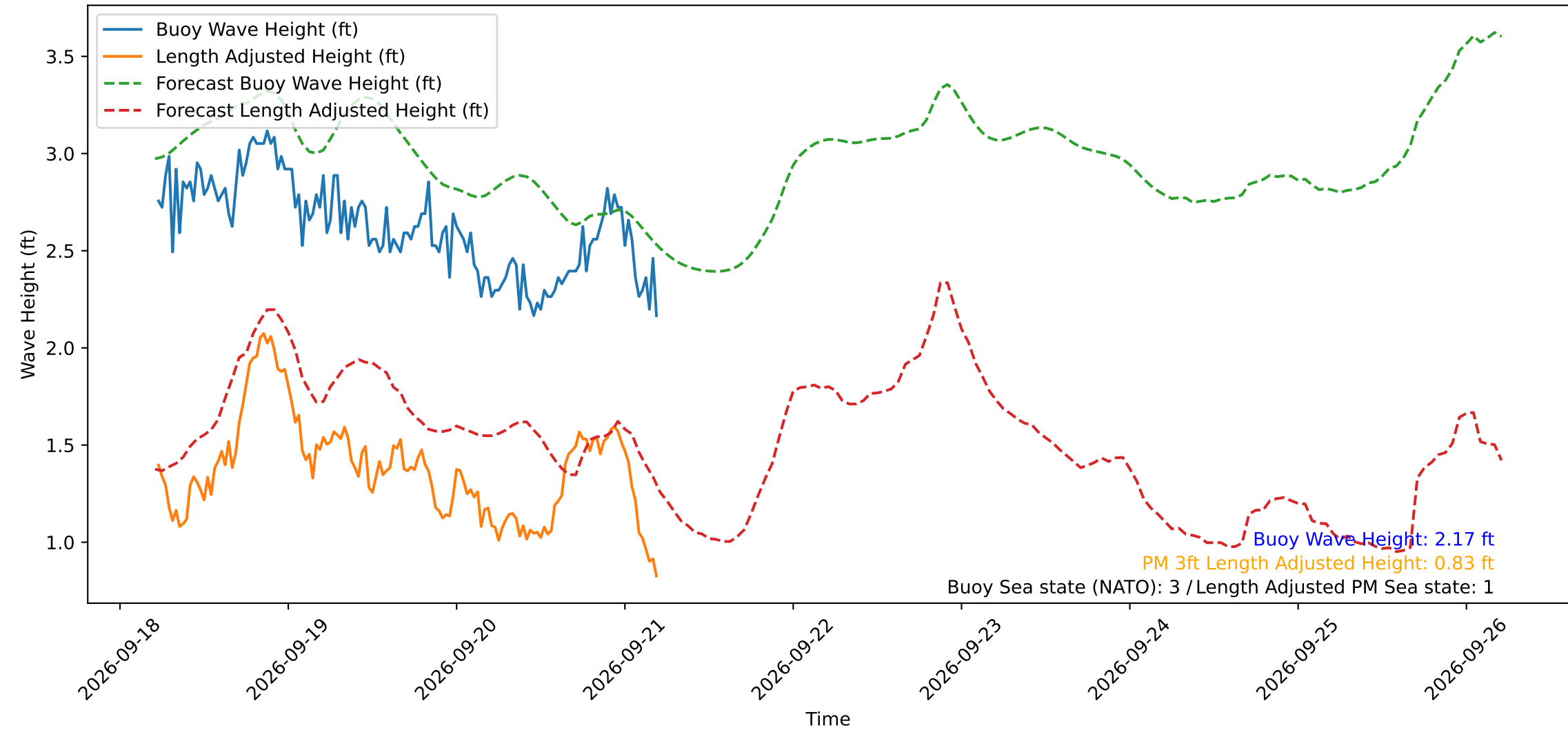
Wave Heights over Time for Green Beach at 2026-09-21 05:11:13
