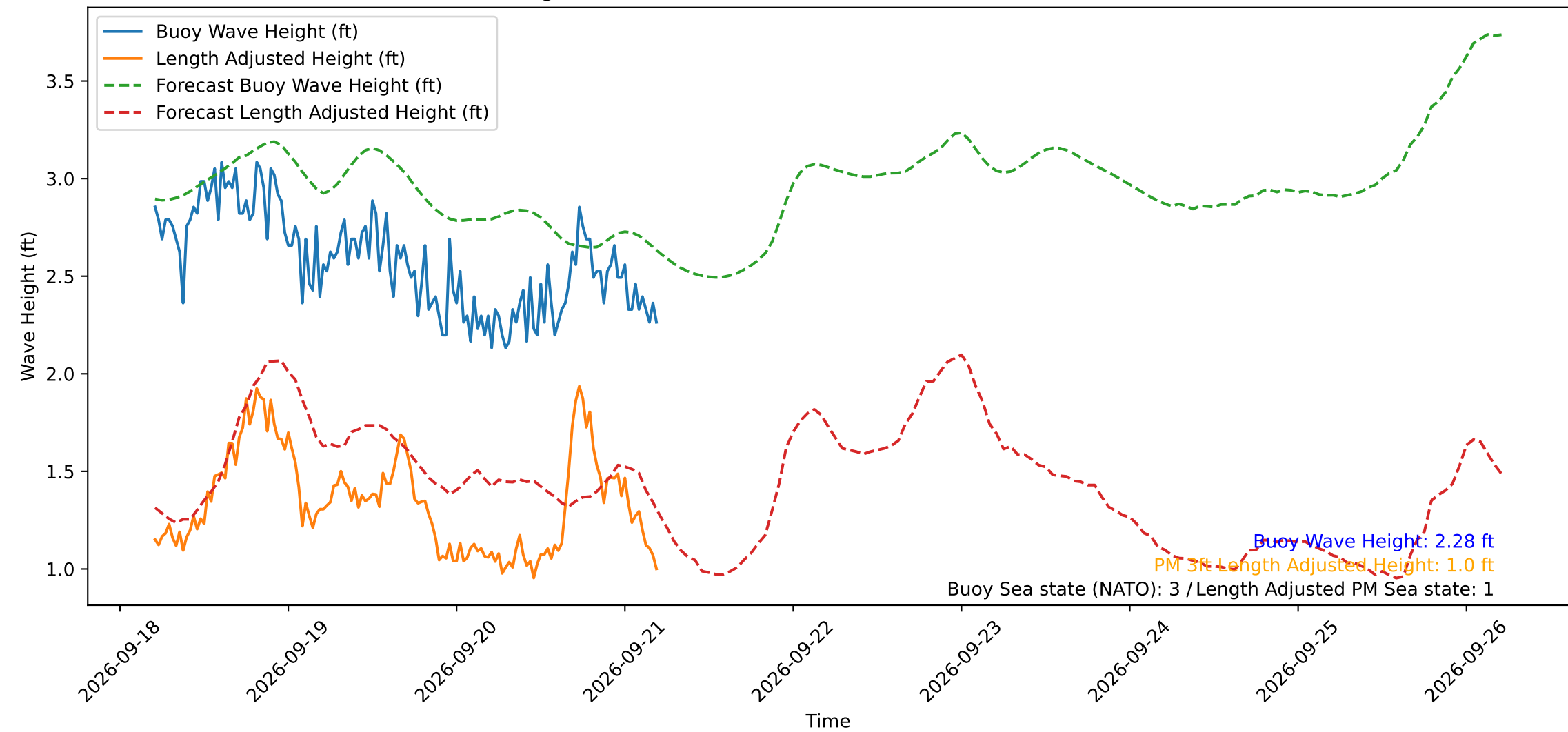
Wave Heights over Time for Oceanside Harbor at 2026-09-21 05:10:30
