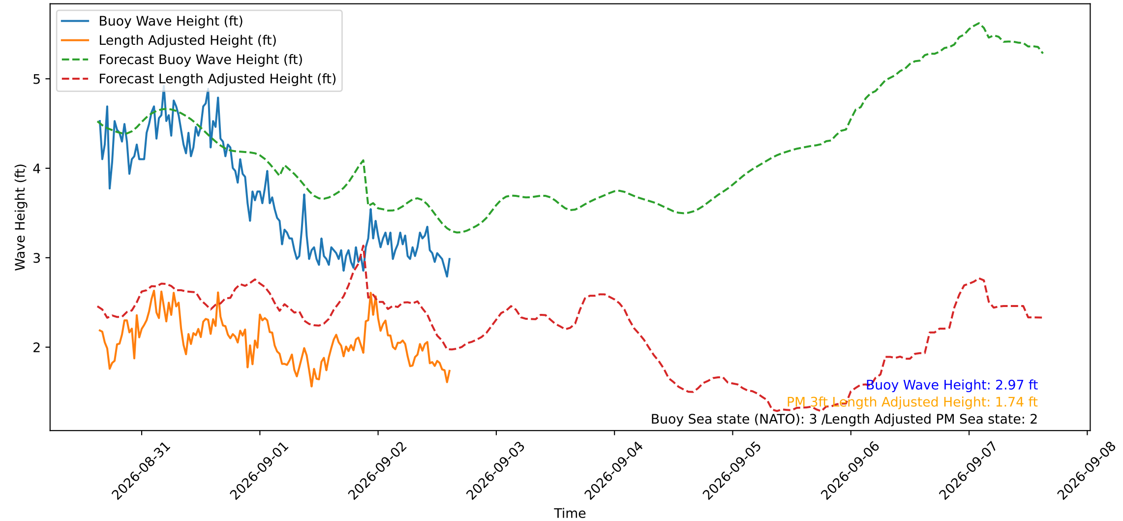
Wave Heights over Time for Oceanside Harbor at 2026-09-02 15:20:29
