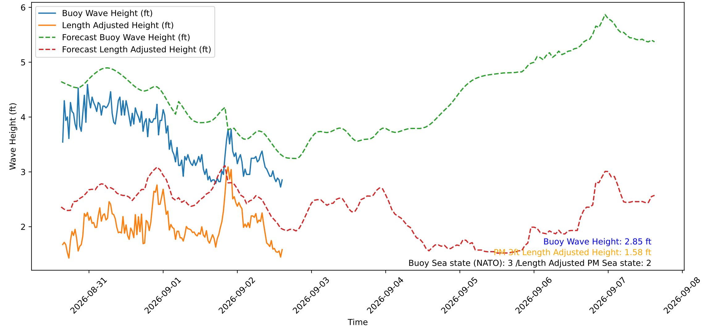
Wave Heights over Time for Green Beach at 2026-09-02 15:21:14
