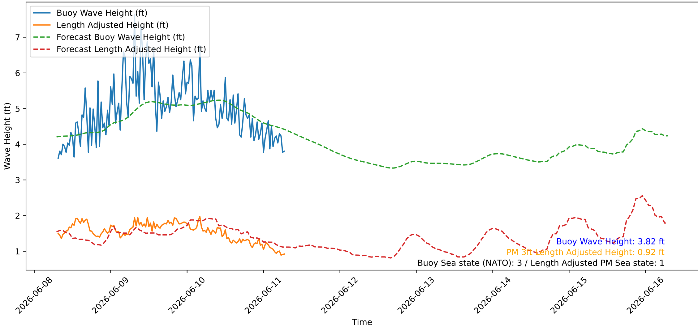
Wave Heights over Time for Red Beach at 2026-06-11 07:20:47
