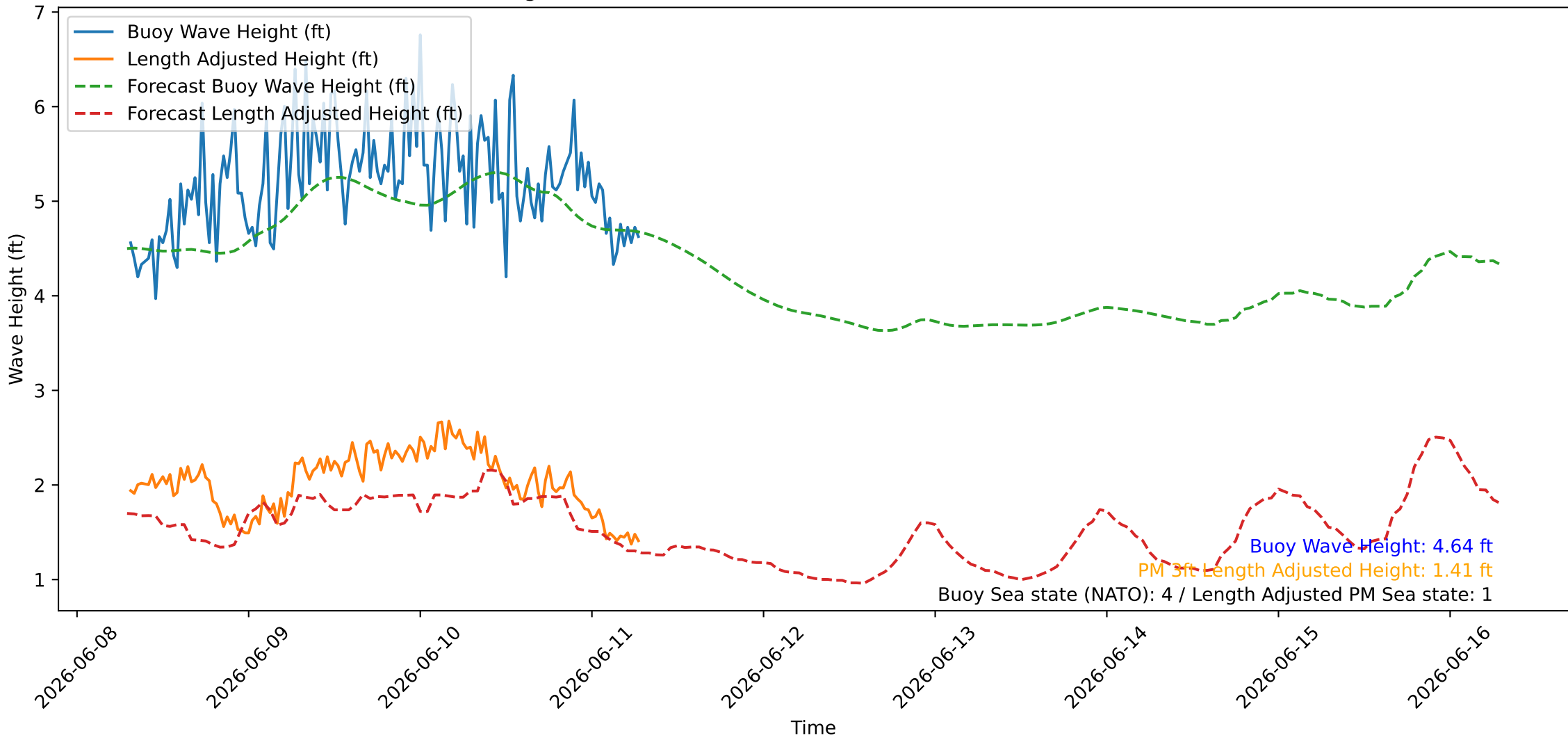
Wave Heights over Time for Oceanside Harbor at 2026-06-11 07:20:26
