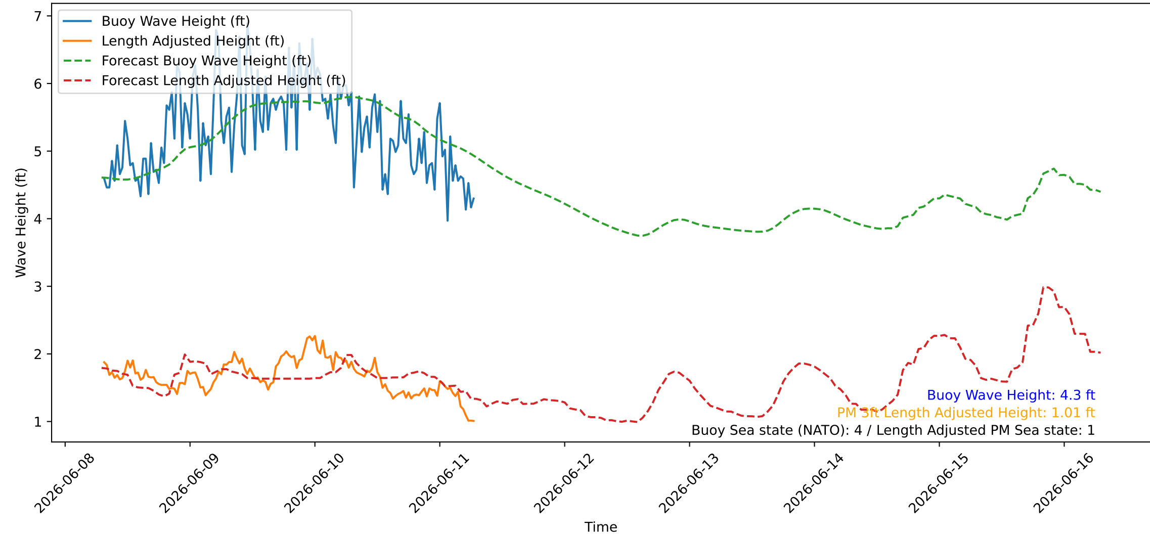
Wave Heights over Time for Green Beach at 2026-06-11 07:21:10
