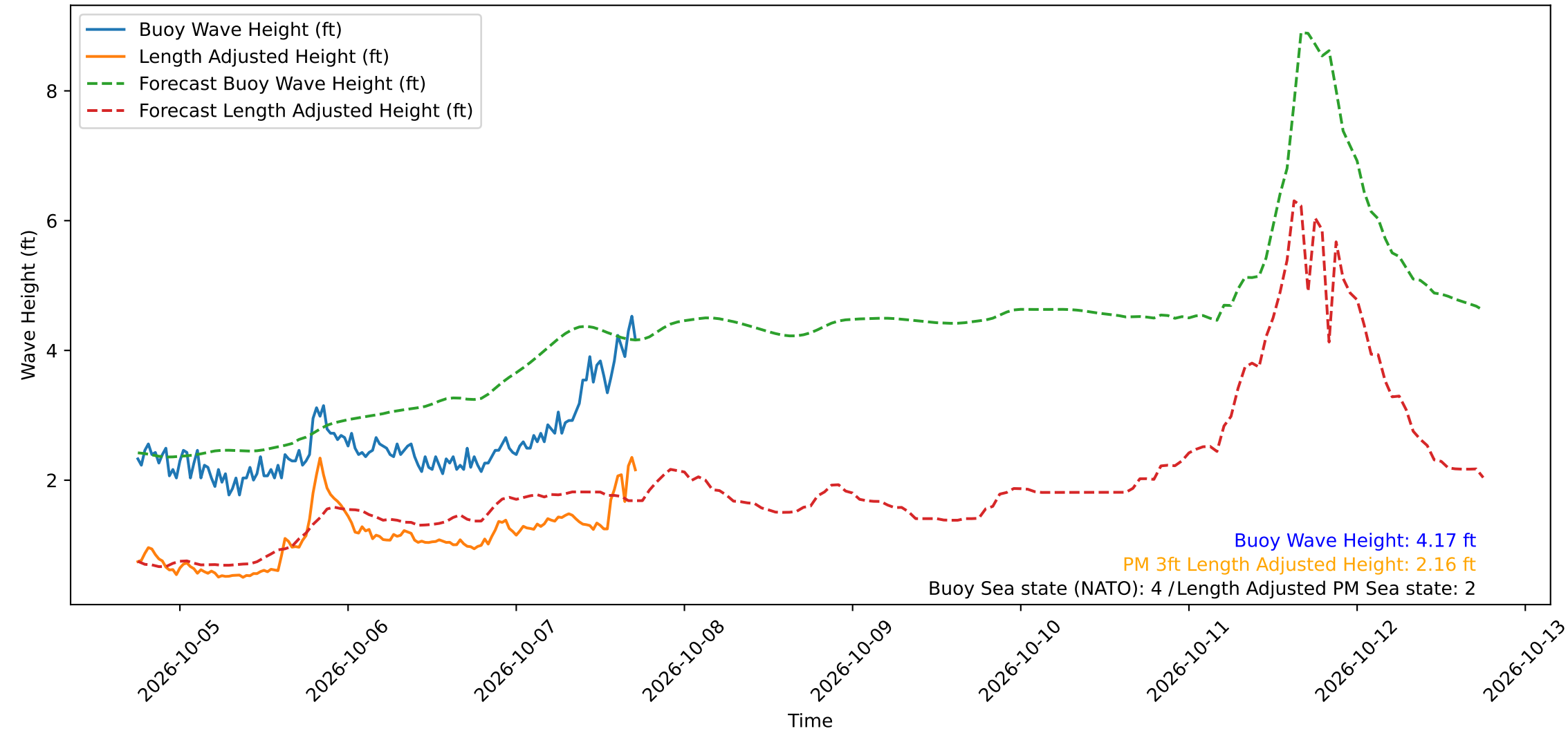
Wave Heights over Time for Green Beach at 2026-10-07 17:41:13
