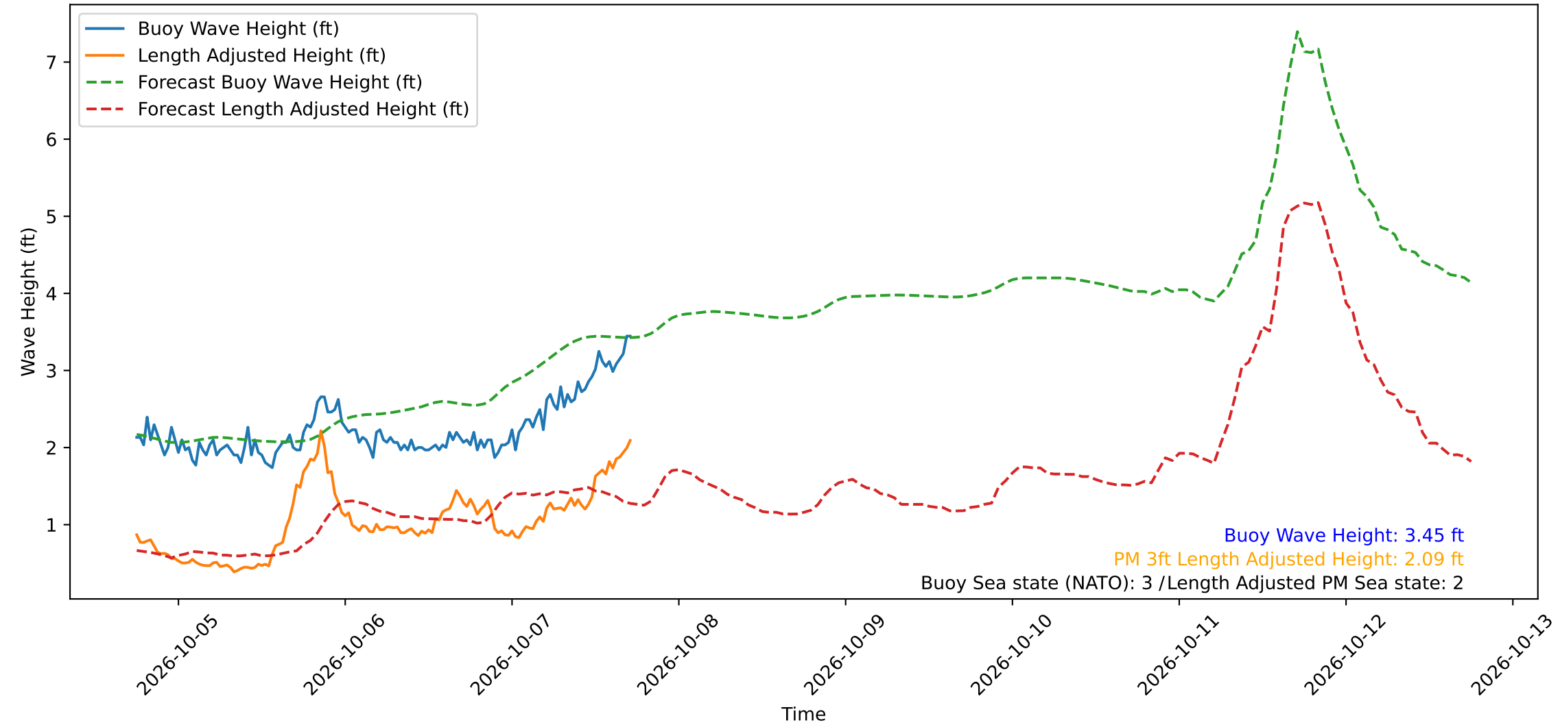
Wave Heights over Time for Red Beach at 2026-10-07 17:40:49
