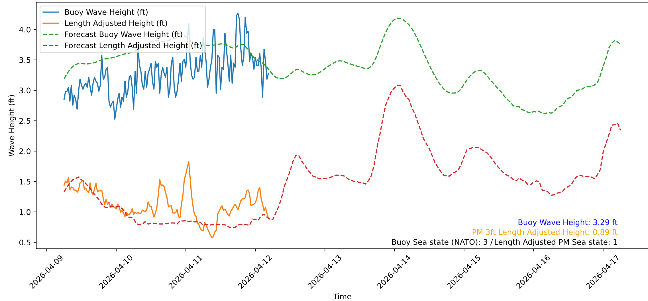
Wave Heights over Time for Red Beach at 2026-04-12 05:50:52
