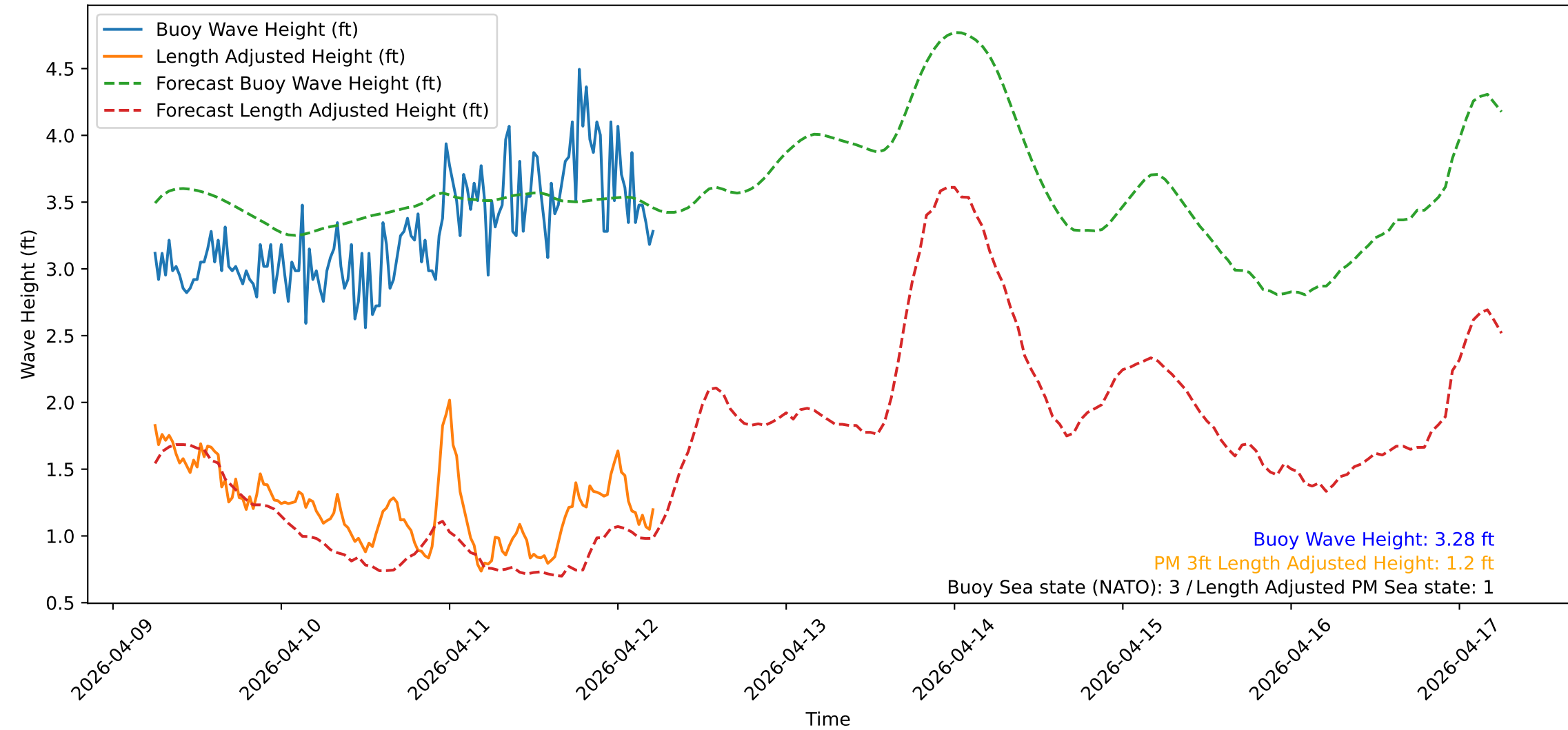
Wave Heights over Time for Green Beach at 2026-04-12 05:51:14
