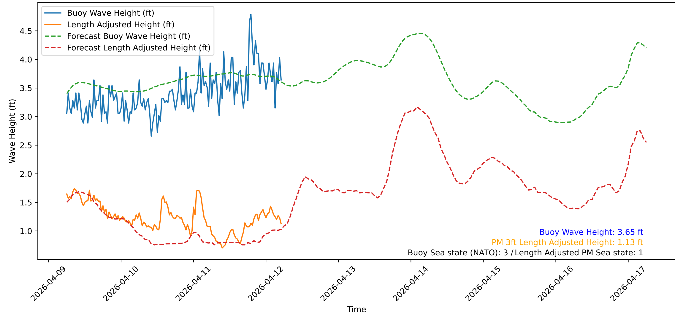
Wave Heights over Time for Oceanside Harbor at 2026-04-12 05:50:32
