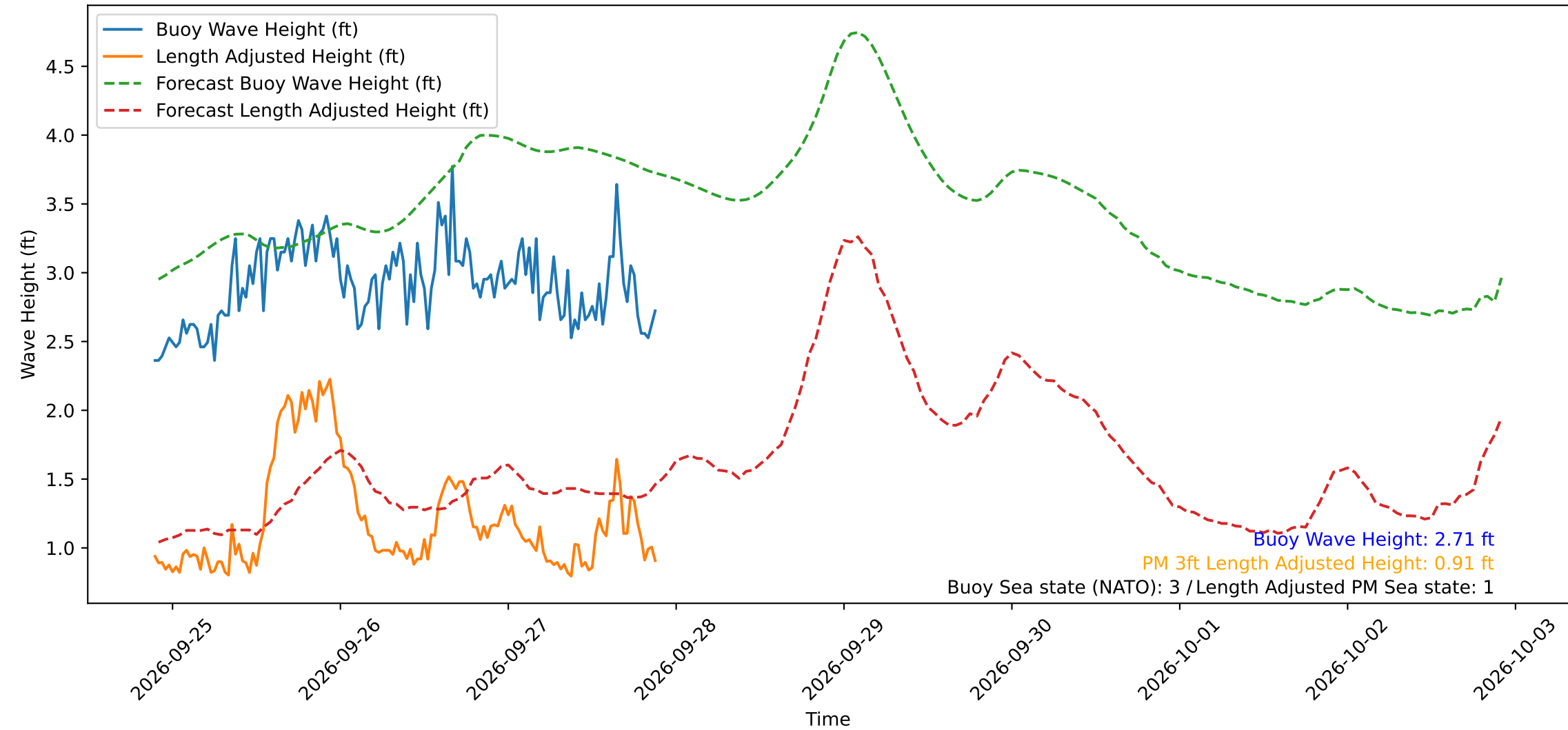
Wave Heights over Time for Oceanside Harbor at 2026-09-27 21:40:30
