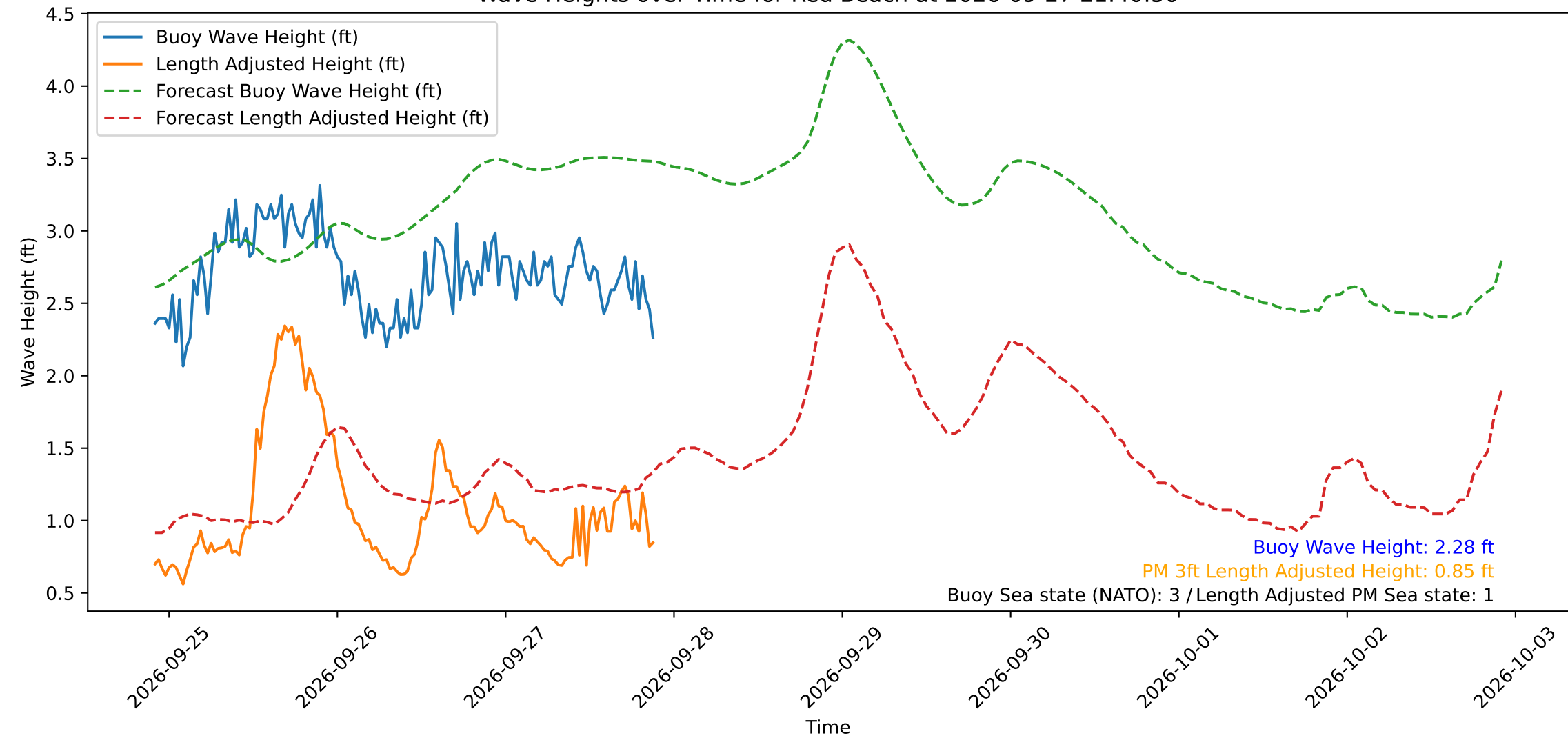
Wave Heights over Time for Red Beach at 2026-09-27 21:40:50
