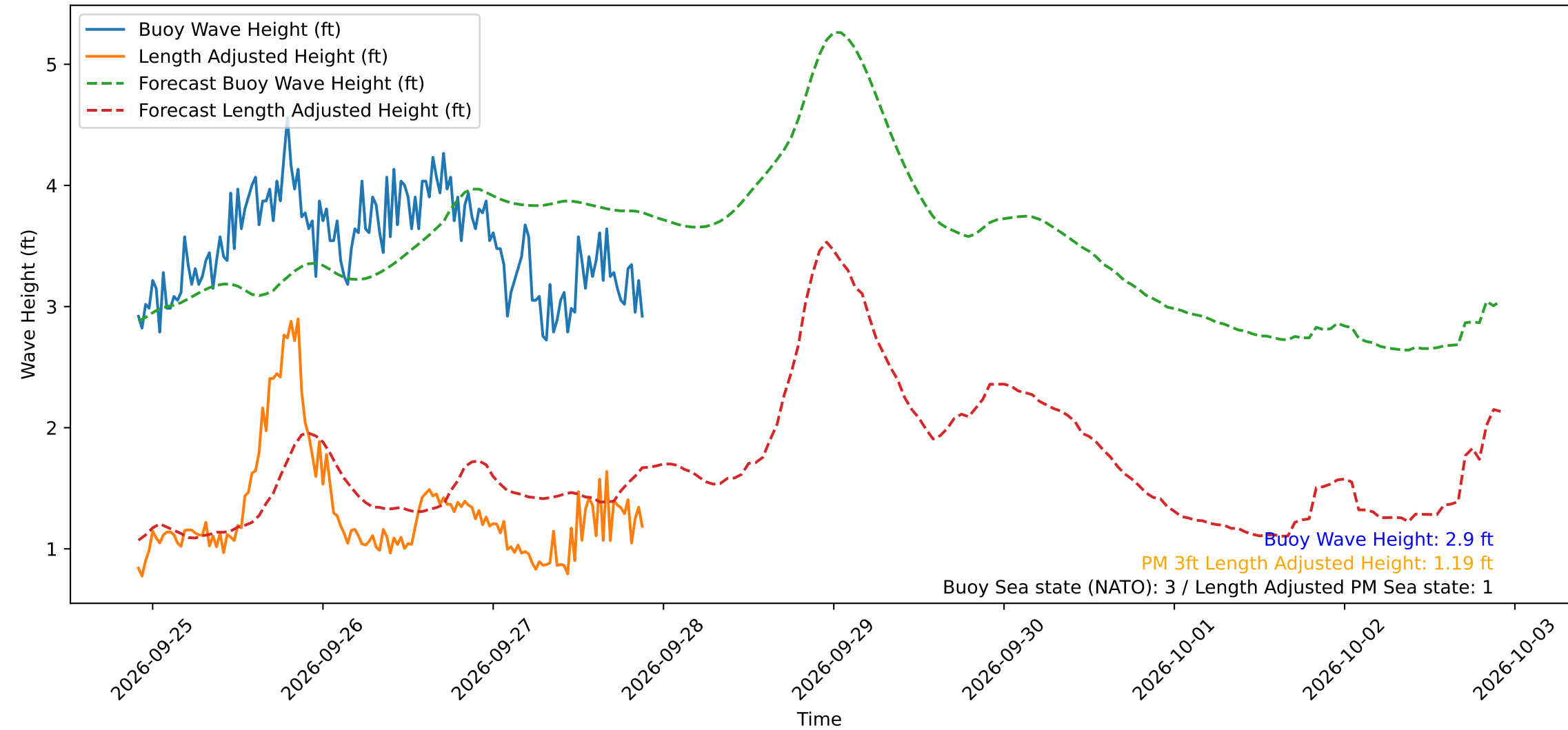
Wave Heights over Time for Green Beach at 2026-09-27 21:41:13
