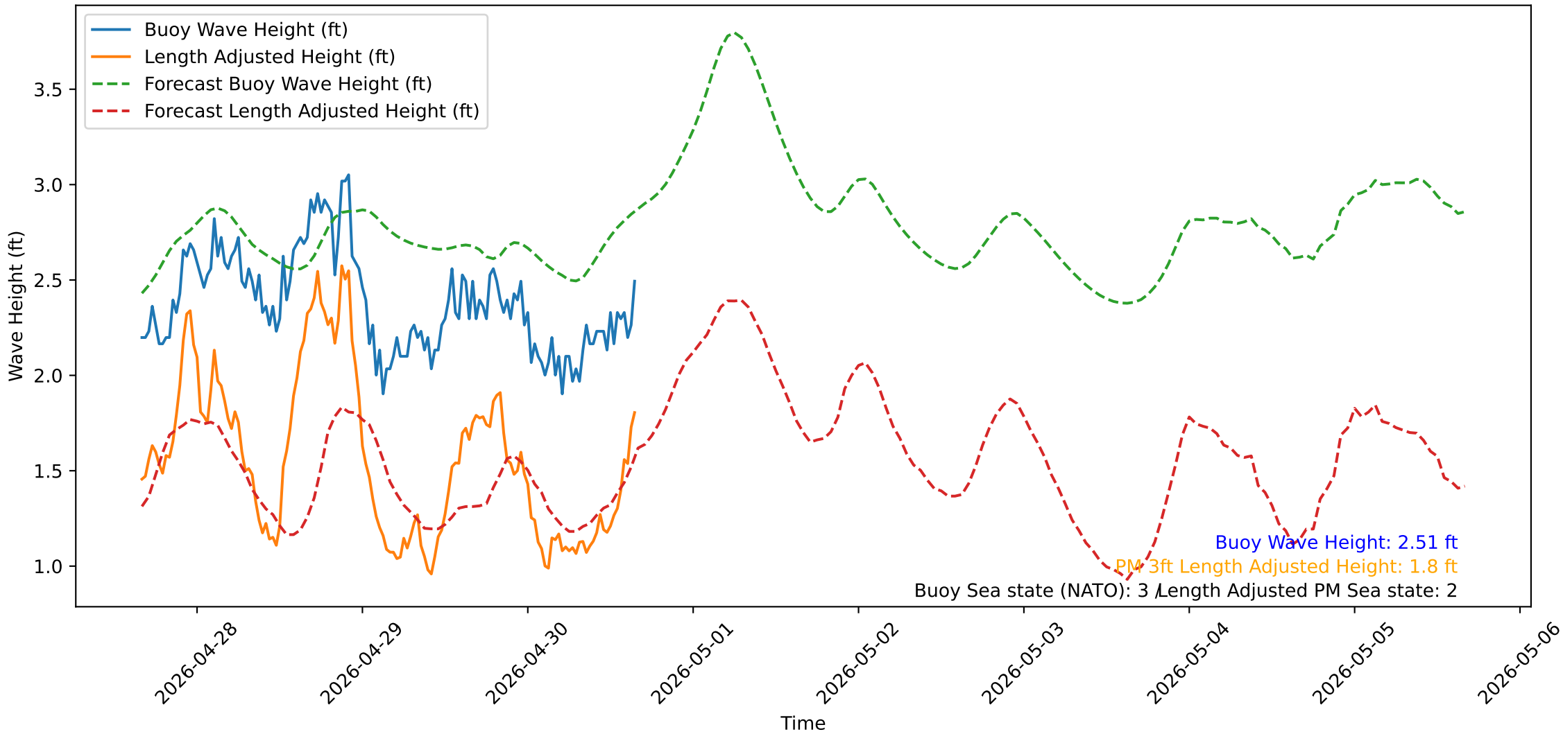
Wave Heights over Time for Oceanside Harbor at 2026-04-30 16:10:31
