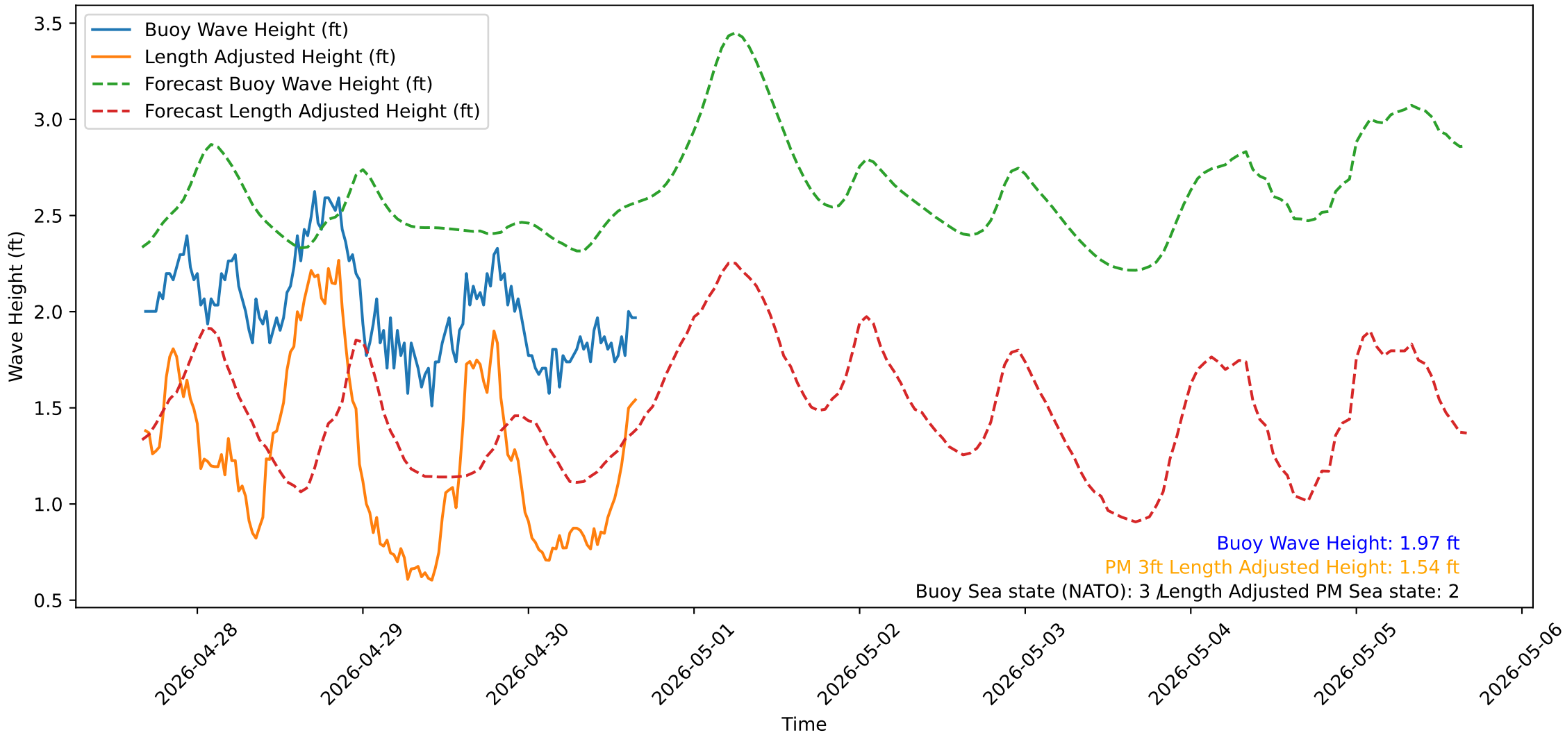
Wave Heights over Time for Red Beach at 2026-04-30 16:10:51
