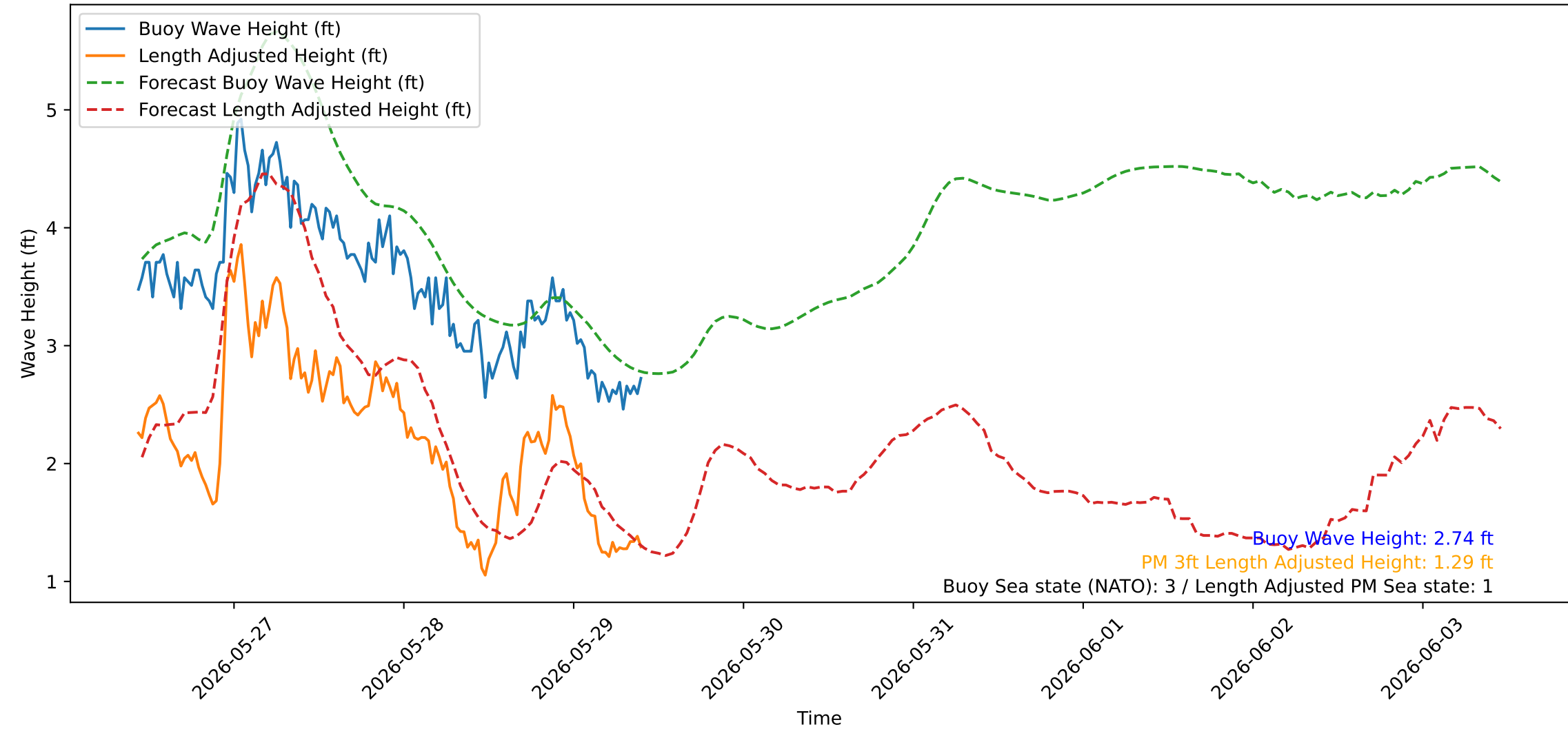
Wave Heights over Time for Green Beach at 2026-05-29 10:31:04
