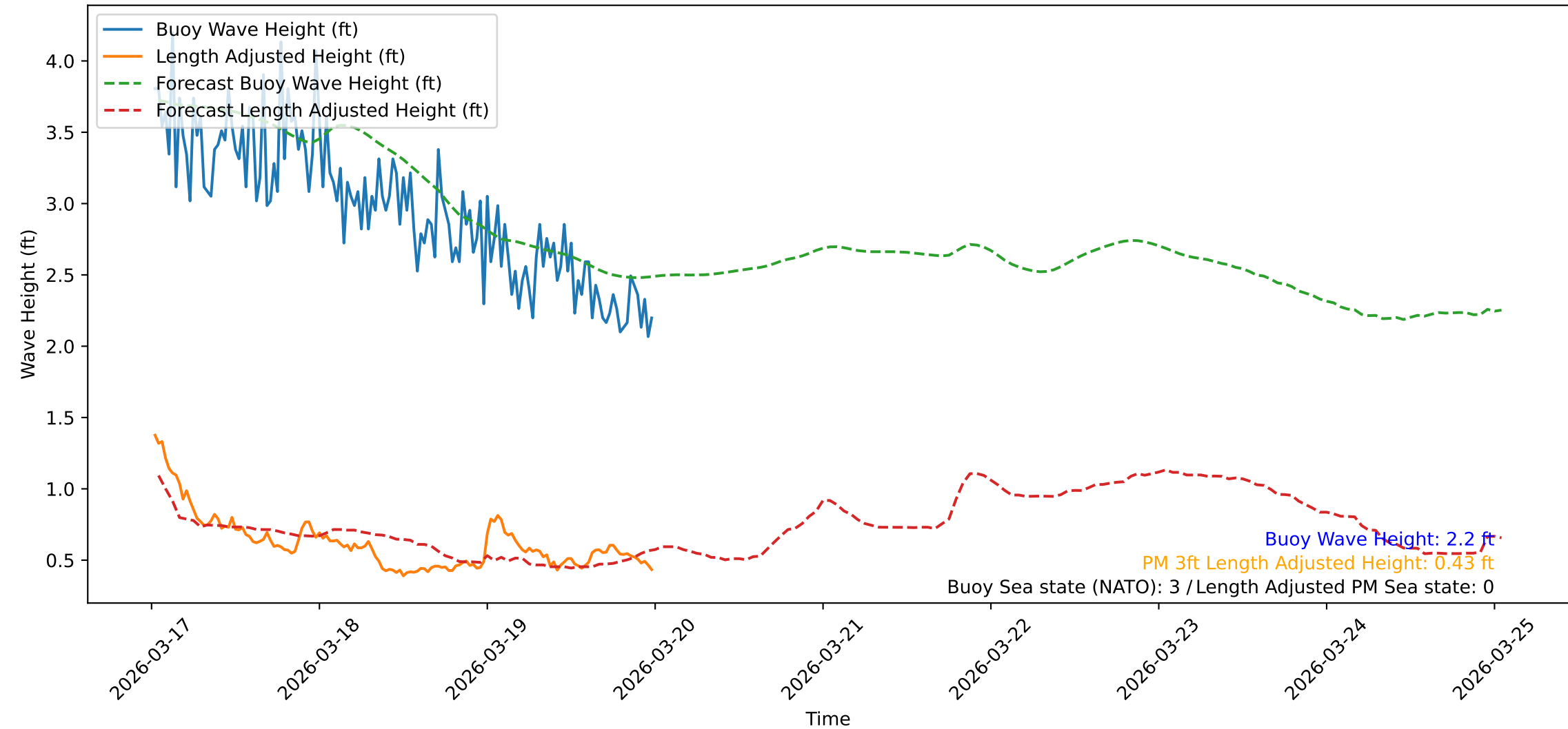
Wave Heights over Time for Green Beach at 2026-03-20 00:31:10
