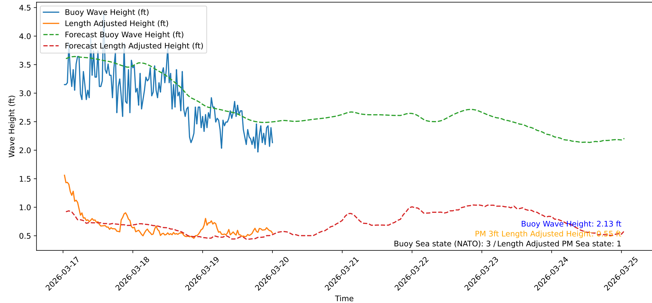
Wave Heights over Time for Oceanside Harbor at 2026-03-20 00:30:31
