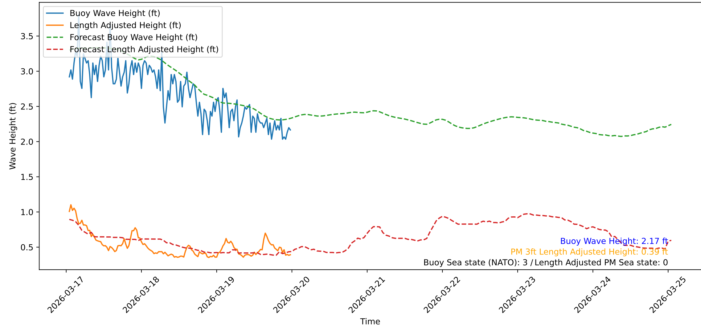
Wave Heights over Time for Red Beach at 2026-03-20 00:30:48
