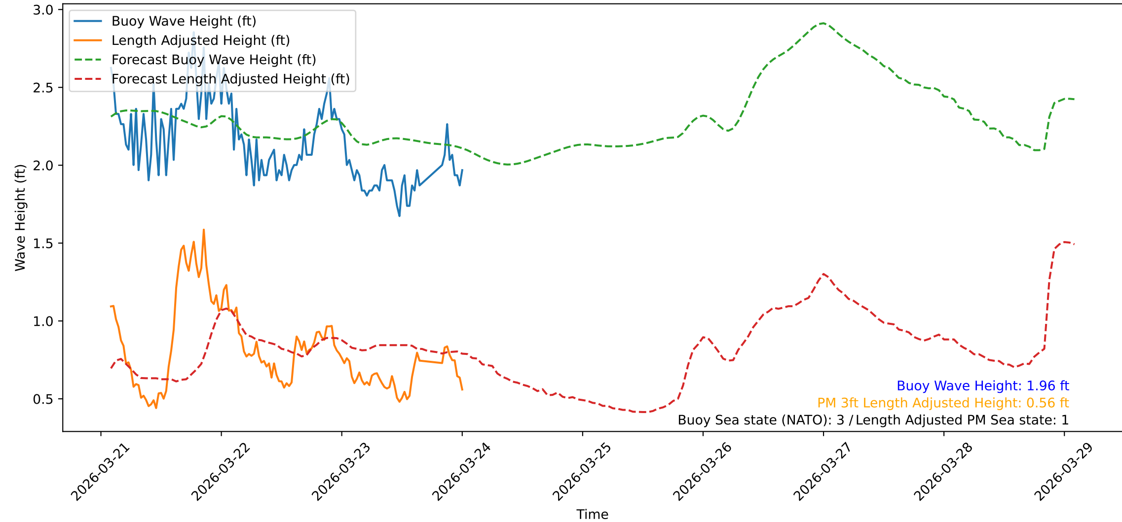
Wave Heights over Time for Red Beach at 2026-03-24 01:30:46
