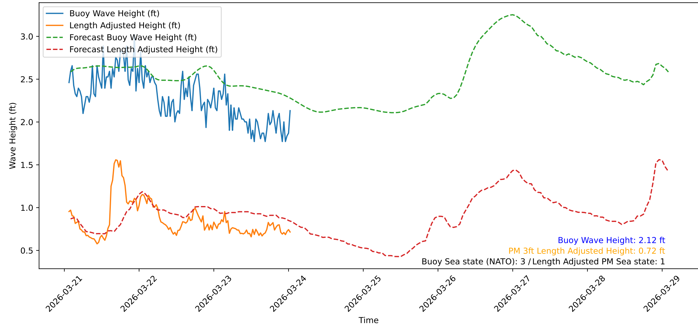
Wave Heights over Time for Oceanside Harbor at 2026-03-24 01:30:31
