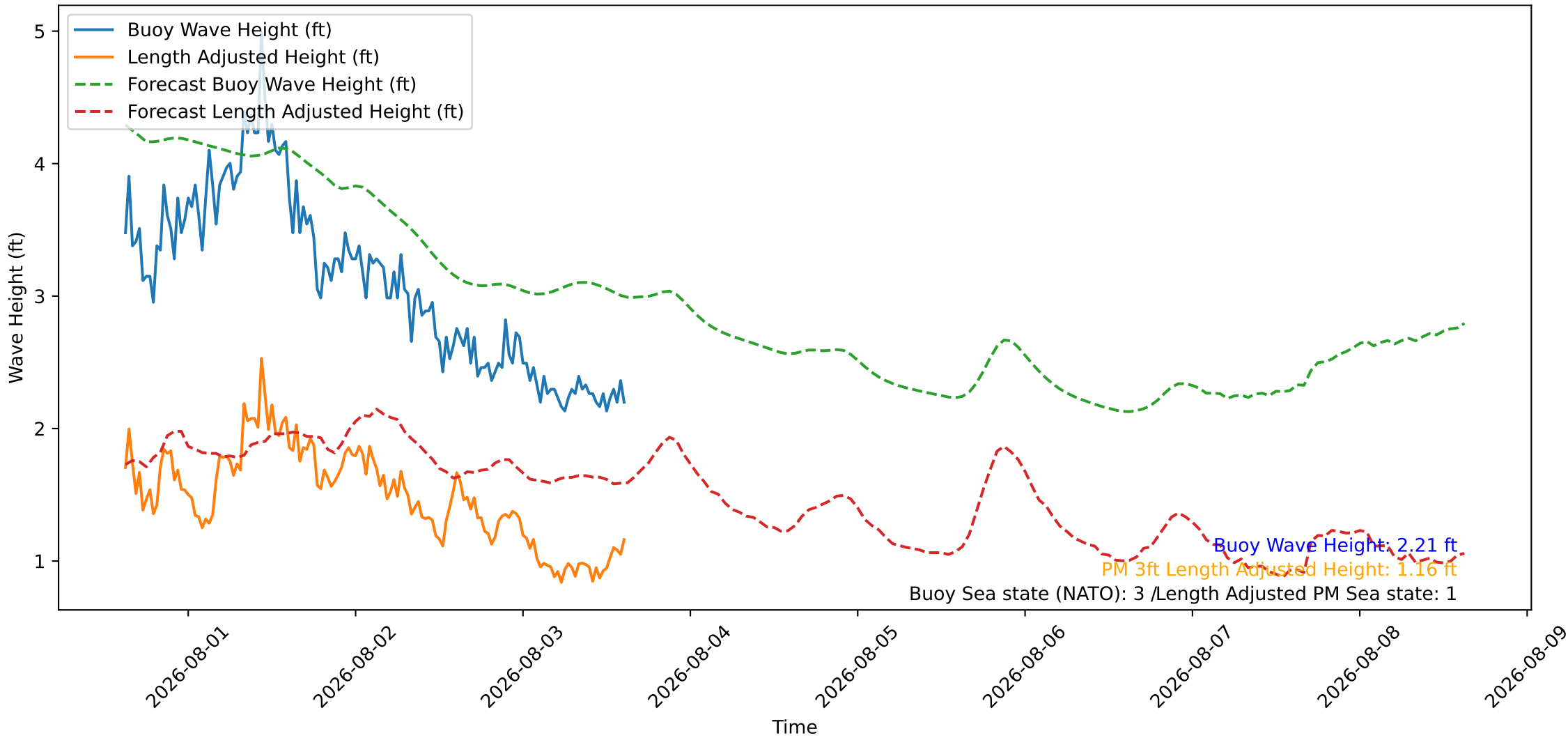
Wave Heights over Time for Green Beach at 2026-08-03 15:11:08
