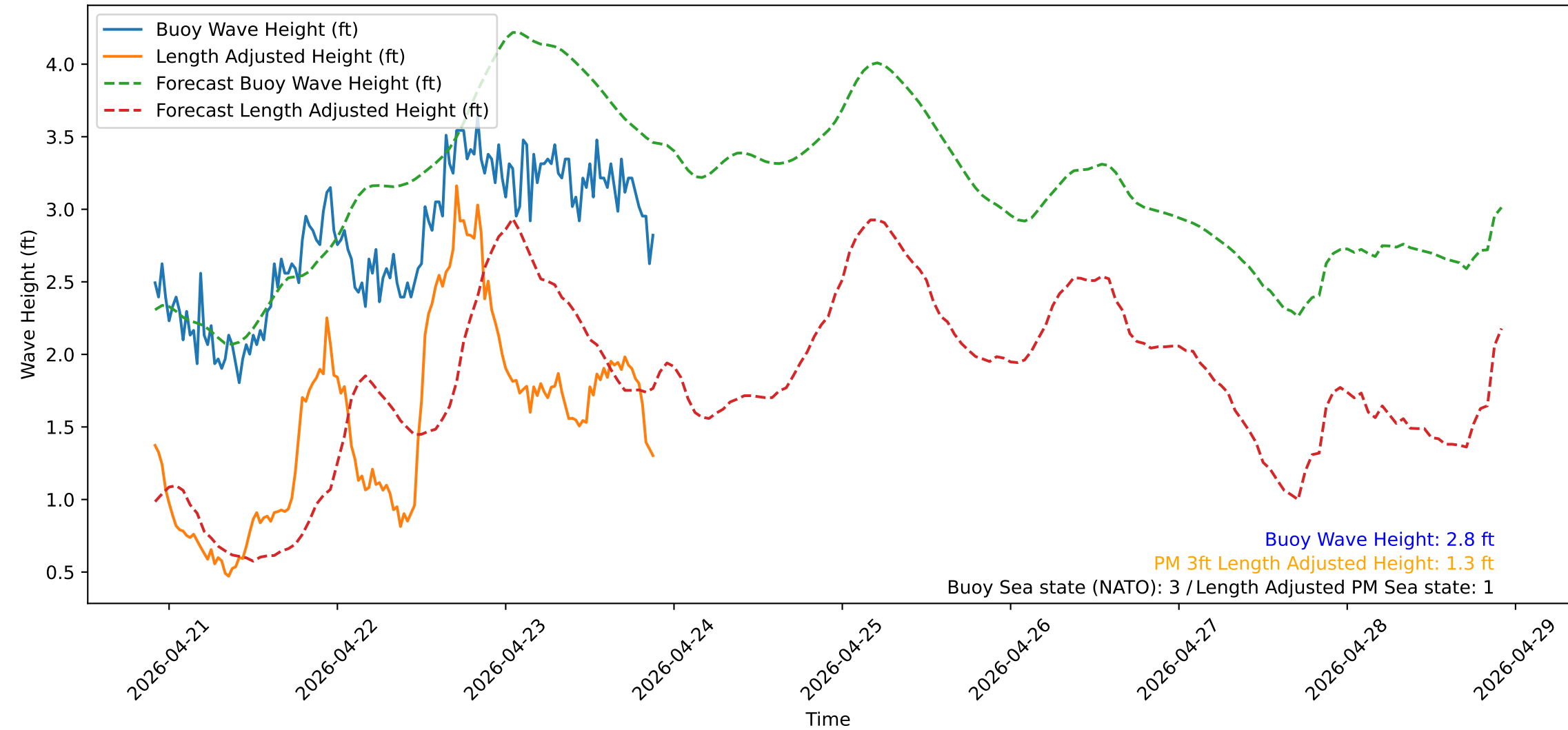
Wave Heights over Time for Red Beach at 2026-04-23 21:40:51
