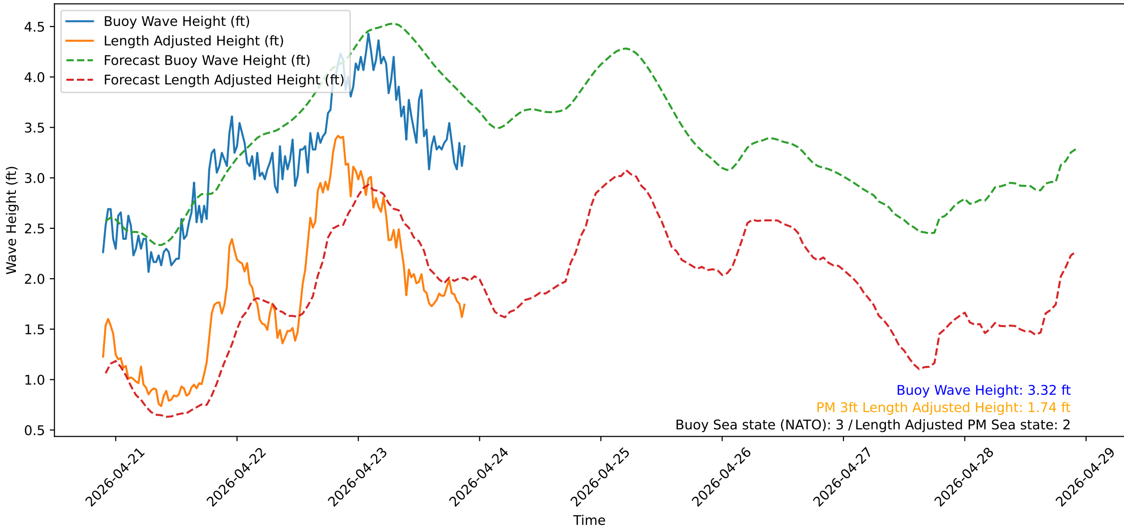
Wave Heights over Time for Oceanside Harbor at 2026-04-23 21:40:31
