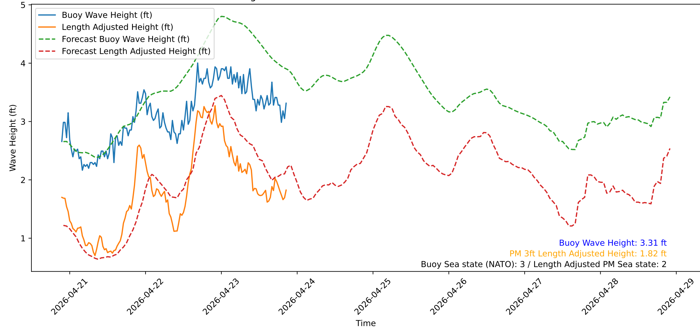
Wave Heights over Time for Green Beach at 2026-04-23 21:41:13
