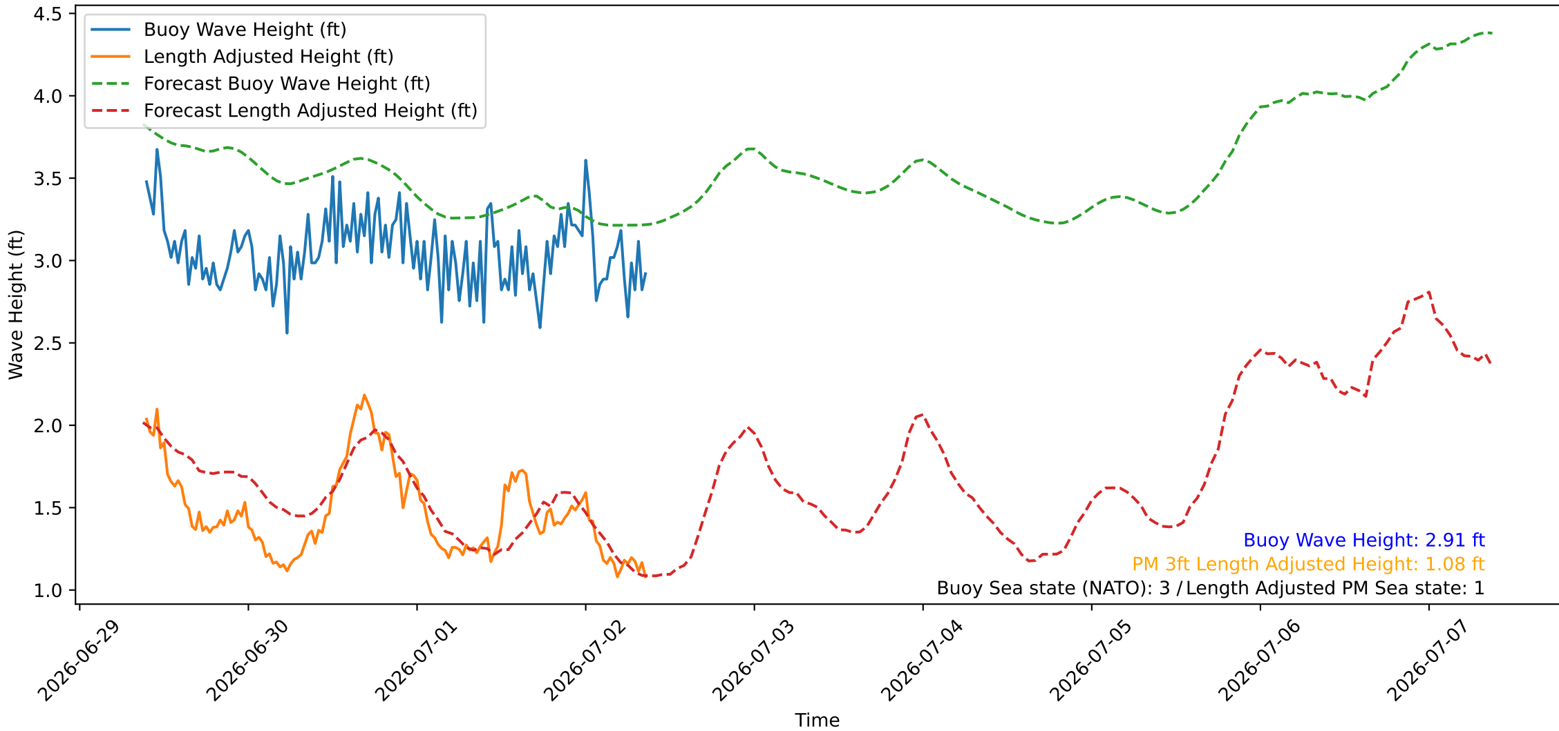
Wave Heights over Time for Oceanside Harbor at 2026-07-02 09:20:26
