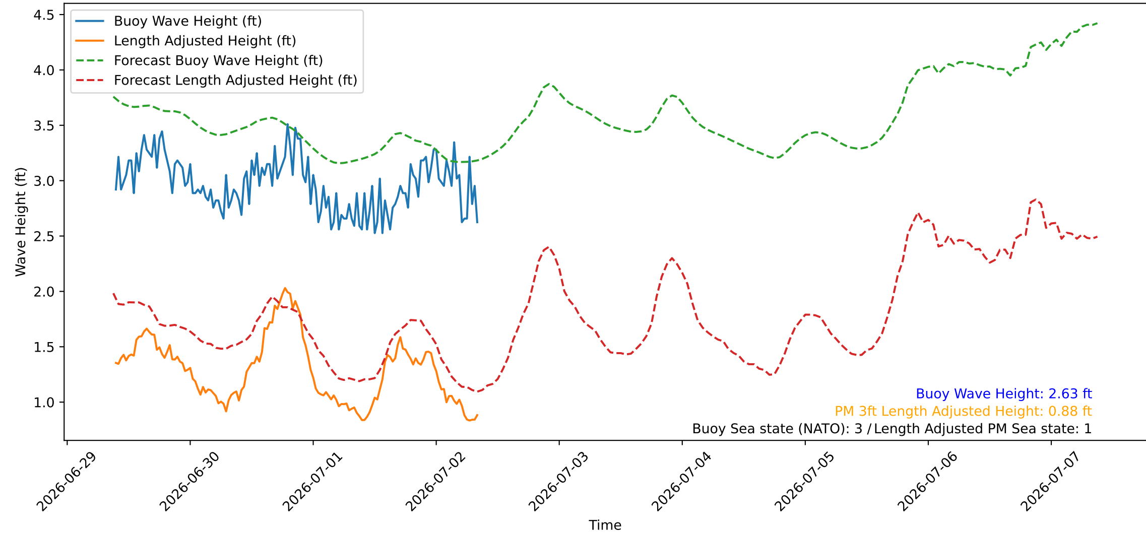
Wave Heights over Time for Green Beach at 2026-07-02 09:21:09
