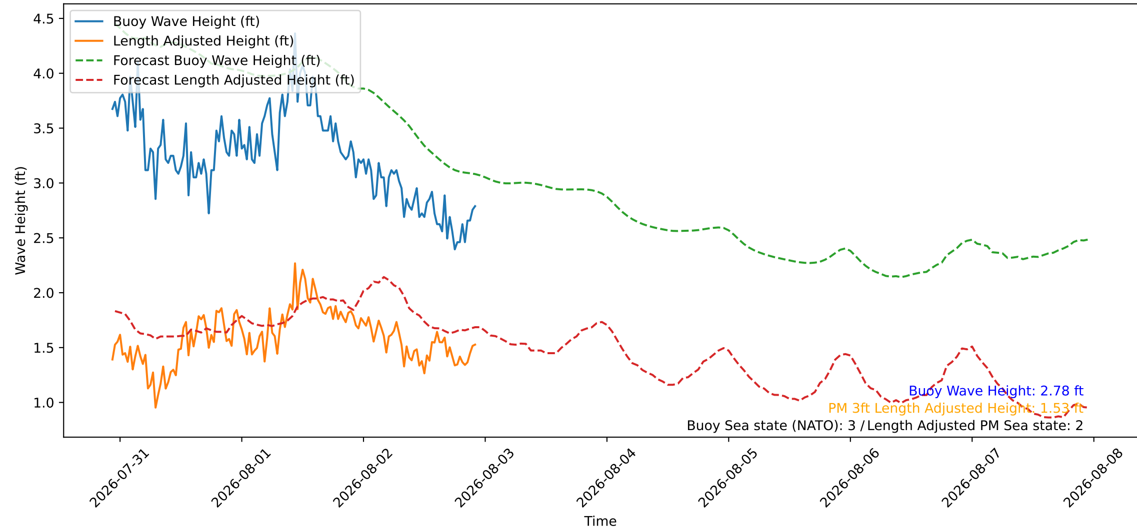
Wave Heights over Time for Oceanside Harbor at 2026-08-02 22:40:26
