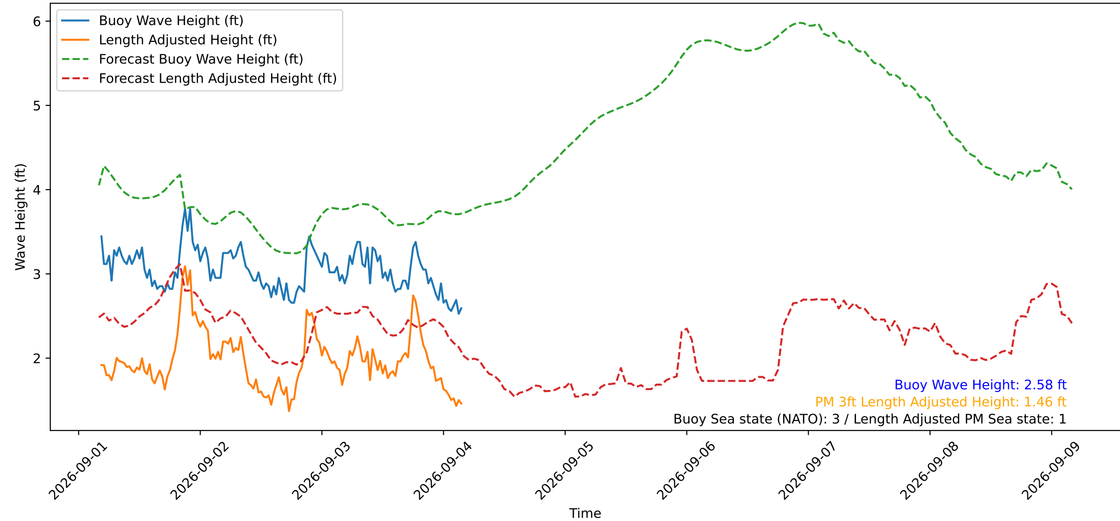
Wave Heights over Time for Green Beach at 2026-09-04 04:11:13
