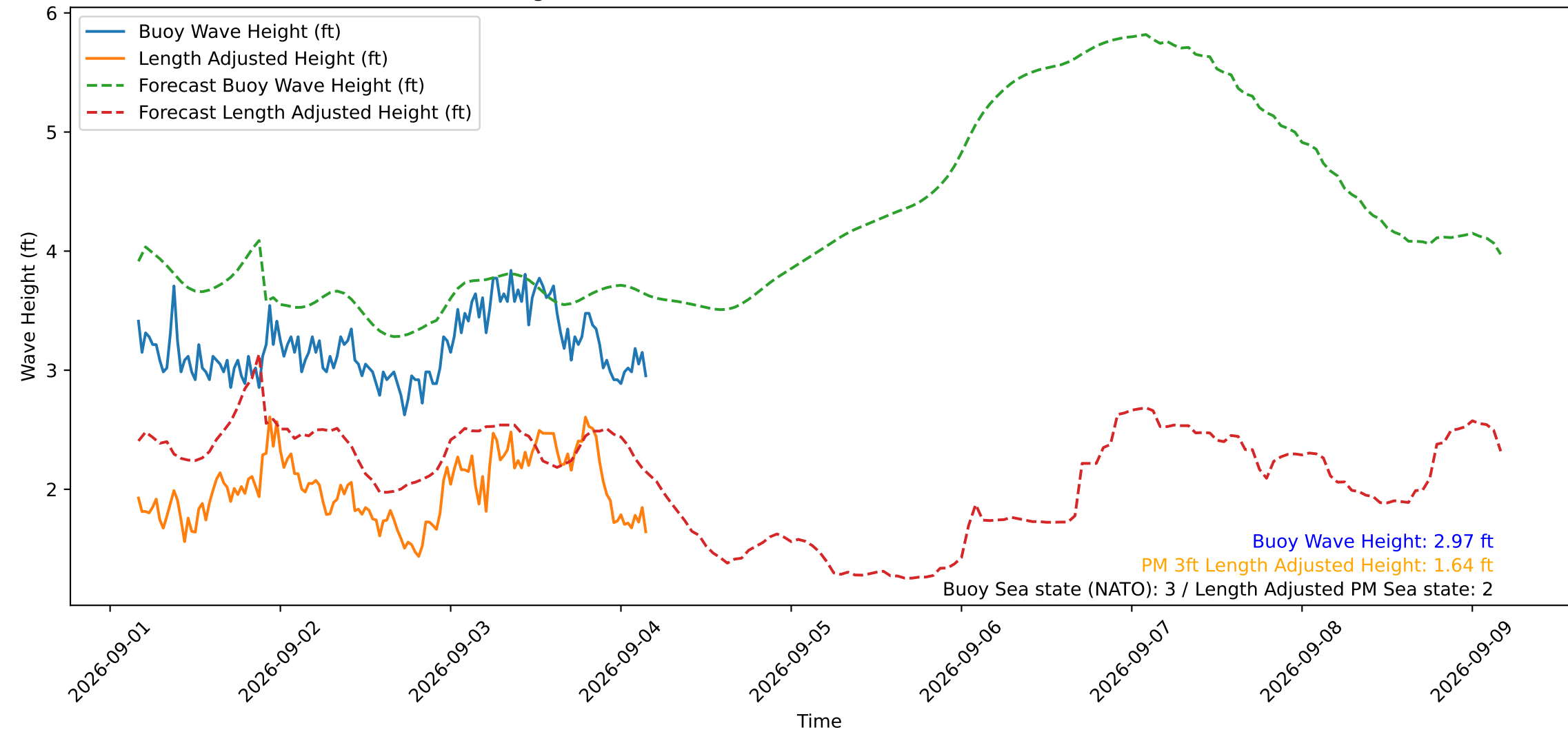
Wave Heights over Time for Oceanside Harbor at 2026-09-04 04:10:30
