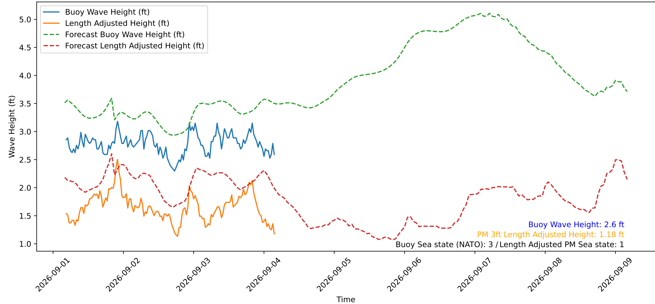
Wave Heights over Time for Red Beach at 2026-09-04 04:10:50
