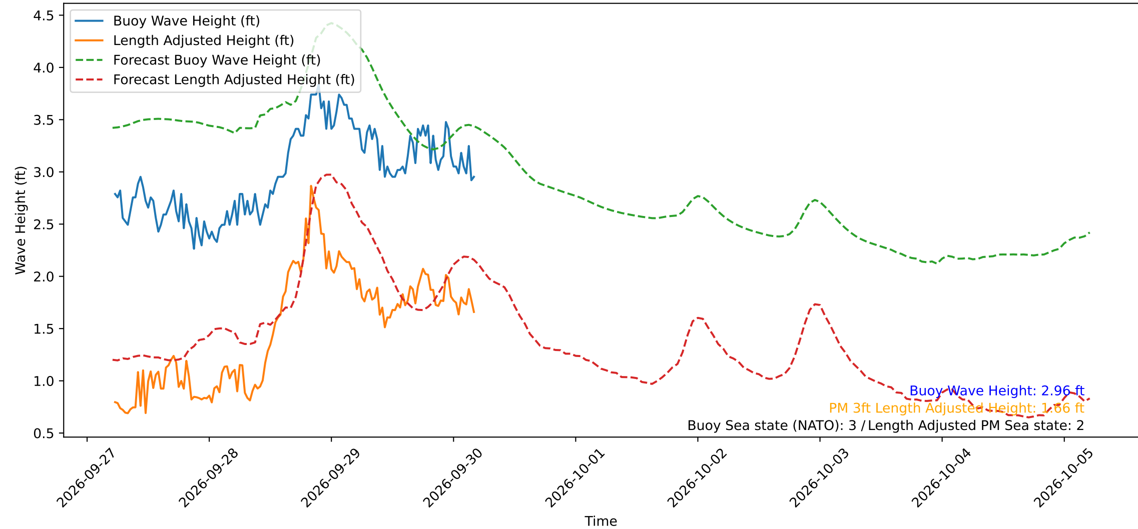
Wave Heights over Time for Red Beach at 2026-09-30 05:10:51
