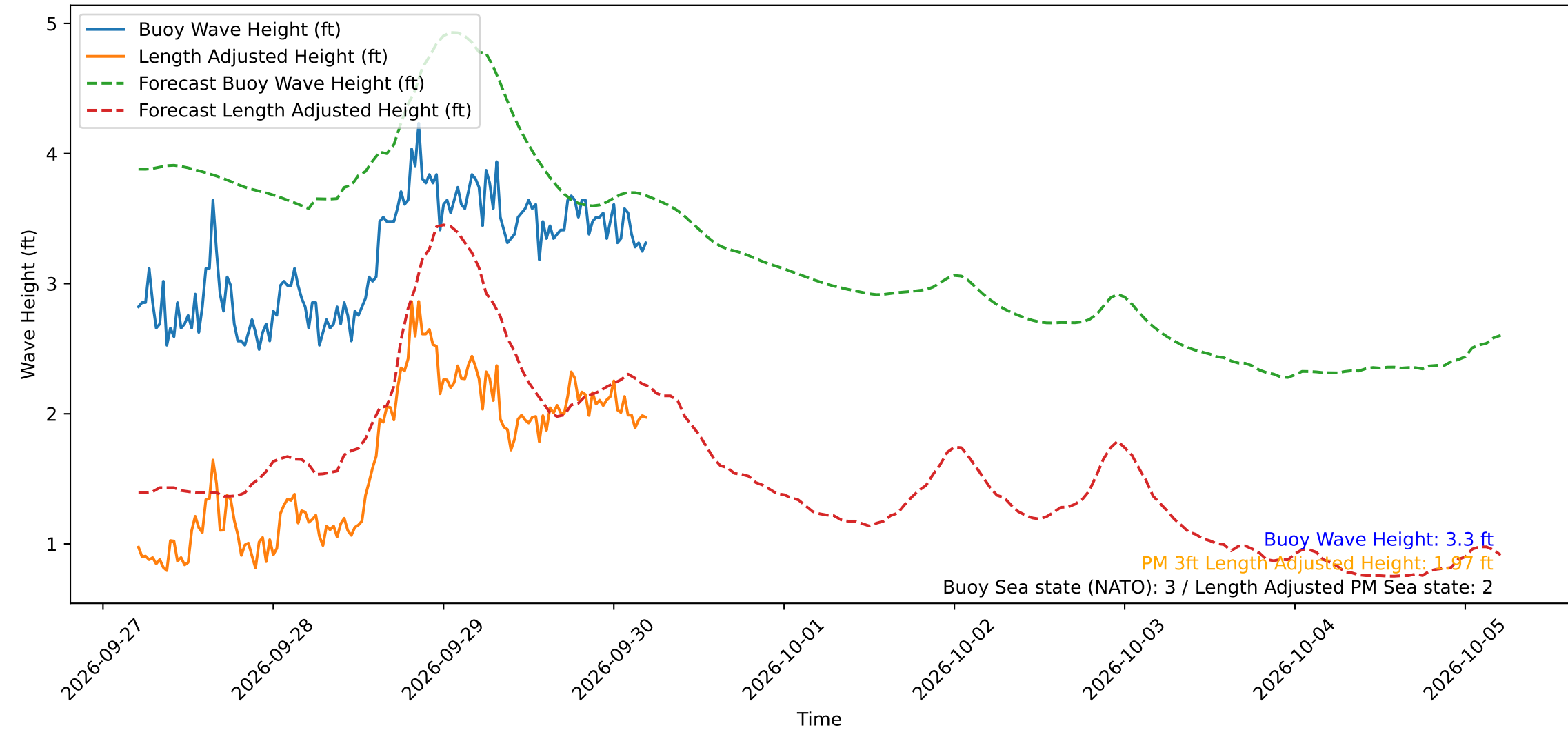
Wave Heights over Time for Oceanside Harbor at 2026-09-30 05:10:31
