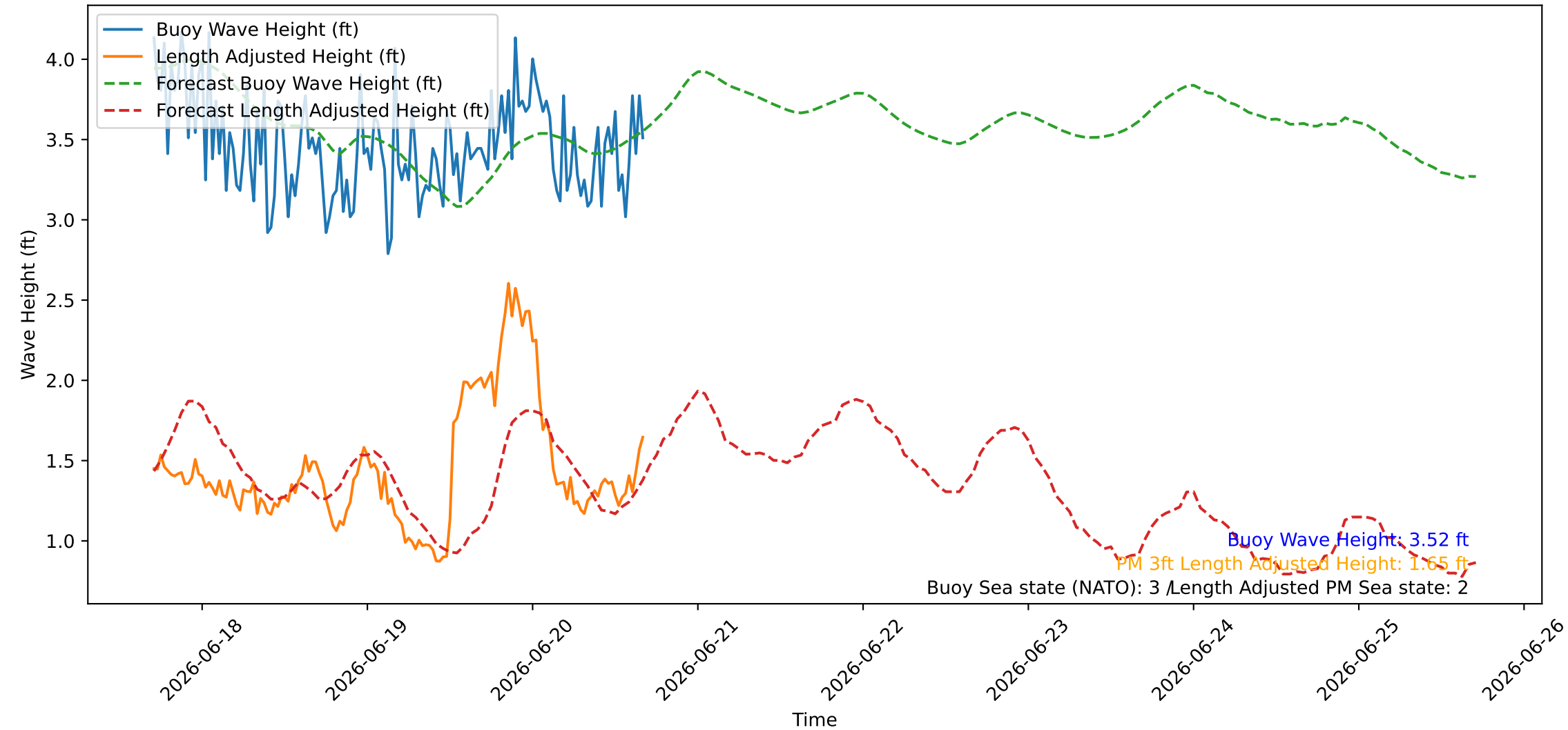
Wave Heights over Time for Oceanside Harbor at 2026-06-20 16:50:26
