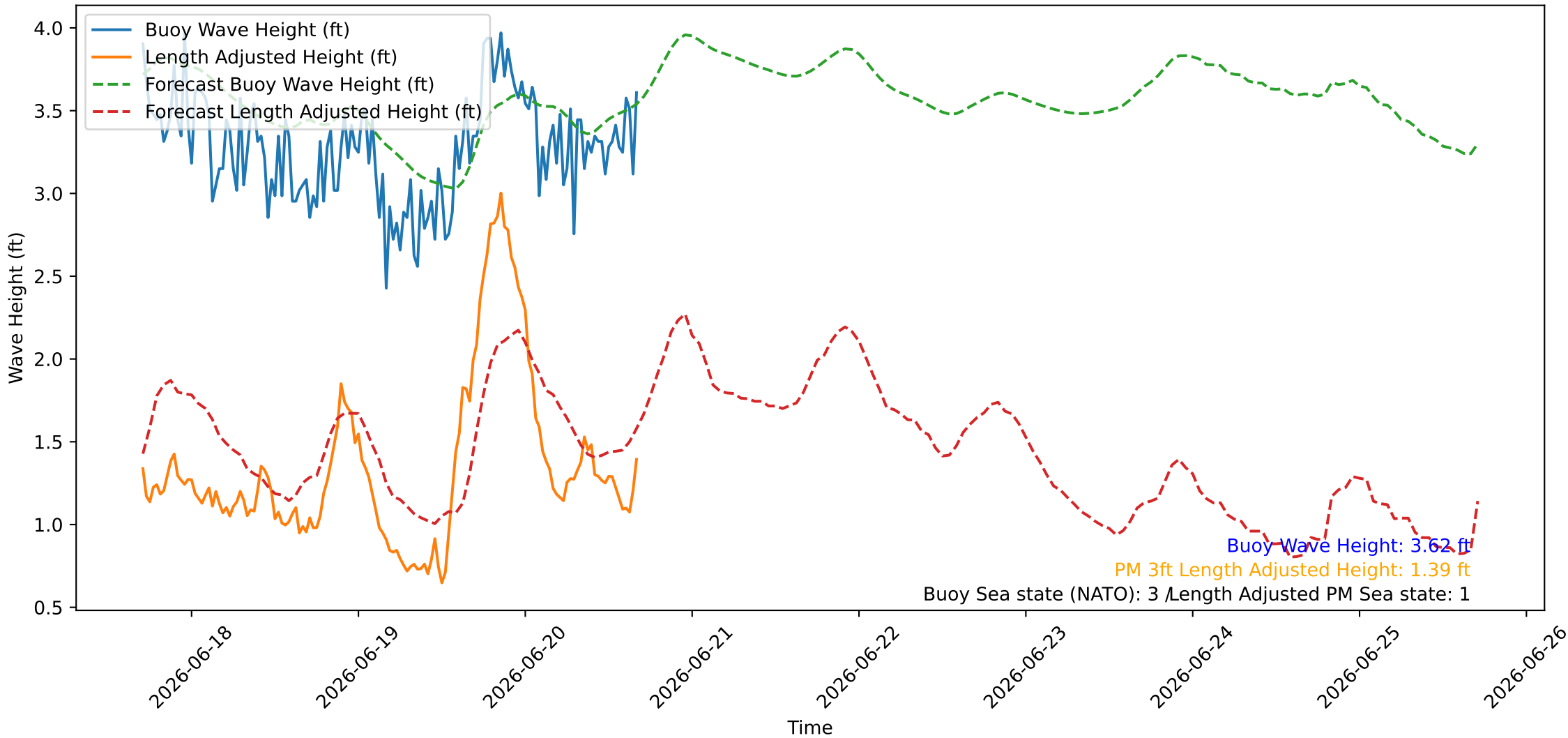
Wave Heights over Time for Green Beach at 2026-06-20 16:51:09
