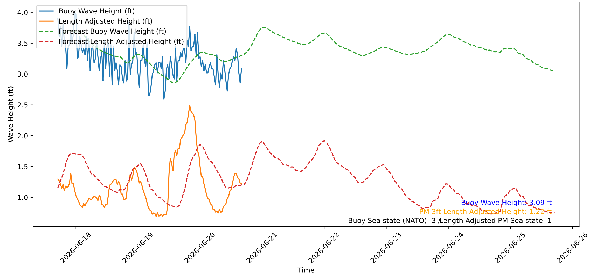
Wave Heights over Time for Red Beach at 2026-06-20 16:50:47
