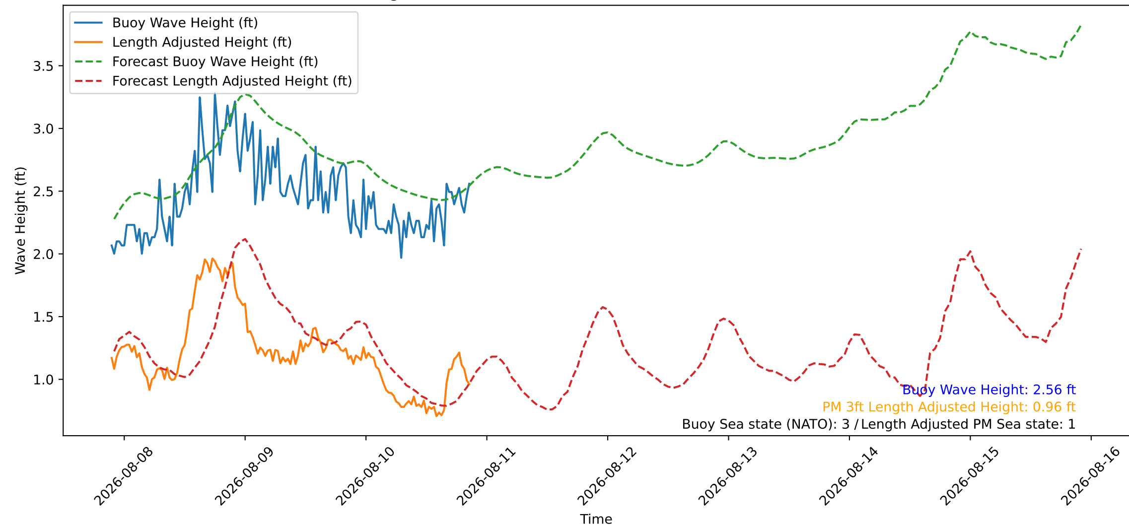
Wave Heights over Time for Oceanside Harbor at 2026-08-10 21:30:27
