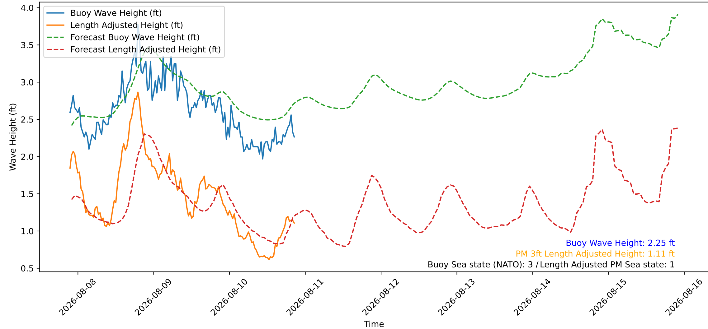
Wave Heights over Time for Green Beach at 2026-08-10 21:31:09
