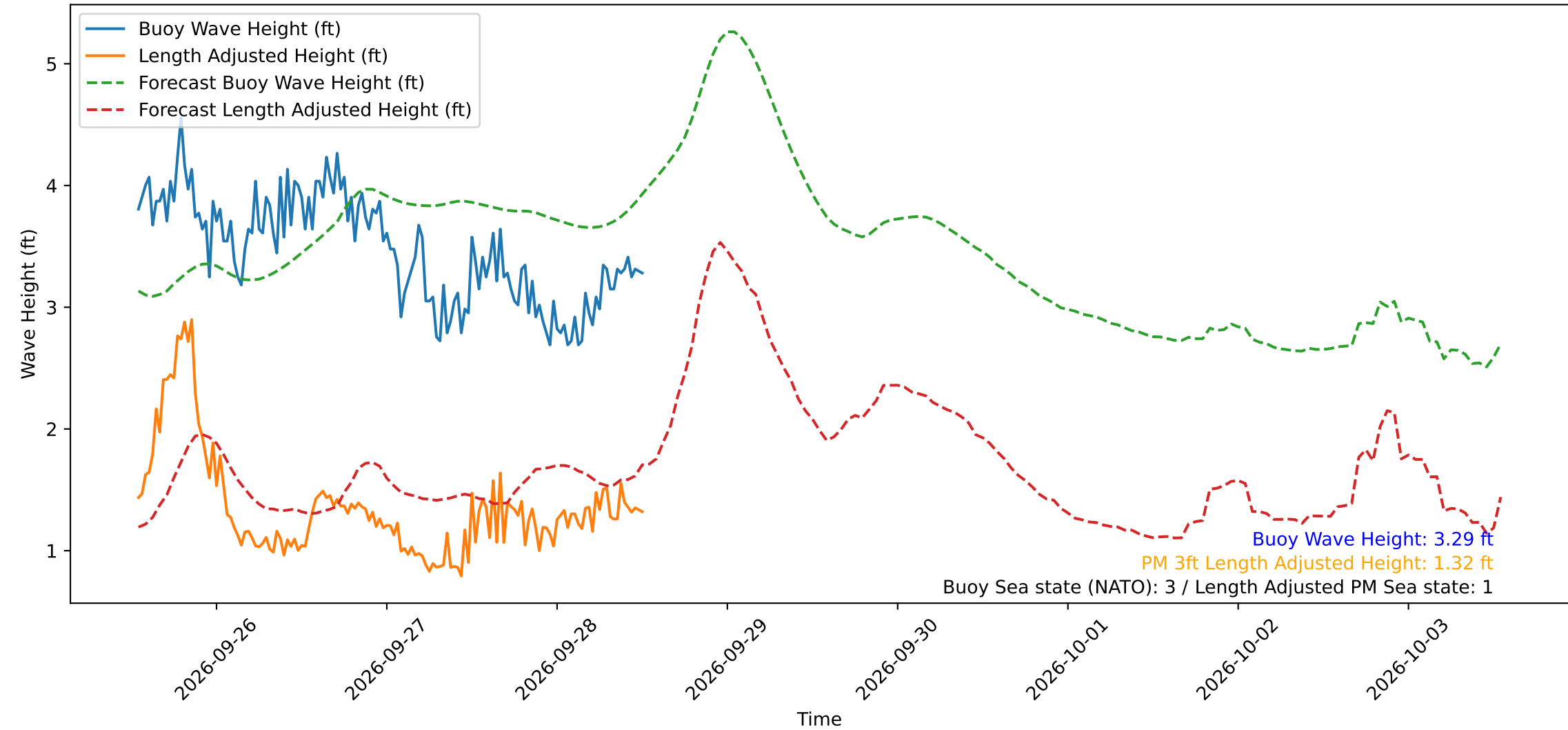
Wave Heights over Time for Green Beach at 2026-09-28 12:51:15
