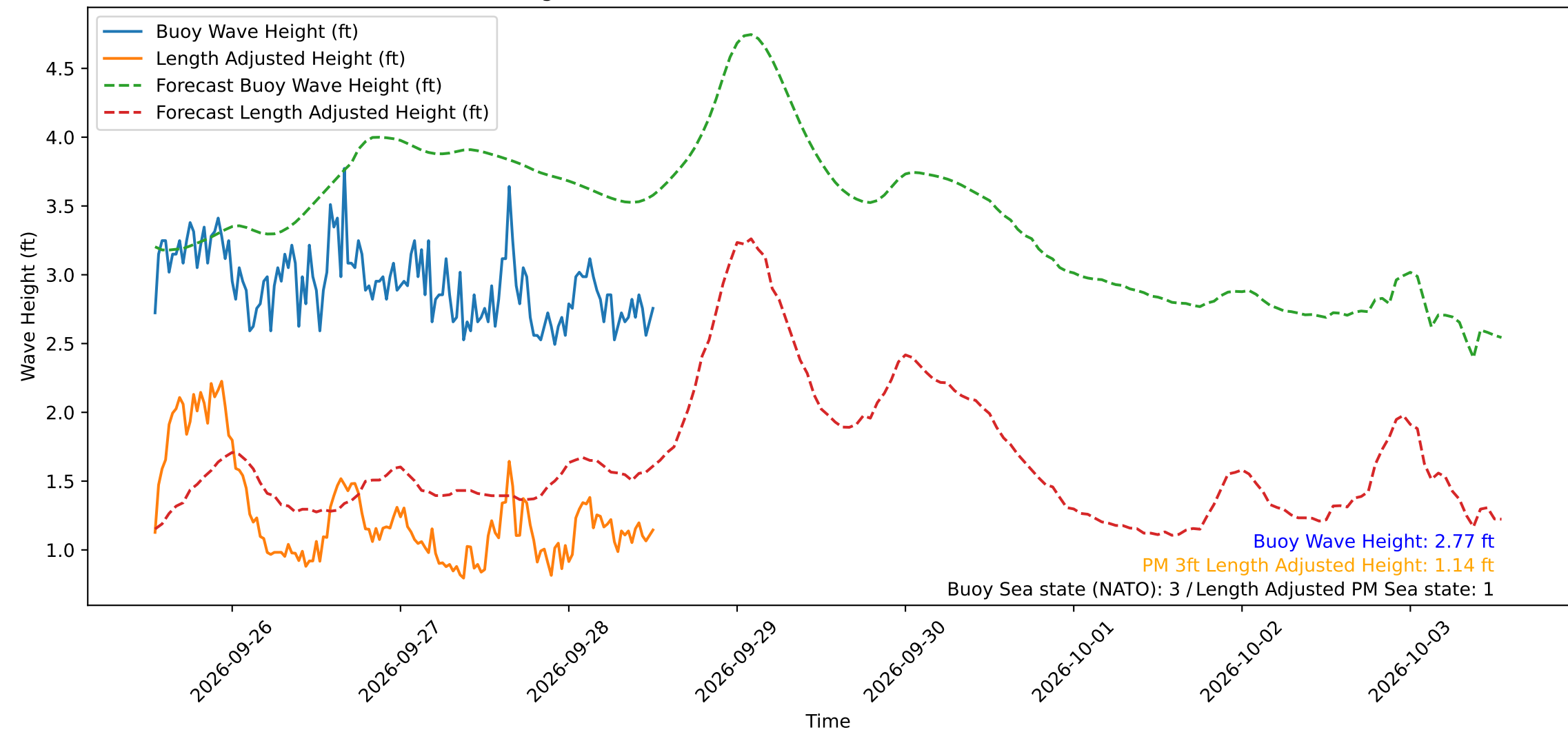
Wave Heights over Time for Oceanside Harbor at 2026-09-28 12:50:30
