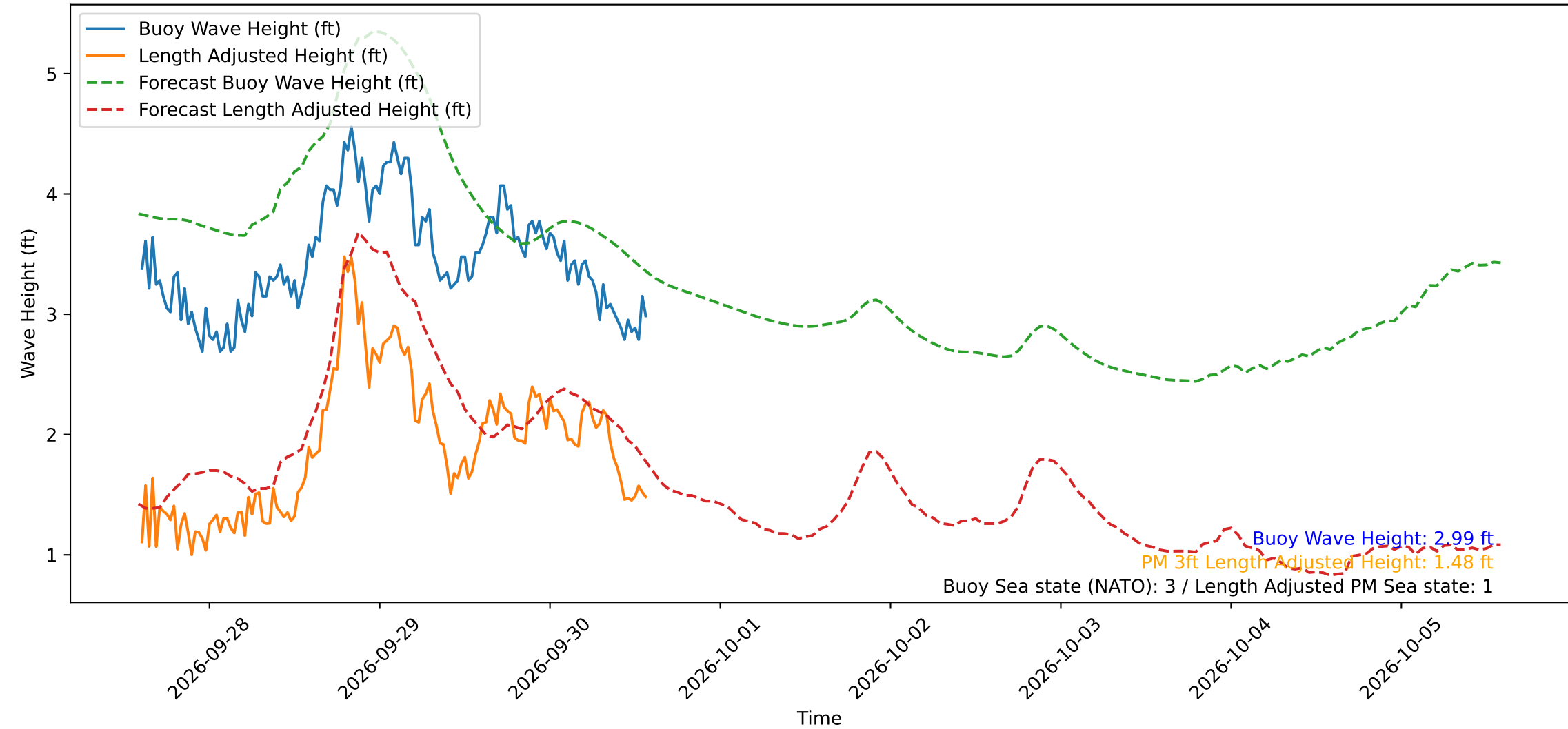
Wave Heights over Time for Green Beach at 2026-09-30 14:21:14
