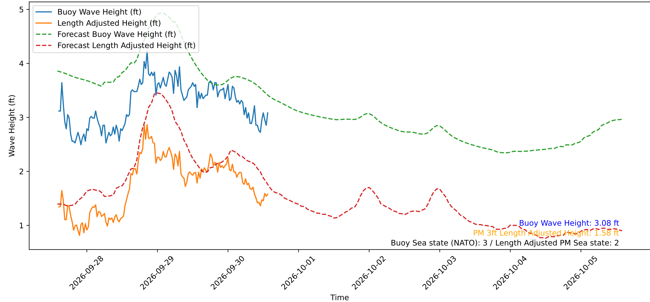
Wave Heights over Time for Oceanside Harbor at 2026-09-30 14:20:30
