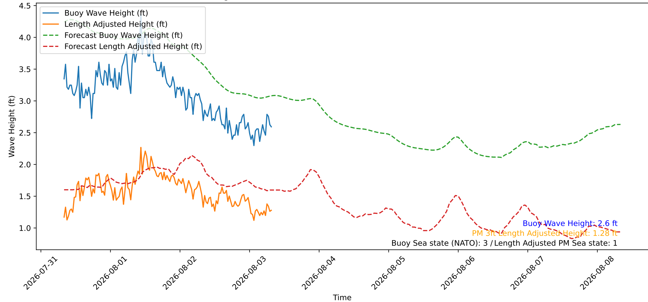
Wave Heights over Time for Oceanside Harbor at 2026-08-03 08:00:26
