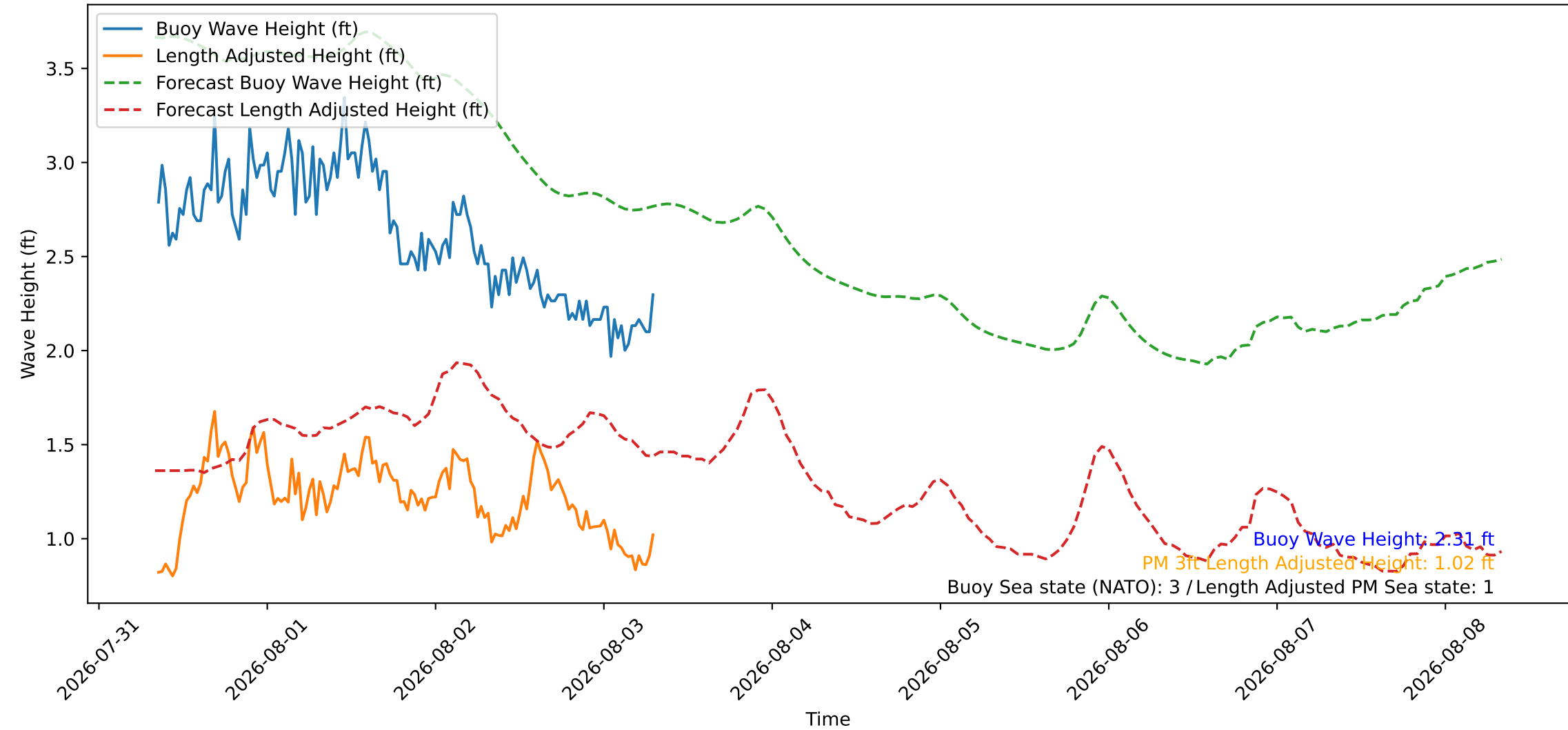
Wave Heights over Time for Red Beach at 2026-08-03 08:00:45
