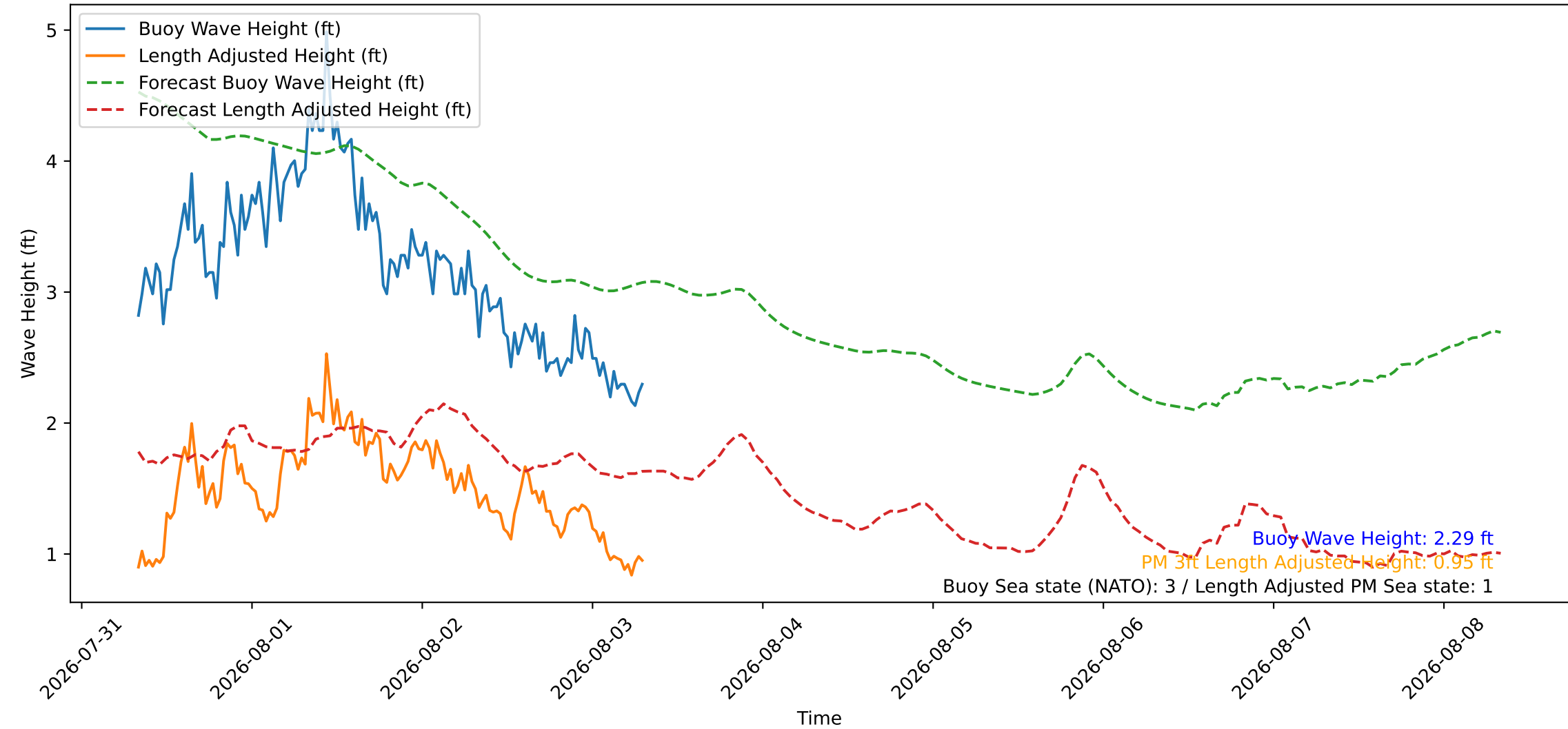
Wave Heights over Time for Green Beach at 2026-08-03 08:01:08
