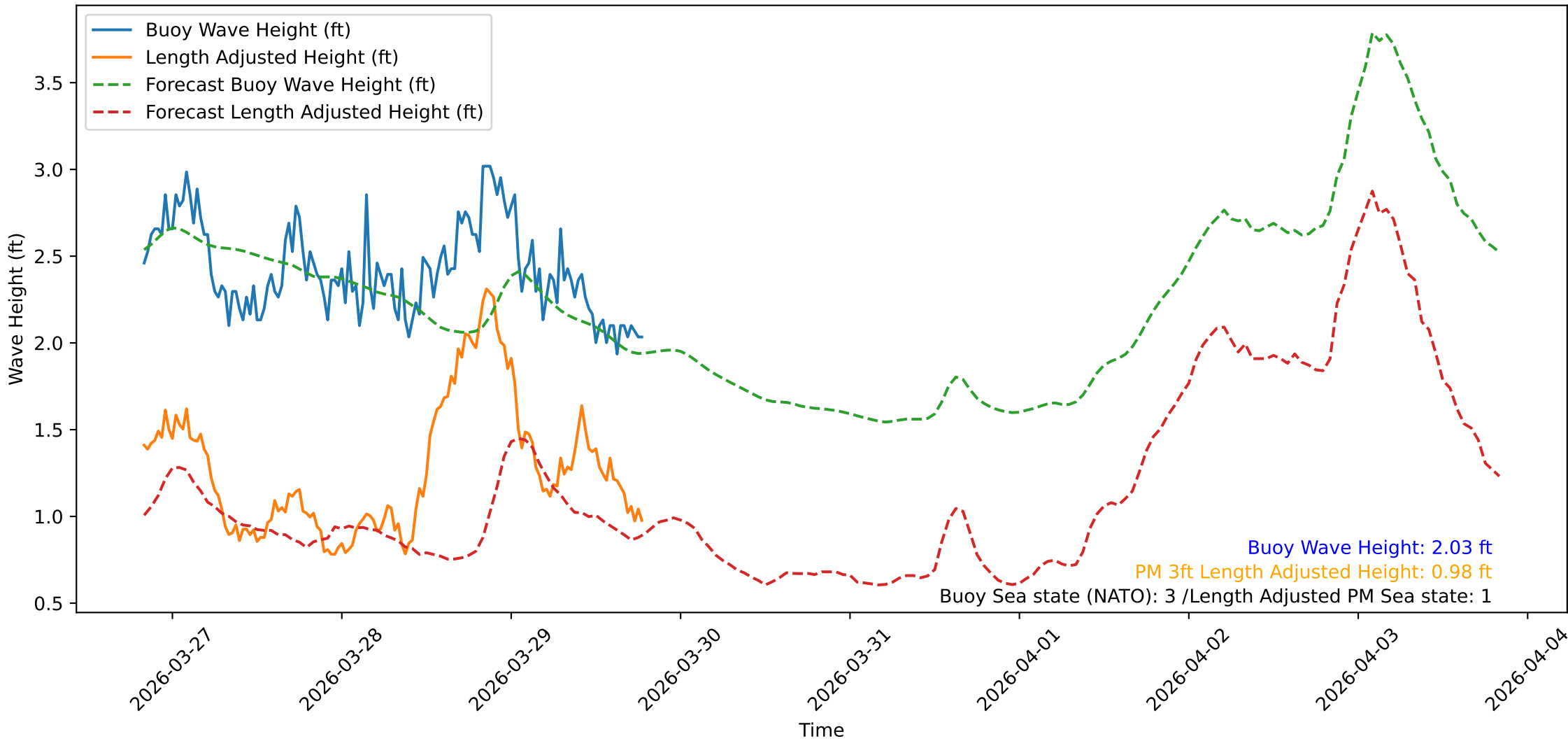
Wave Heights over Time for Red Beach at 2026-03-29 19:30:47
