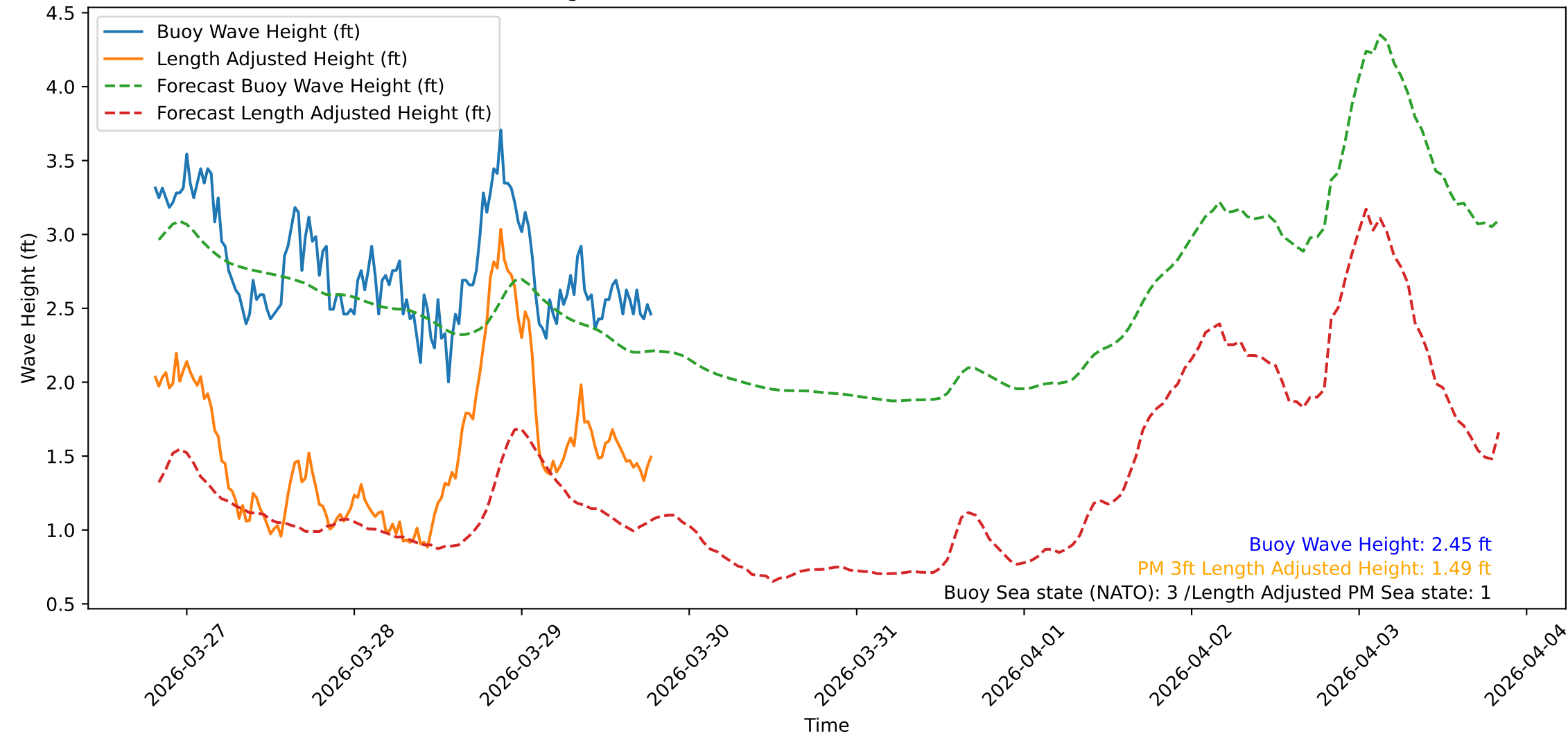
Wave Heights over Time for Green Beach at 2026-03-29 19:31:11
