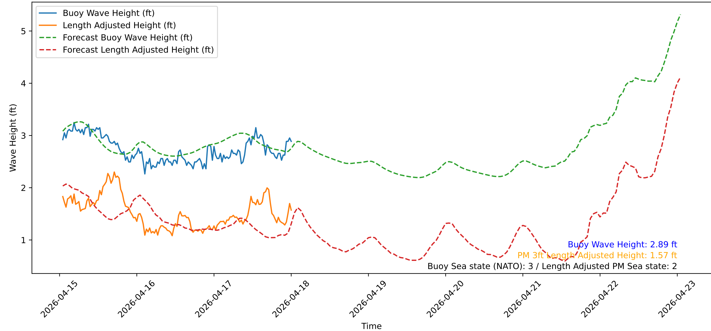
Wave Heights over Time for Red Beach at 2026-04-18 00:50:52
