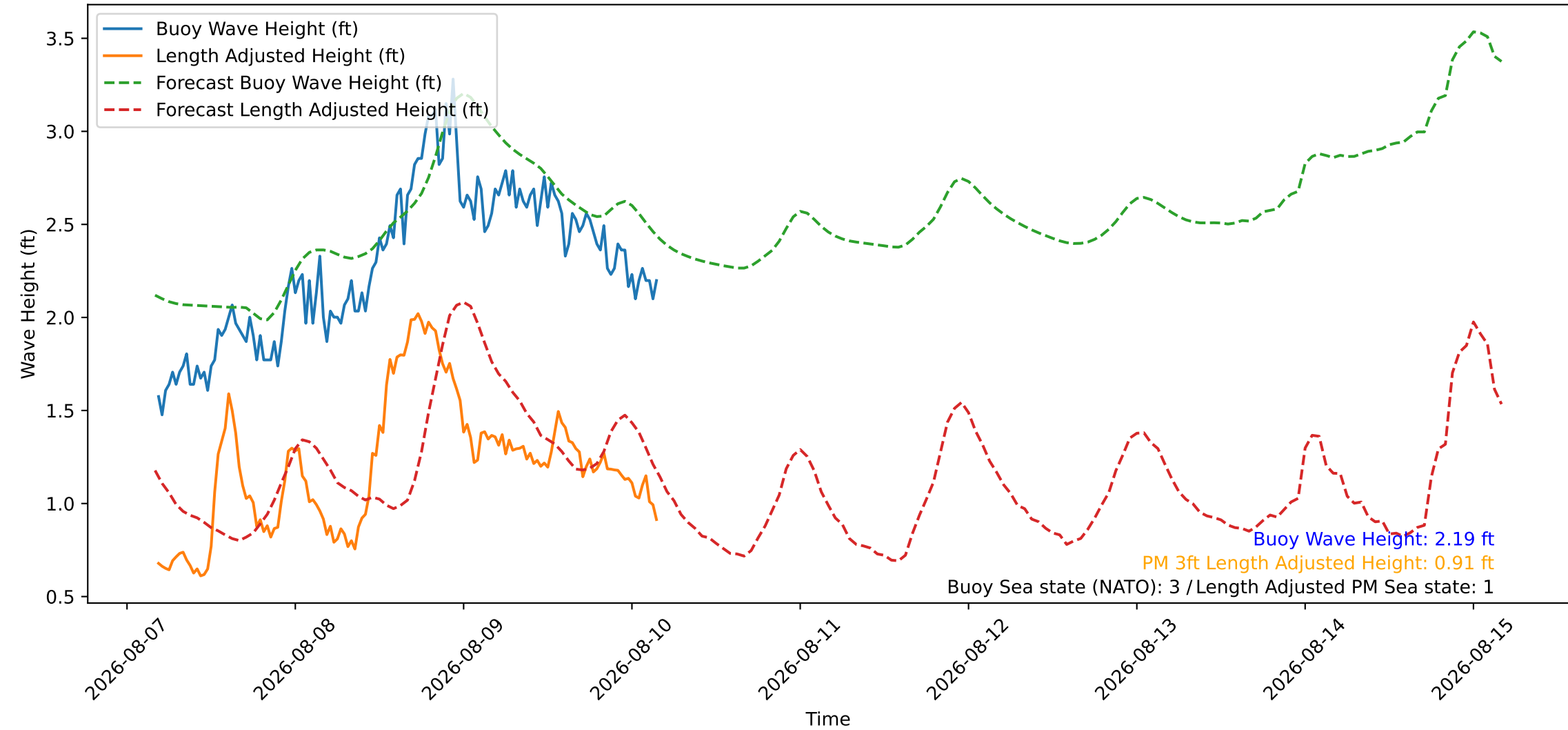
Wave Heights over Time for Red Beach at 2026-08-10 04:10:46
