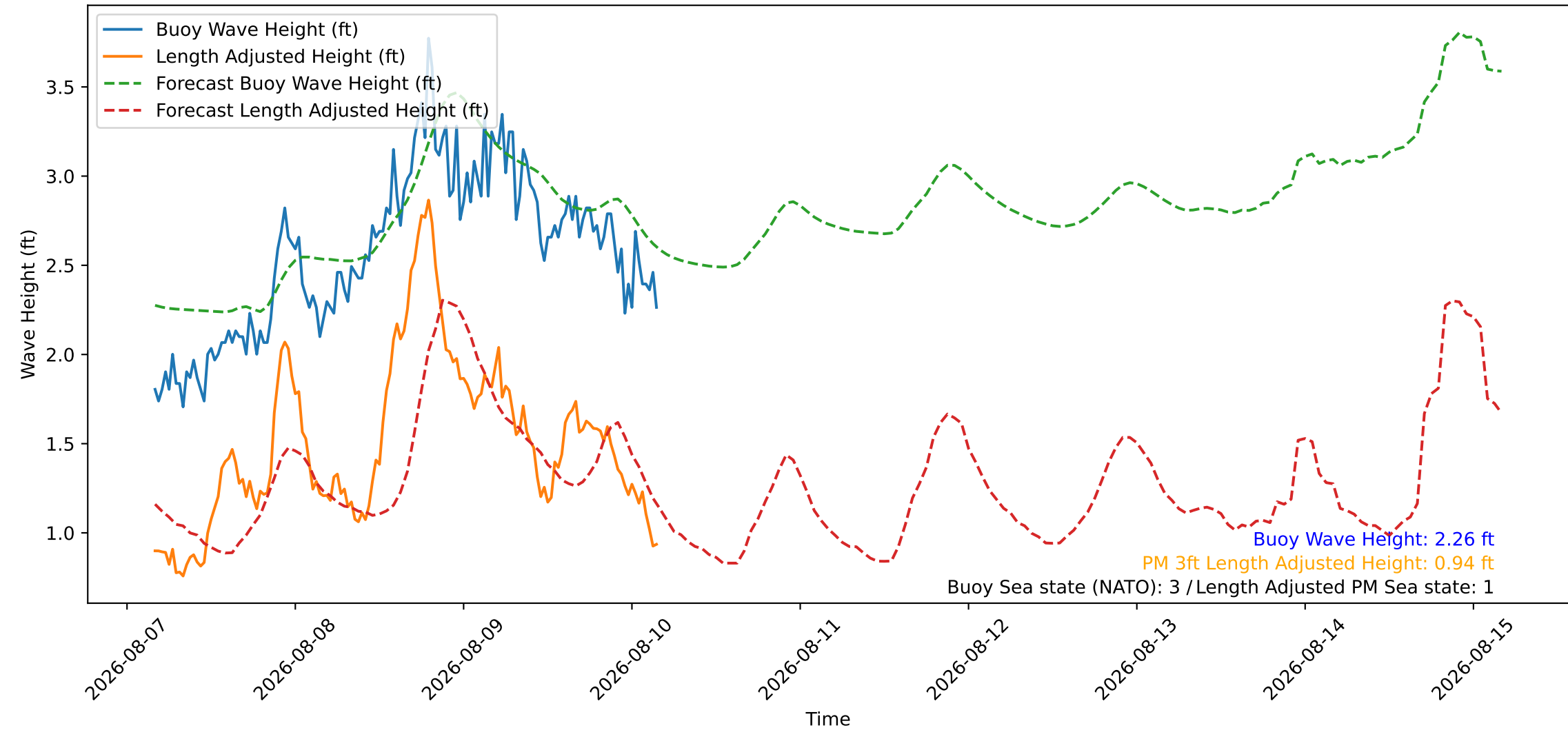
Wave Heights over Time for Green Beach at 2026-08-10 04:11:09
