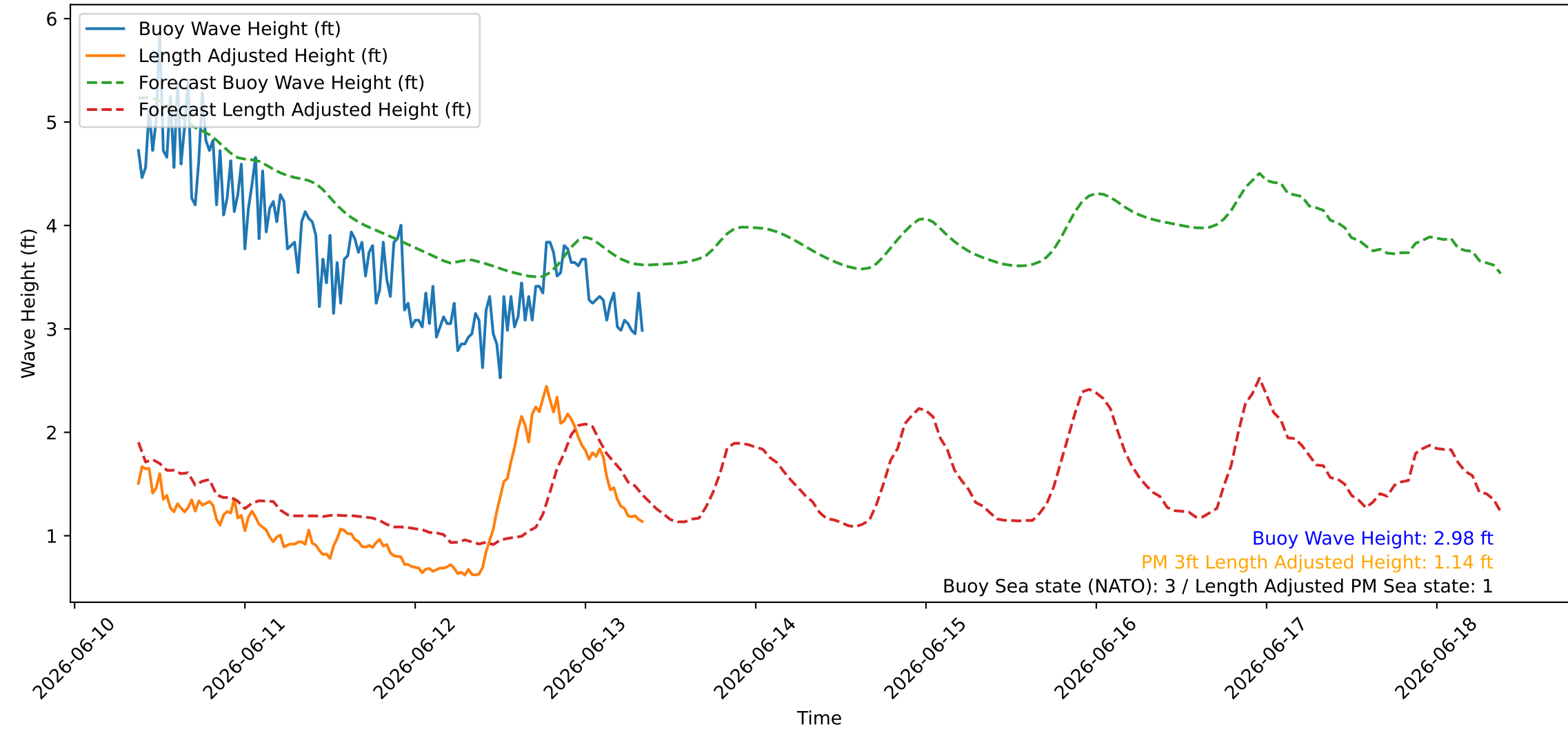
Wave Heights over Time for Red Beach at 2026-06-13 08:40:46
