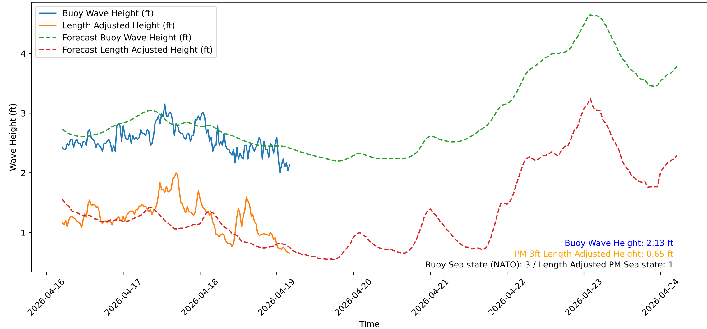
Wave Heights over Time for Red Beach at 2026-04-19 04:40:50
