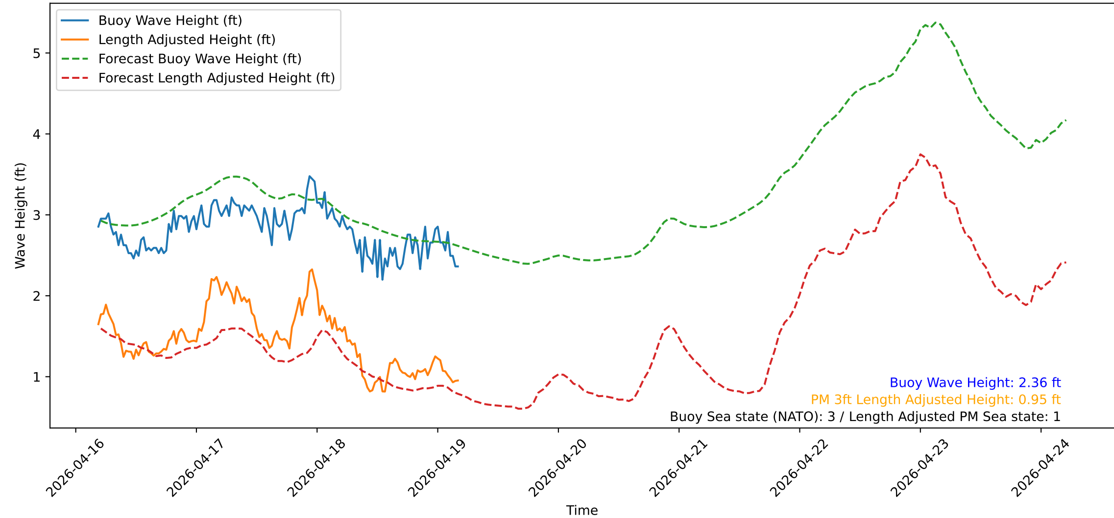
Wave Heights over Time for Green Beach at 2026-04-19 04:41:13
