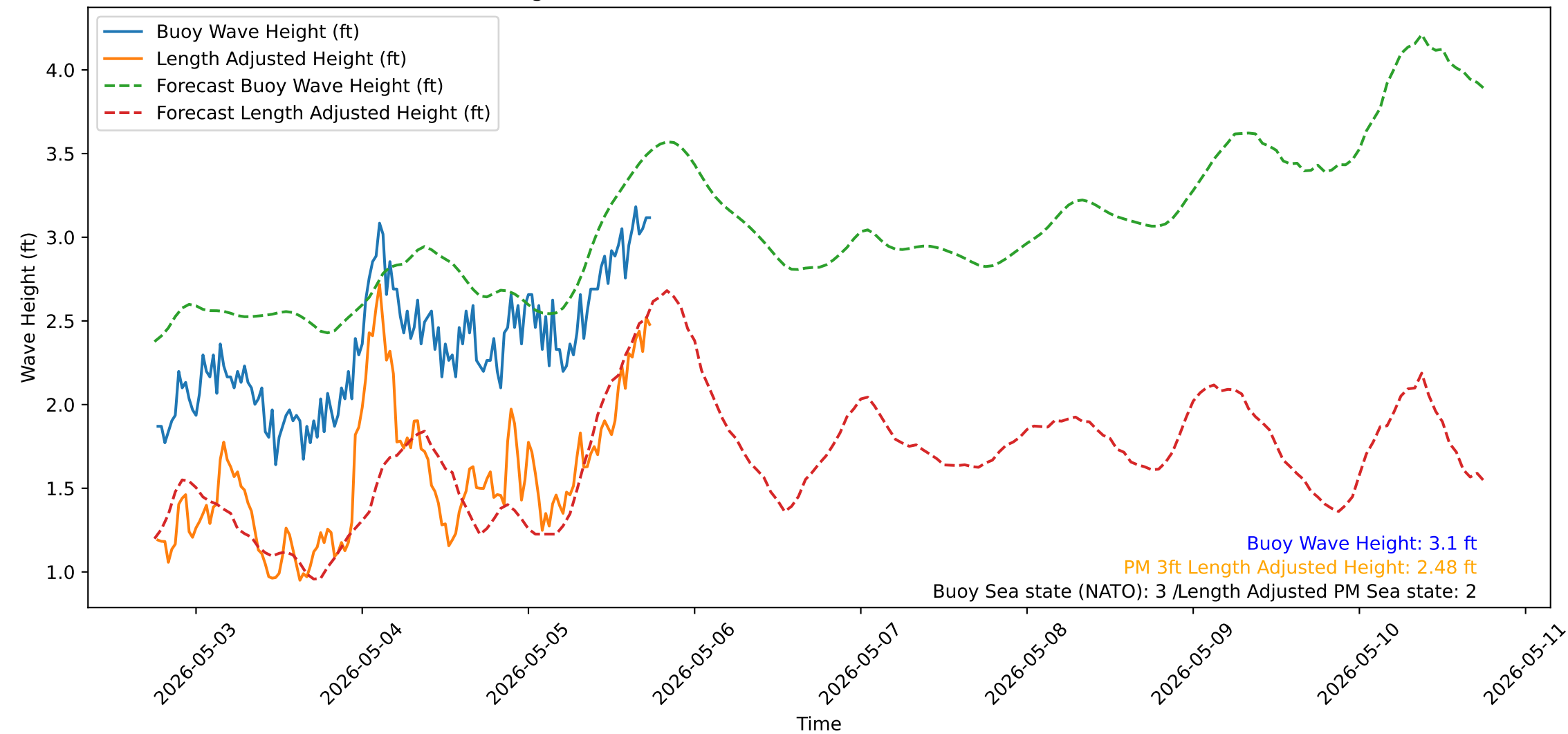
Wave Heights over Time for Oceanside Harbor at 2026-05-05 18:20:31
