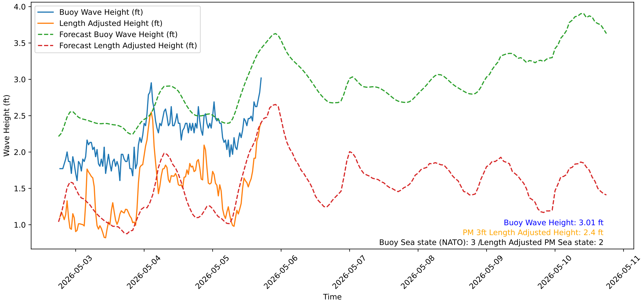
Wave Heights over Time for Red Beach at 2026-05-05 18:20:51
