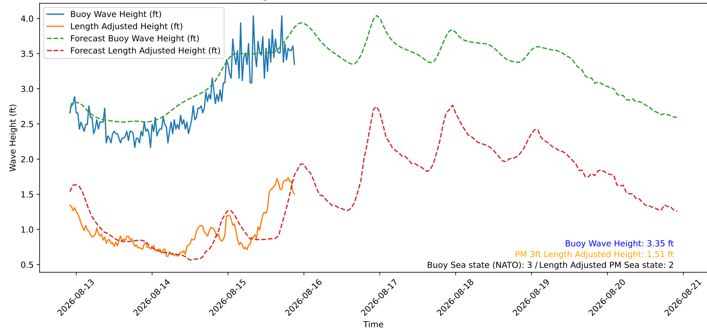
Wave Heights over Time for Red Beach at 2026-08-15 21:40:46
