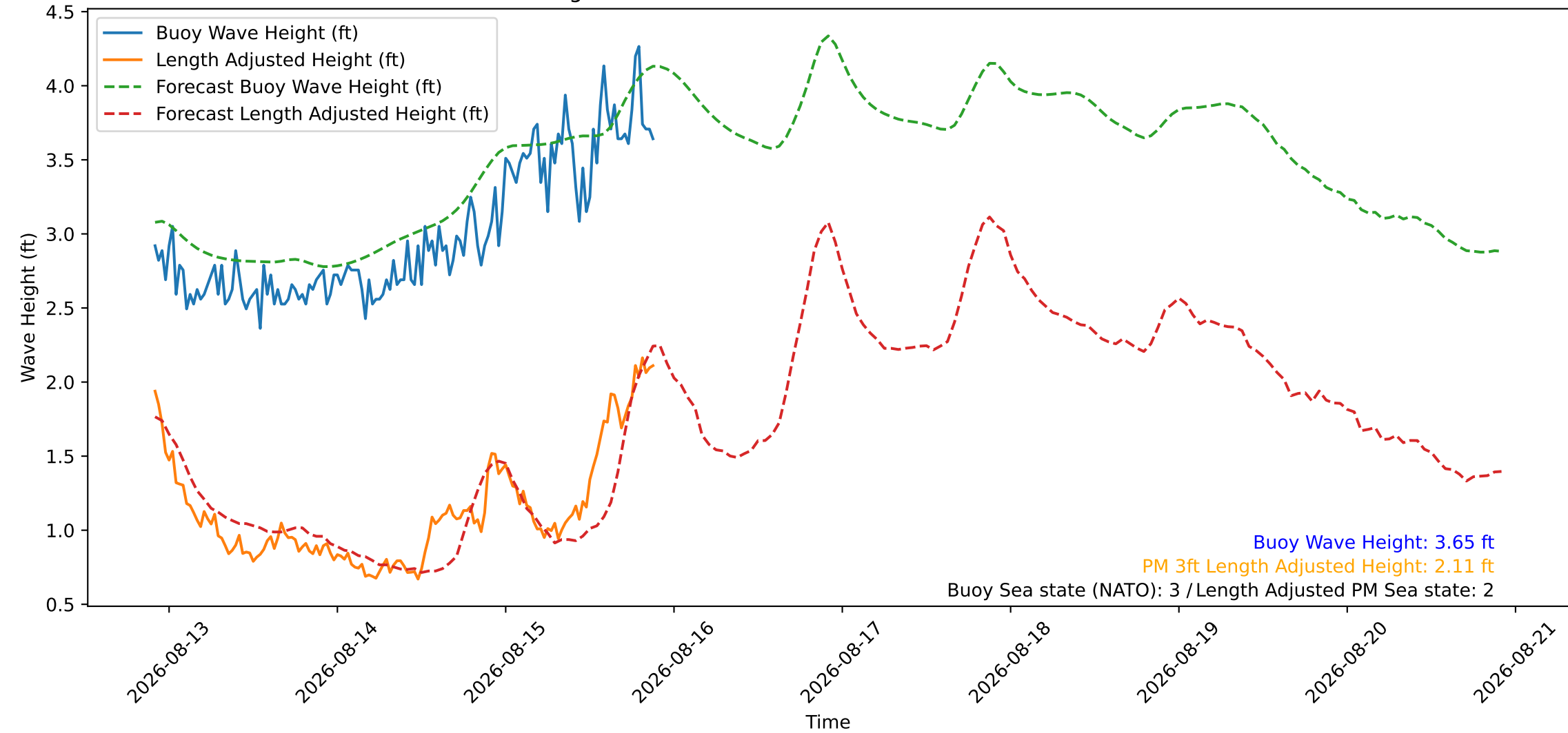
Wave Heights over Time for Green Beach at 2026-08-15 21:41:09
