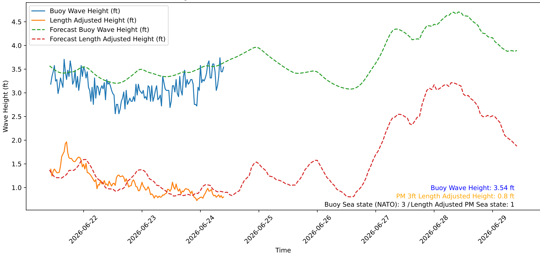
Wave Heights over Time for Oceanside Harbor at 2026-06-24 10:20:26
