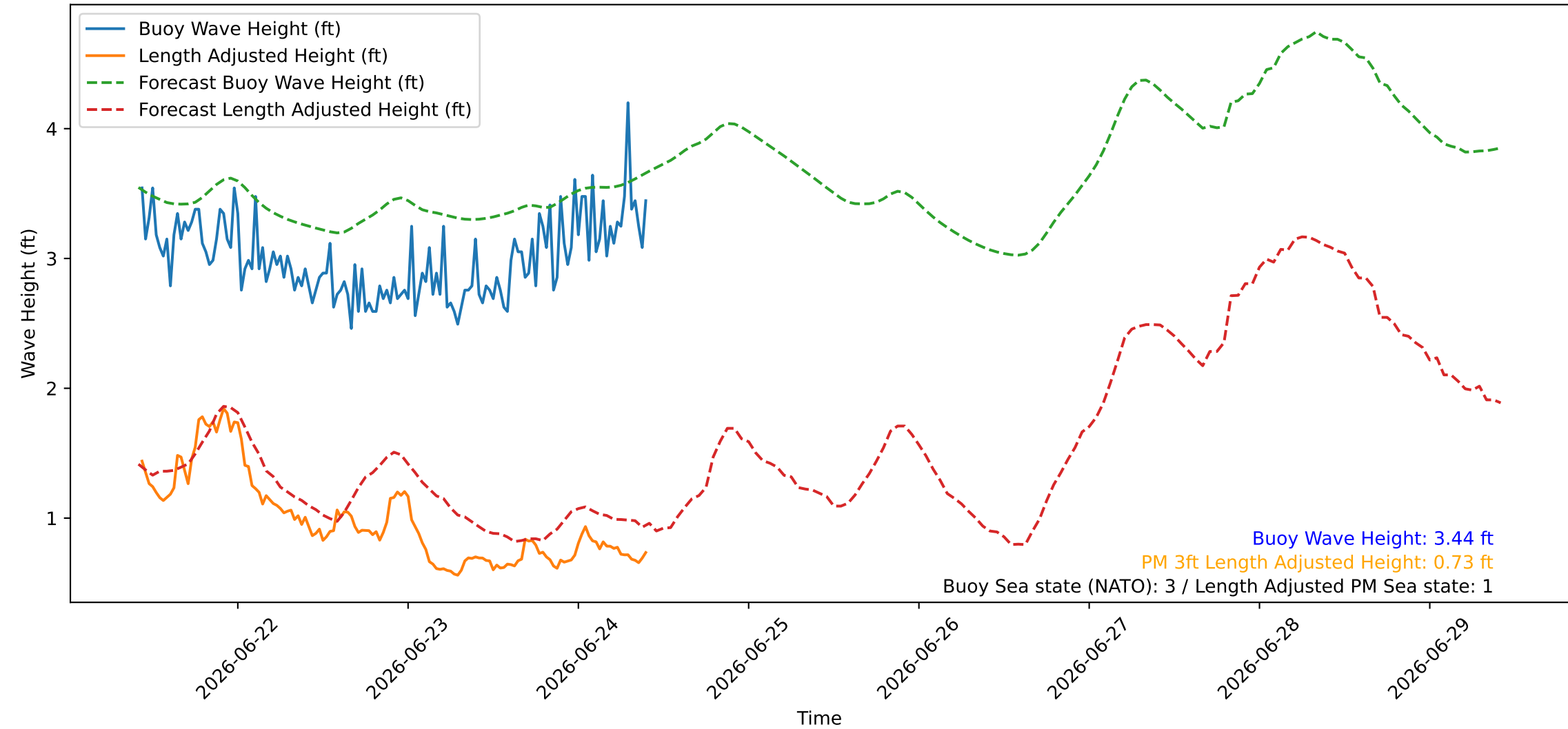
Wave Heights over Time for Green Beach at 2026-06-24 10:21:09
