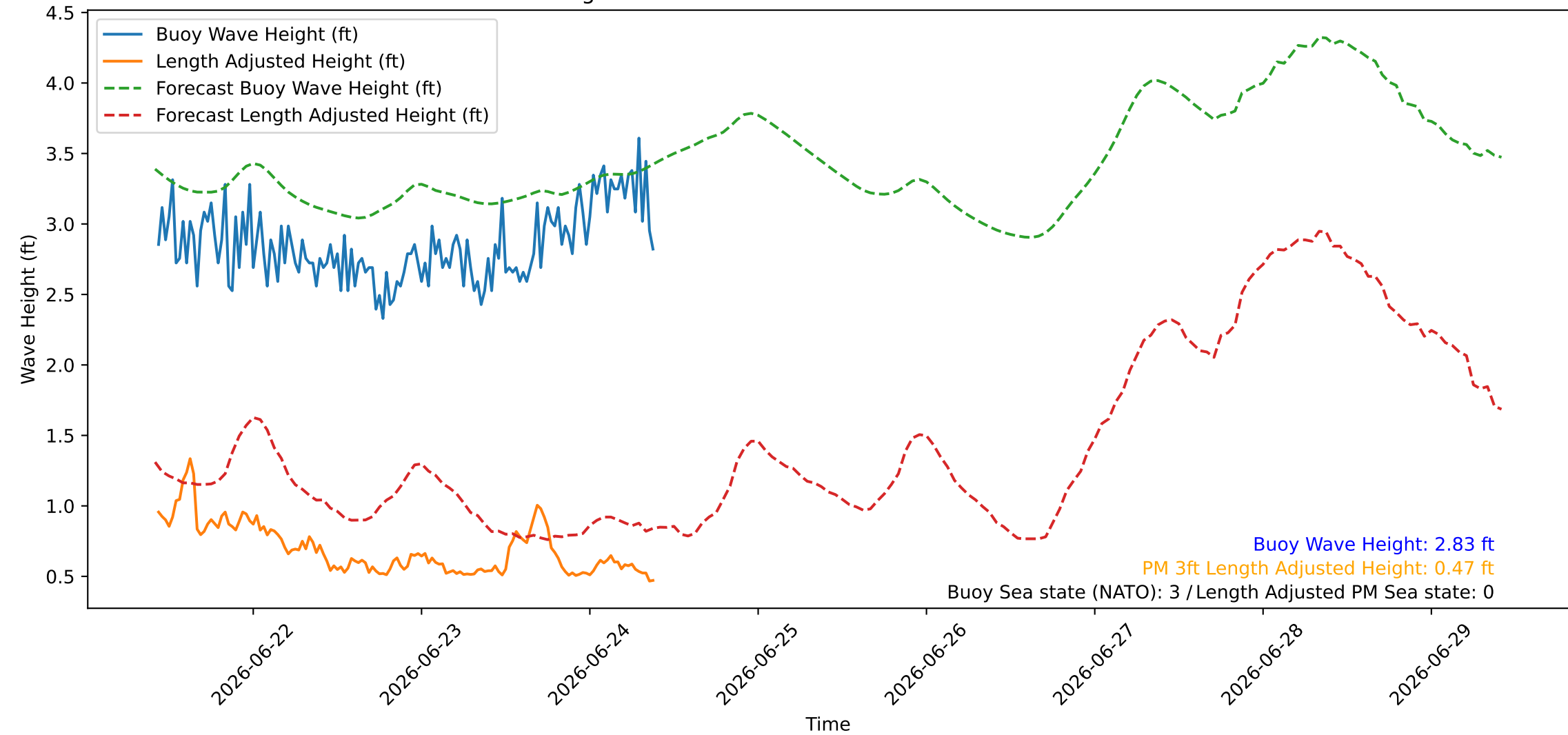
Wave Heights over Time for Red Beach at 2026-06-24 10:20:46
