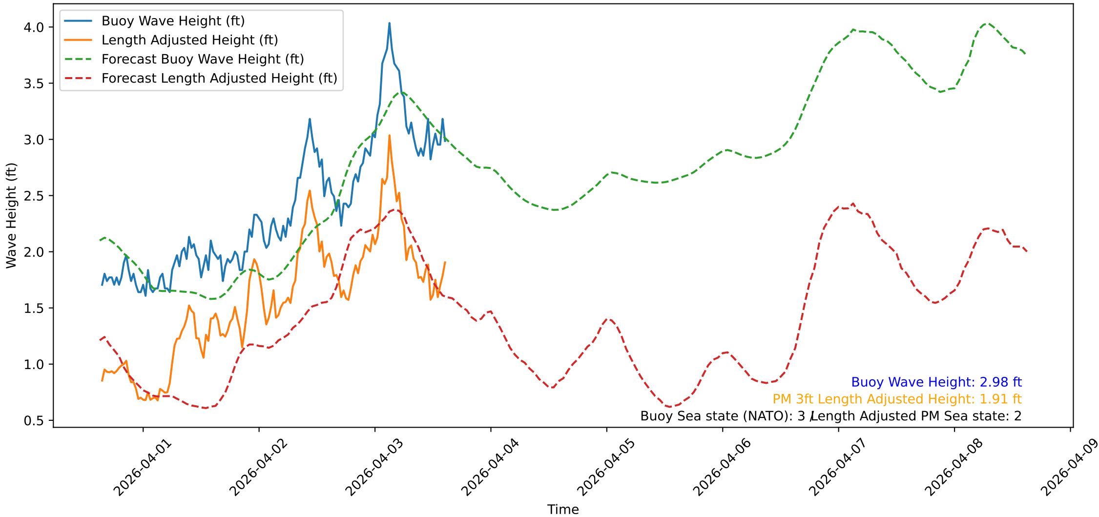
Wave Heights over Time for Oceanside Harbor at 2026-04-03 15:20:33
