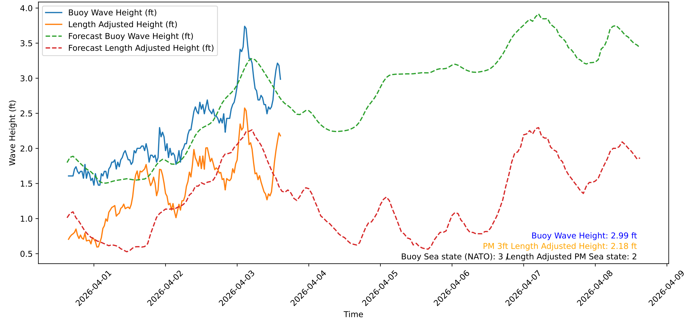
Wave Heights over Time for Red Beach at 2026-04-03 15:20:51
