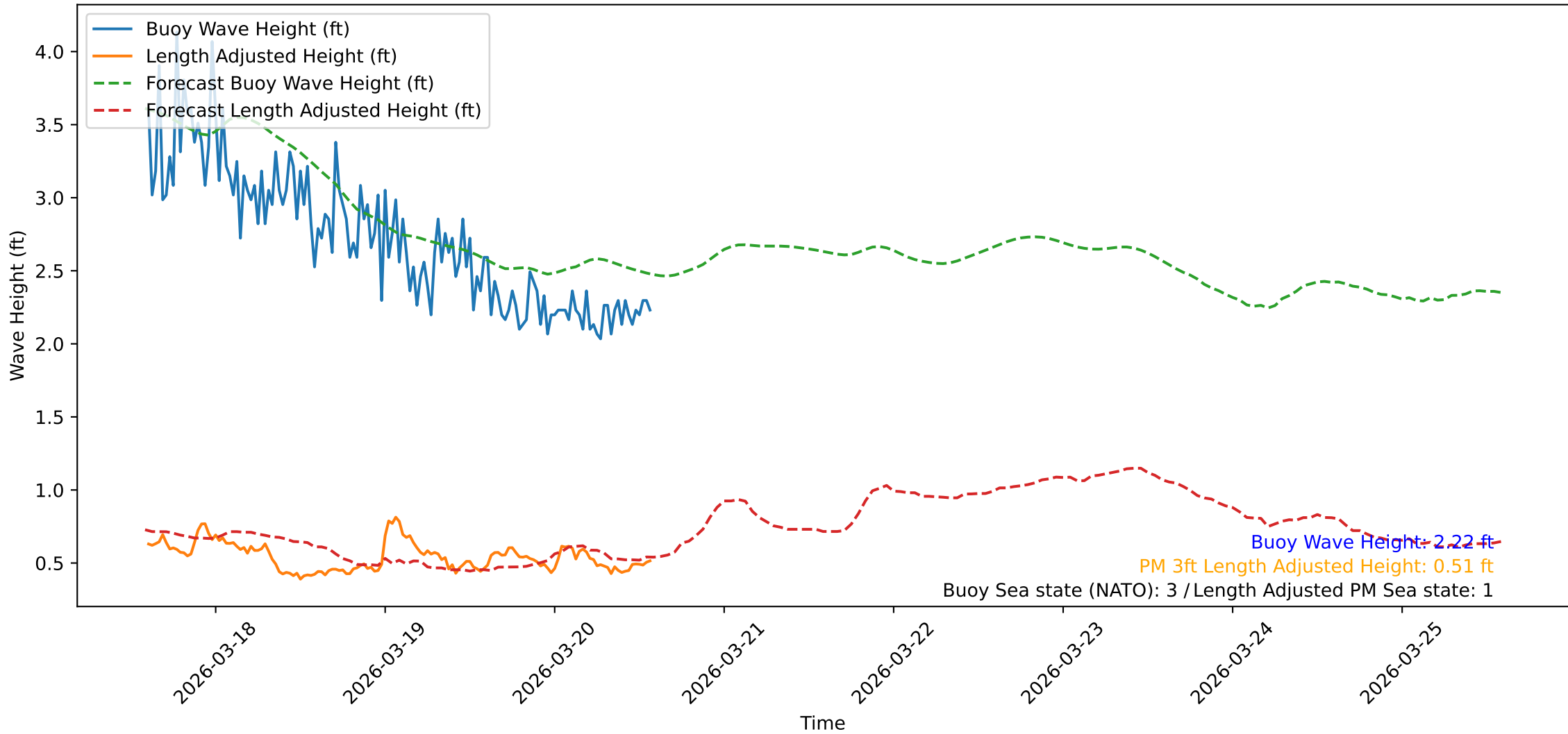
Wave Heights over Time for Green Beach at 2026-03-20 14:21:10
