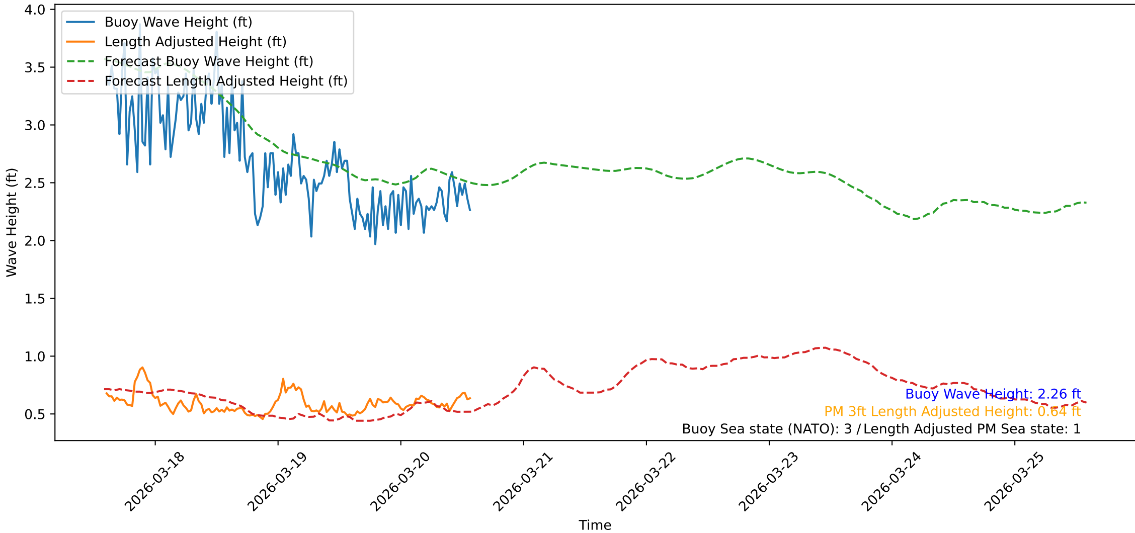
Wave Heights over Time for Oceanside Harbor at 2026-03-20 14:20:31
