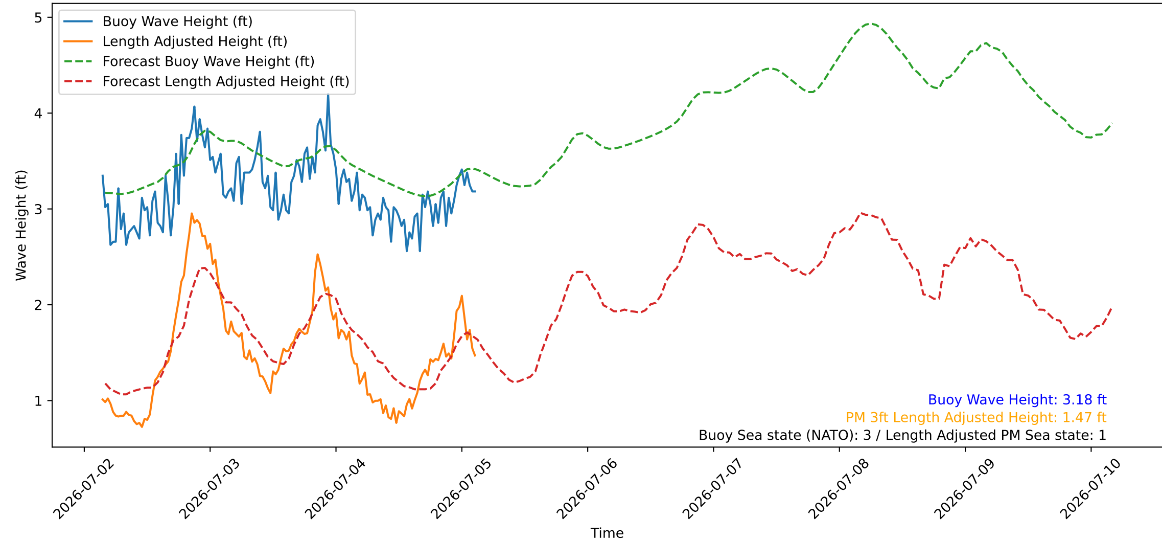
Wave Heights over Time for Green Beach at 2026-07-05 03:31:08
