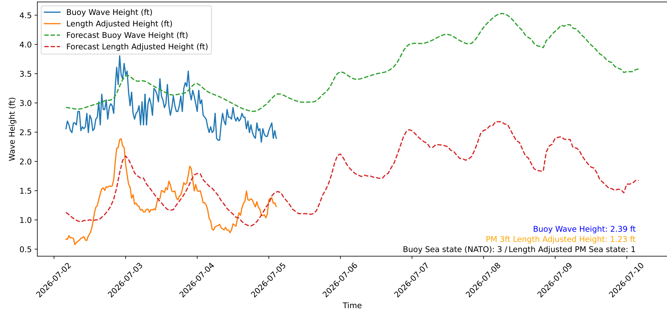
Wave Heights over Time for Red Beach at 2026-07-05 03:30:46
