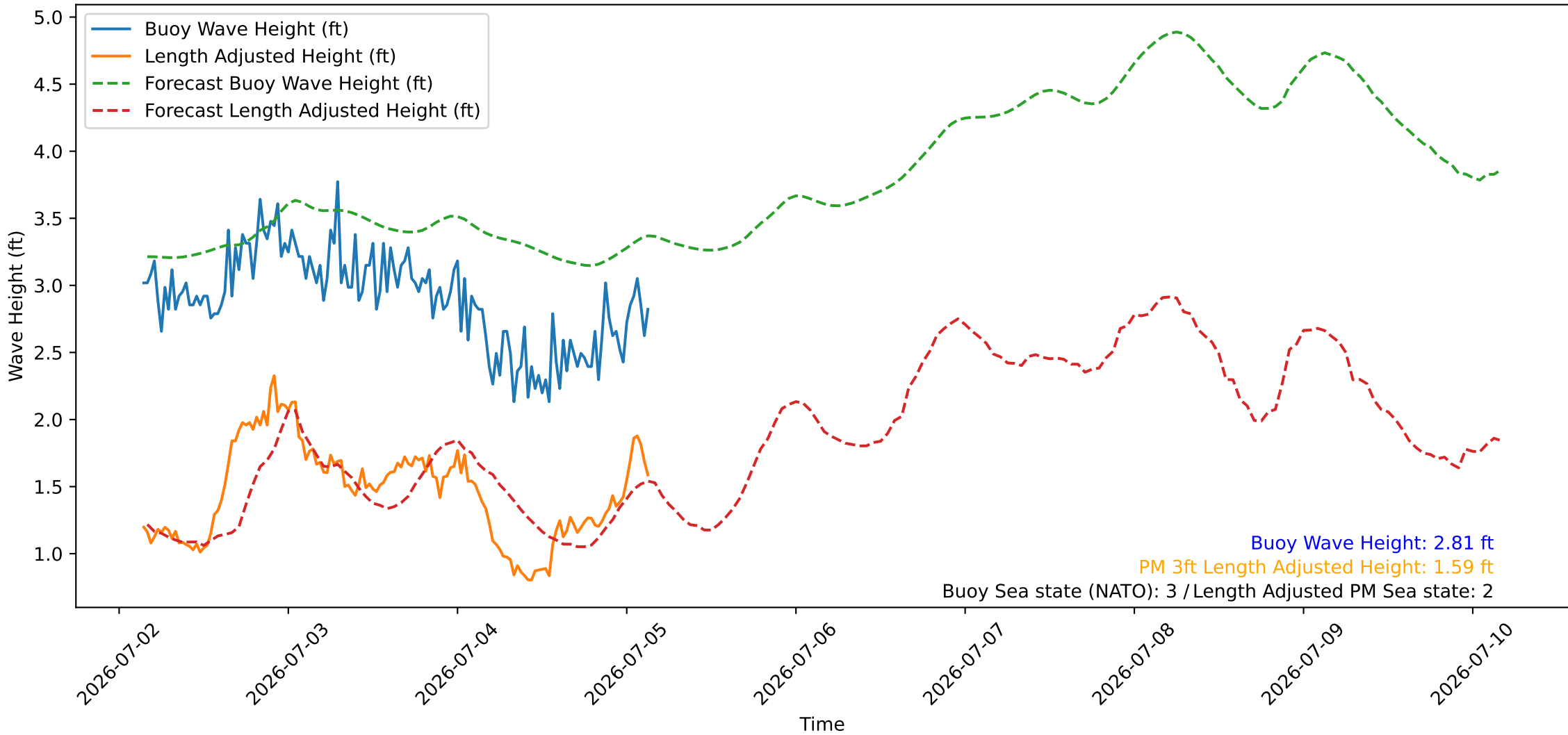
Wave Heights over Time for Oceanside Harbor at 2026-07-05 03:30:26
