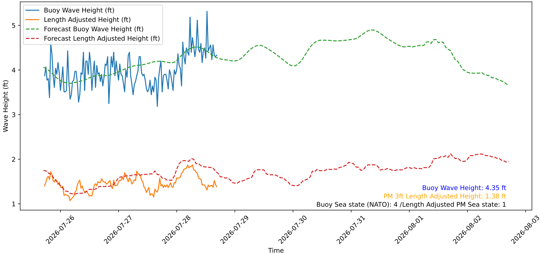
Wave Heights over Time for Oceanside Harbor at 2026-07-28 17:20:26
