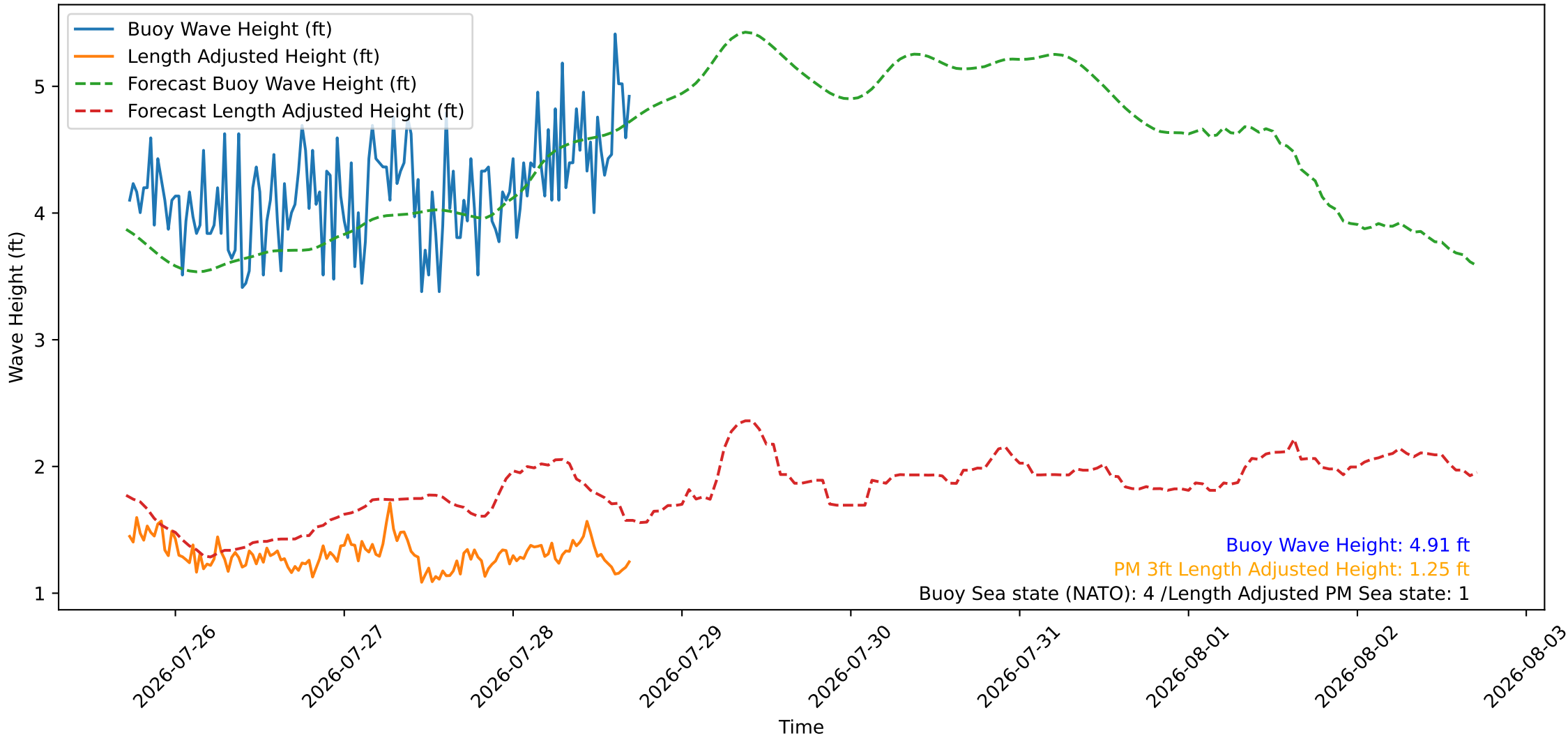
Wave Heights over Time for Green Beach at 2026-07-28 17:21:09
