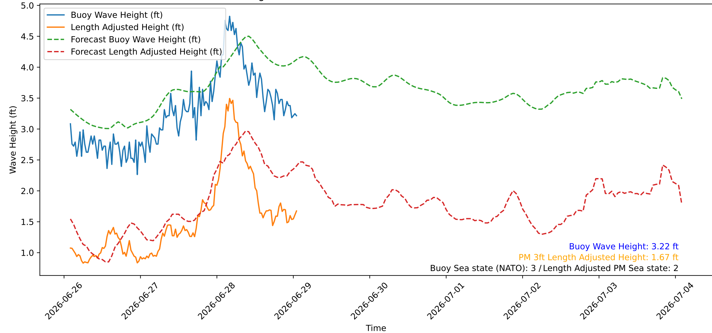
Wave Heights over Time for Green Beach at 2026-06-29 01:51:09
