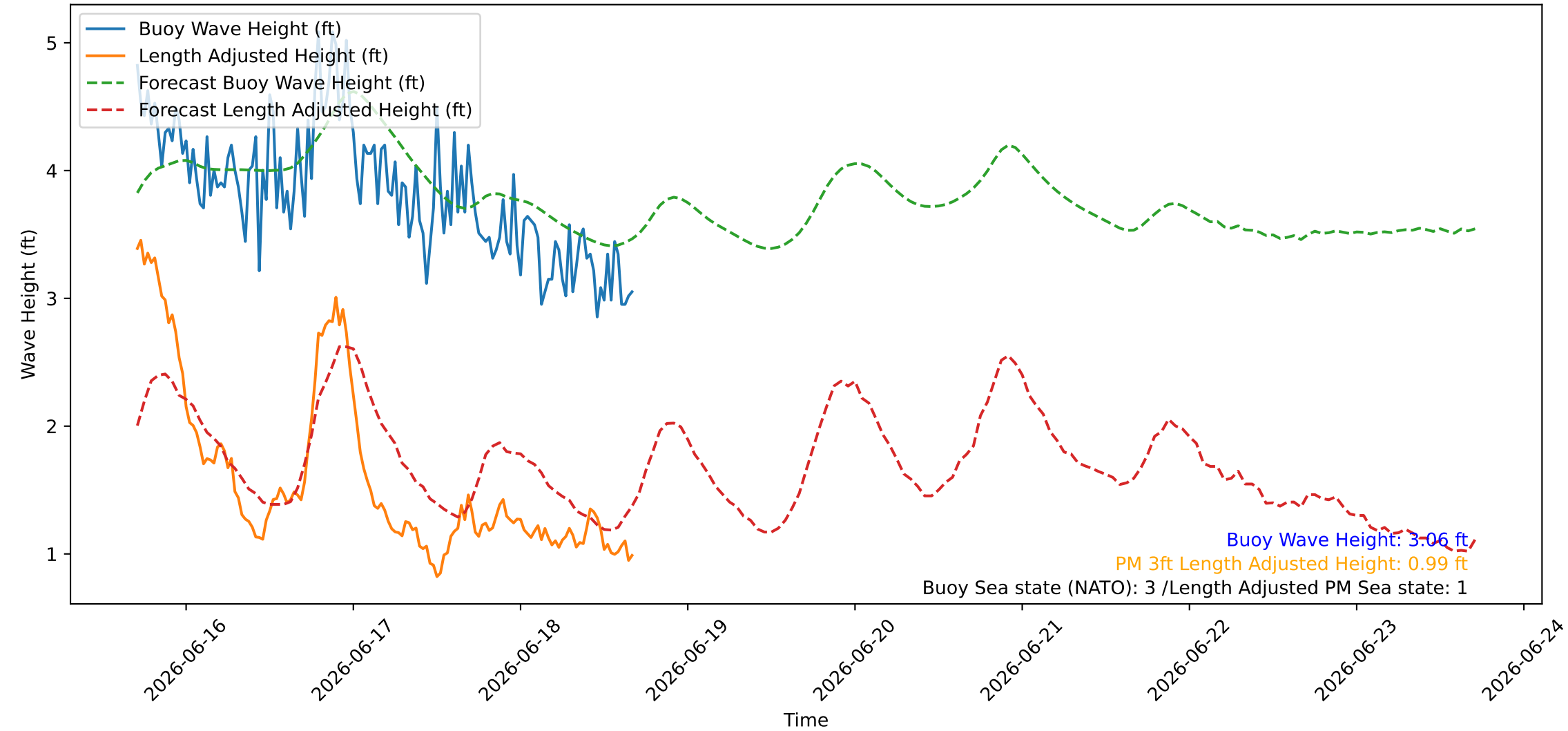
Wave Heights over Time for Green Beach at 2026-06-18 16:51:08
