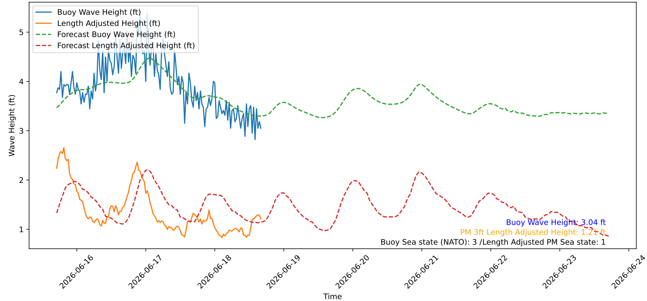
Wave Heights over Time for Red Beach at 2026-06-18 16:50:46
